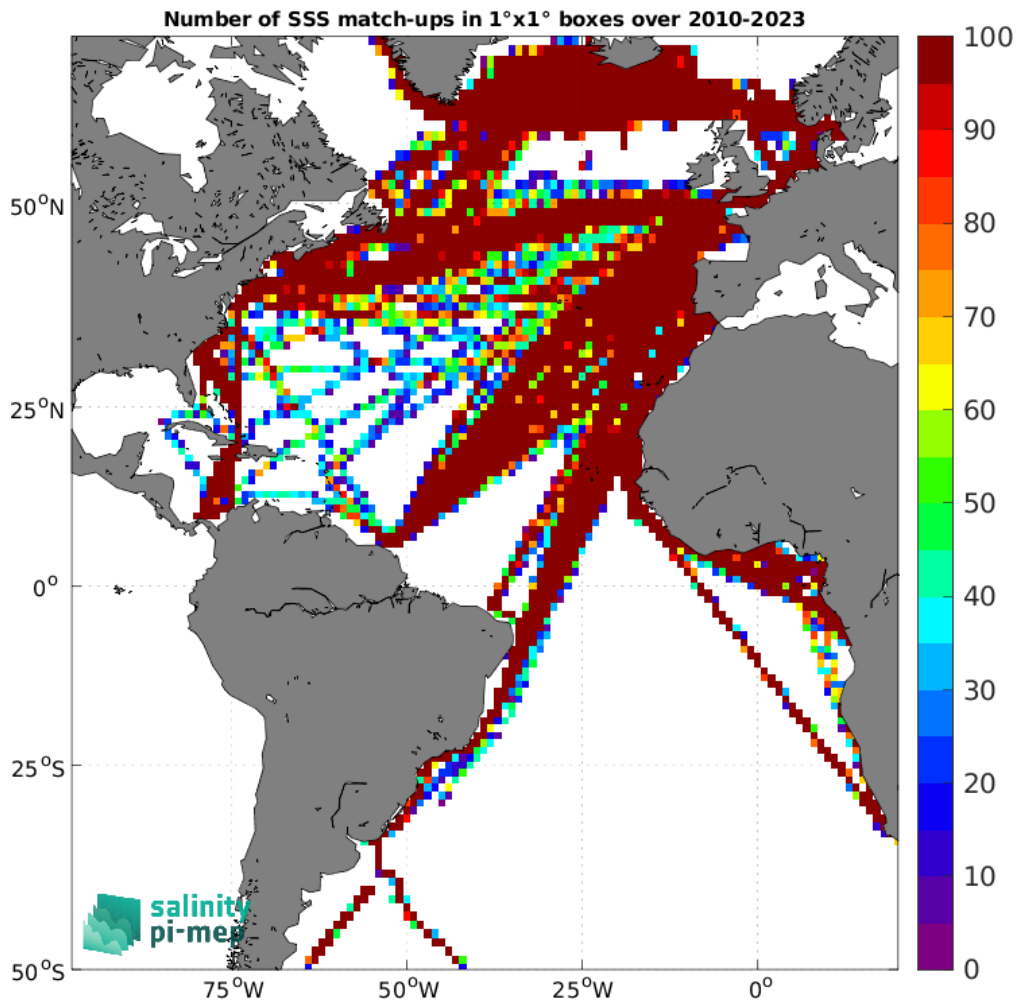
Figure 5: Number of SSS match-ups between TSG (LEGOS-DM) SSS and the SMOS SSS L4 OI v346 - Weekly (CMEMS-CATDS-LOPS) SSS product for the Atlantic Ocean Pi-MEP region over 1^\circ \times 1^\circ boxes and for the full satellite product period.
