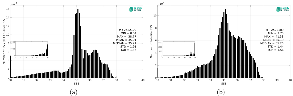
Figure 3: Histograms of SSS from TSG (LEGOS-DM) (a) and SMOS SSS L4 OI v346 - Weekly (CMEMS-CATDS-LOPS) (b) considering all match-up pairs per bins of 0.1 over the Atlantic Ocean Pi-MEP region and for the full satellite product period.
