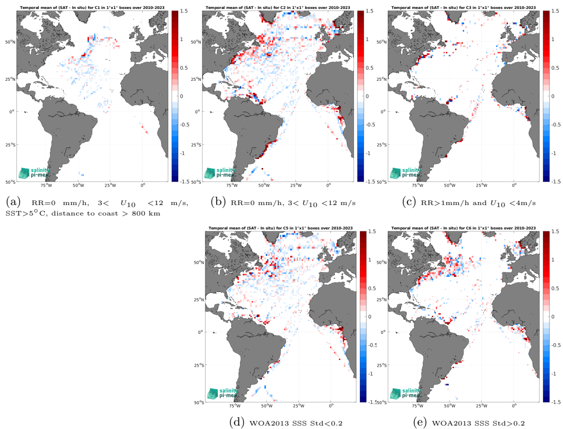
Figure 14: Temporal mean gridded over spatial boxes of size 1^\circ \times 1^\circ of \Delta\text{SSS} (SMOS SSS L4 OI v346 - Weekly (CMEMS-CATDS-LOPS) - TSG (LEGOS-DM)) for 5 different subdatasets corresponding to:RR=0 mm/h, 3 < U_{10} < 12 m/s, SST>5°C, distance to coast > 800 km (a), RR=0 mm/h, 3 < U_{10} < 12 m/s (b), RR>1mm/h and U_{10} < 4 m/s (c), WOA2013 SSS Std<0.2 (d), WOA2013 SSS Std>0.2 (e).
