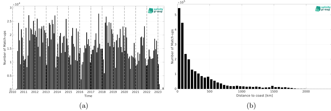
Figure 2: Number of match-ups between TSG (LEGOS-DM) and SMOS SSS L4 OI v346 - Weekly (CMEMS-CATDS-LOPS) SSS as a function of time (a) and as function of the distance to coast (b) over the Atlantic Ocean Pi-MEP region and for the full satellite product period.
