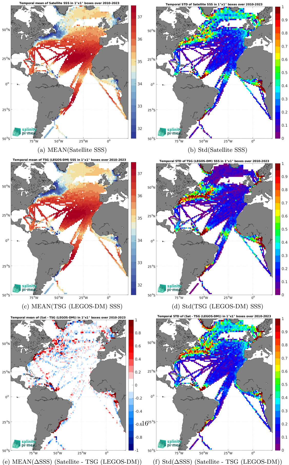
Figure 7: Temporal mean (left) and Std (right) of SSS from SMOS SSS L4 OI v346 - Weekly (CMEMS-CATDS-LOPS) (top), TSG (LEGOS-DM) (middle), and of \Delta SSS (Satellite - TSG (LEGOS-DM)). Only match-up pairs are used to generate these maps.
