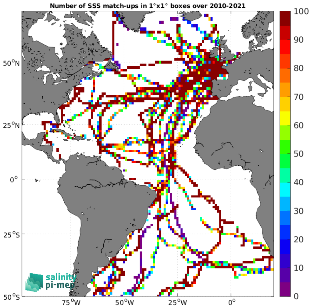
Figure 5: Number of SSS match-ups between TSG (GOSUD-Sailing-ship) SSS and the SMOS SSS L4 OI v346 - Weekly (CMEMS-CATDS-LOPS) SSS product for the Atlantic Ocean Pi-MEP region over 1^\circ \times 1^\circ boxes and for the full satellite product period.
