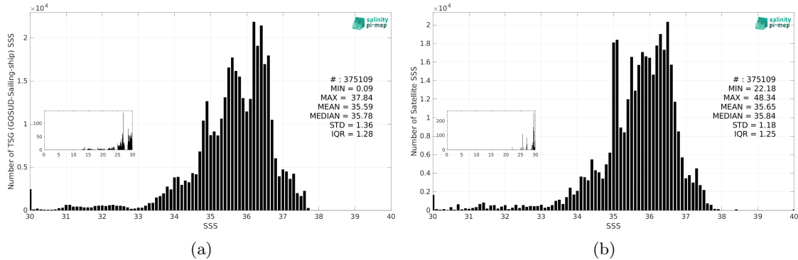
Figure 3: Histograms of SSS from TSG (GOSUD-Sailing-ship) (a) and SMOS SSS L4 OI v346 - Weekly (CMEMS-CATDS-LOPS) (b) considering all match-up pairs per bins of 0.1 over the Atlantic Ocean Pi-MEP region and for the full satellite product period.
