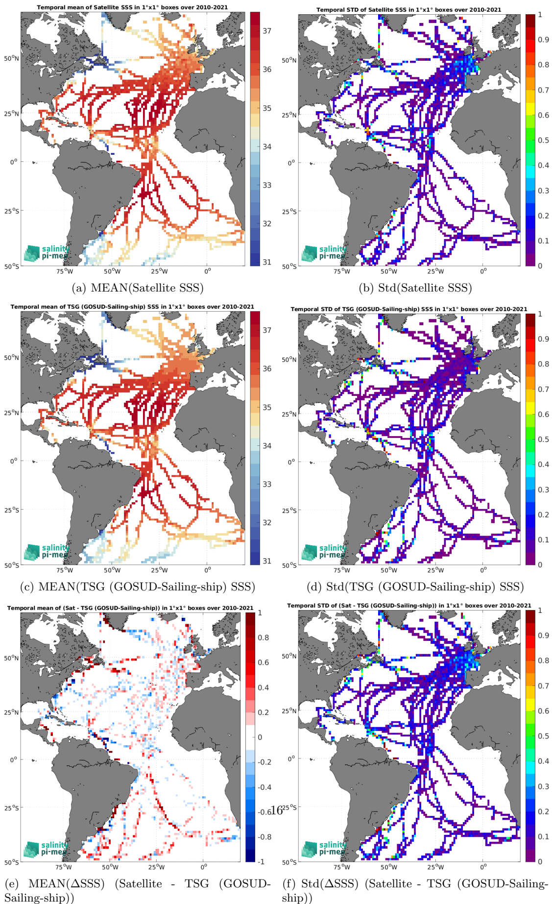
Figure 7: Temporal mean (left) and Std (right) of SSS from SMOS SSS L4 OI v346 - Weekly (CMEMS-CATDS-LOPS) (top), TSG (GOSUD-Sailing-ship) (middle), and of \Delta SSS (Satellite - TSG (GOSUD-Sailing-ship)). Only match-up pairs are used to generate these maps.
