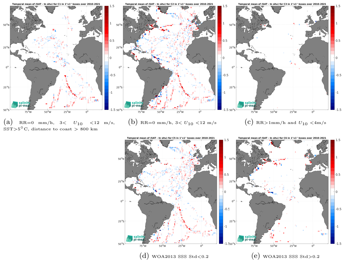
Figure 14: Temporal mean gridded over spatial boxes of size 1^\circ \times 1^\circ of \Delta\text{SSS} (SMOS SSS L4 OI v346 - Weekly (CMEMS-CATDS-LOPS) - TSG (GOSUD-Sailing-ship)) for 5 different sub-datasets corresponding to:RR=0 mm/h, 3 < U_{10} < 12 m/s, SST>5°C, distance to coast > 800 km (a), RR=0 mm/h, 3 < U_{10} < 12 m/s (b), RR>1mm/h and U_{10} < 4 m/s (c), WOA2013 SSS Std<0.2 (d), WOA2013 SSS Std>0.2 (e).
