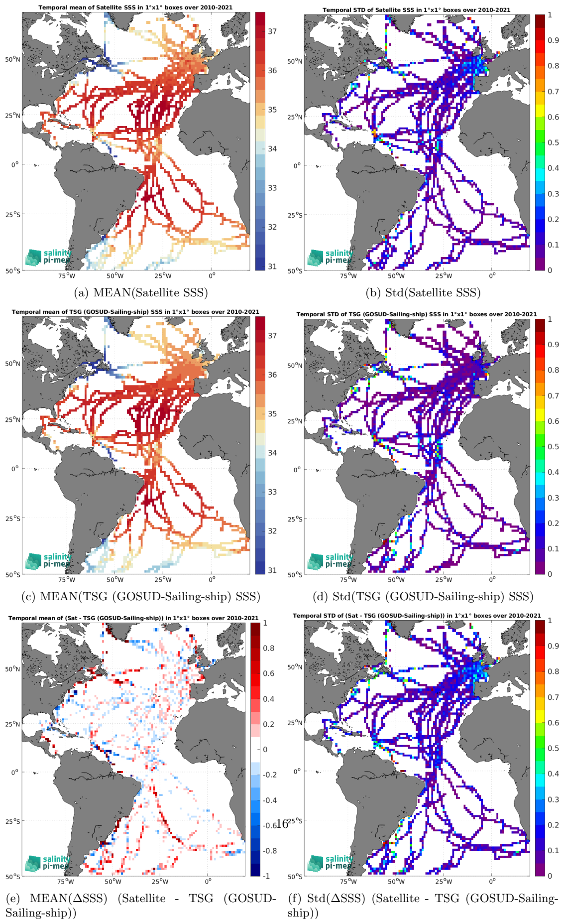
Figure 7: Temporal mean (left) and Std (right) of SSS from SMOS SSS L4 OI v346 - Weekly (CMEMS-CATDS-LOPS) (top), TSG (GOSUD-Sailing-ship) (middle), and of \Delta\text{SSS} (Satellite - TSG (GOSUD-Sailing-ship)). Only match-up pairs are used to generate these maps.
