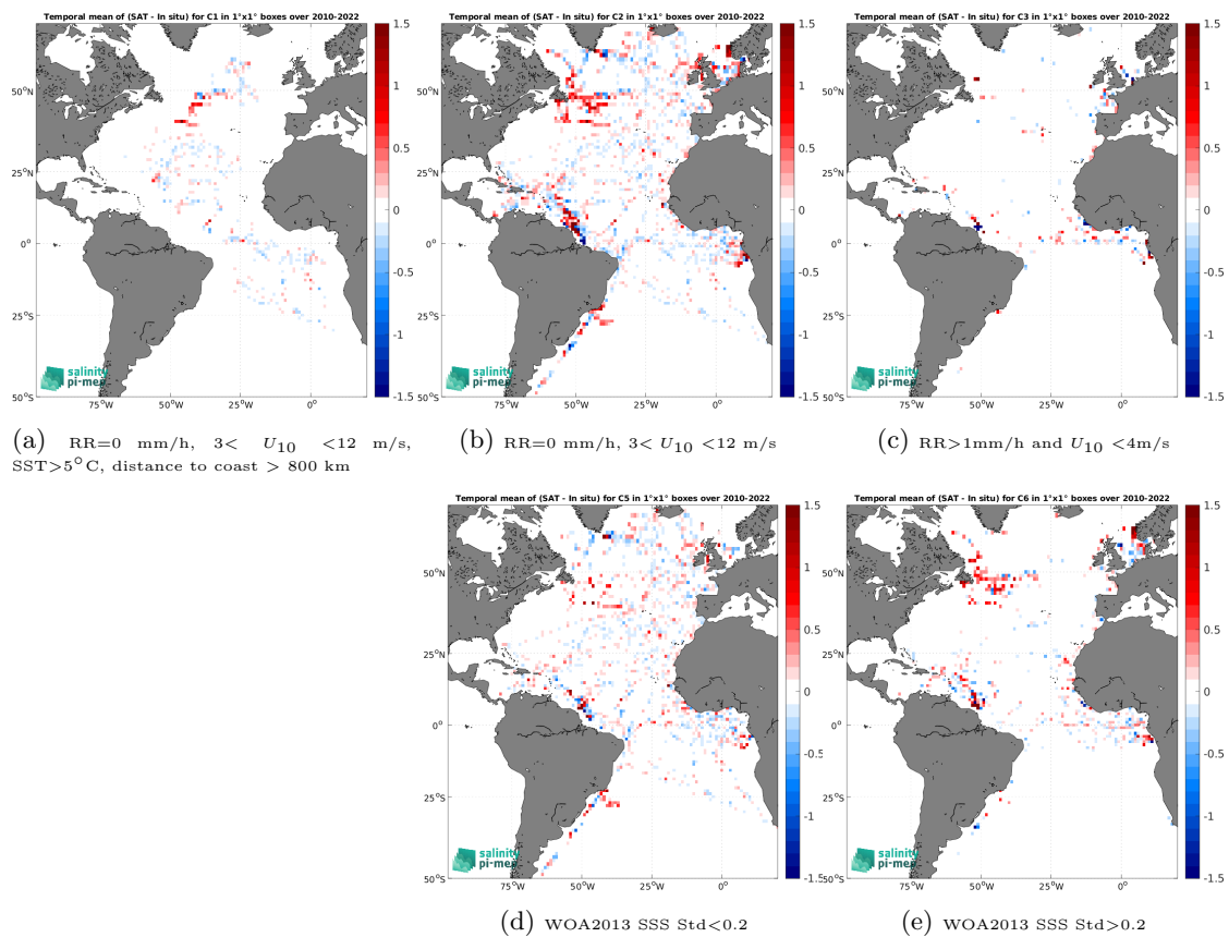
Figure 14: Temporal mean gridded over spatial boxes of size 1^\circ \times 1^\circ of \Delta SSS (SMOS SSS L4 OI v346 - Weekly (CMEMS-CATDS-LOPS) - TSG (GOSUD-Research-vessel)) for 5 different subdatasets corresponding to:RR=0 mm/h, 3 < U_{10} < 12 m/s, SST >5^\circ\text{C} , distance to coast > 800 km (a), RR=0 mm/h, 3 < U_{10} < 12 m/s (b), RR >1 mm/h and U_{10} < 4 m/s (c), WOA2013 SSS Std <0.2 (d), WOA2013 SSS Std >0.2 (e).
