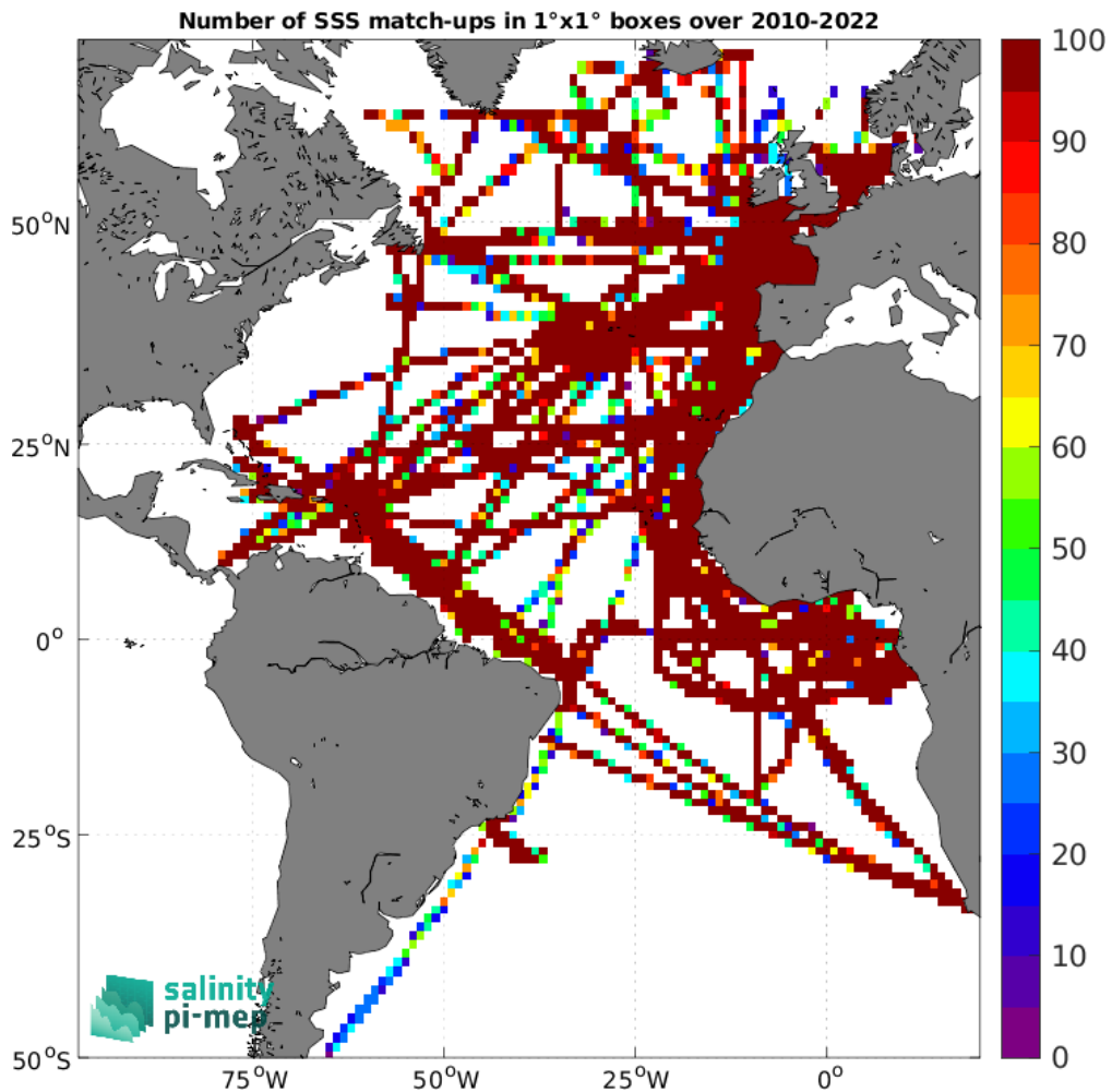
Figure 5: Number of SSS match-ups between TSG (GOSUD-Research-vessel) SSS and the SMOS SSS L4 OI v346 - Weekly (CMEMS-CATDS-LOPS) SSS product for the Atlantic Ocean Pi-MEP region over 1°x1° boxes and for the full satellite product period.
