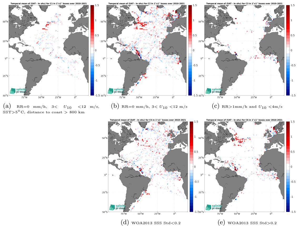
Figure 14: Temporal mean gridded over spatial boxes of size 1^\circ \times 1^\circ of \Delta\text{SSS} (SMOS SSS L4 OI v346 - Weekly (CMEMS-CATDS-LOPS) - TSG (GOSUD-Research-vessel)) for 5 different subdatasets corresponding to:RR=0 mm/h, 3 < U_{10} < 12 m/s, SST >5^\circ\text{C} , distance to coast > 800 km (a), RR=0 mm/h, 3 < U_{10} < 12 m/s (b), RR >1 mm/h and U_{10} < 4 m/s (c), WOA2013 SSS Std <0.2 (d), WOA2013 SSS Std >0.2 (e).
