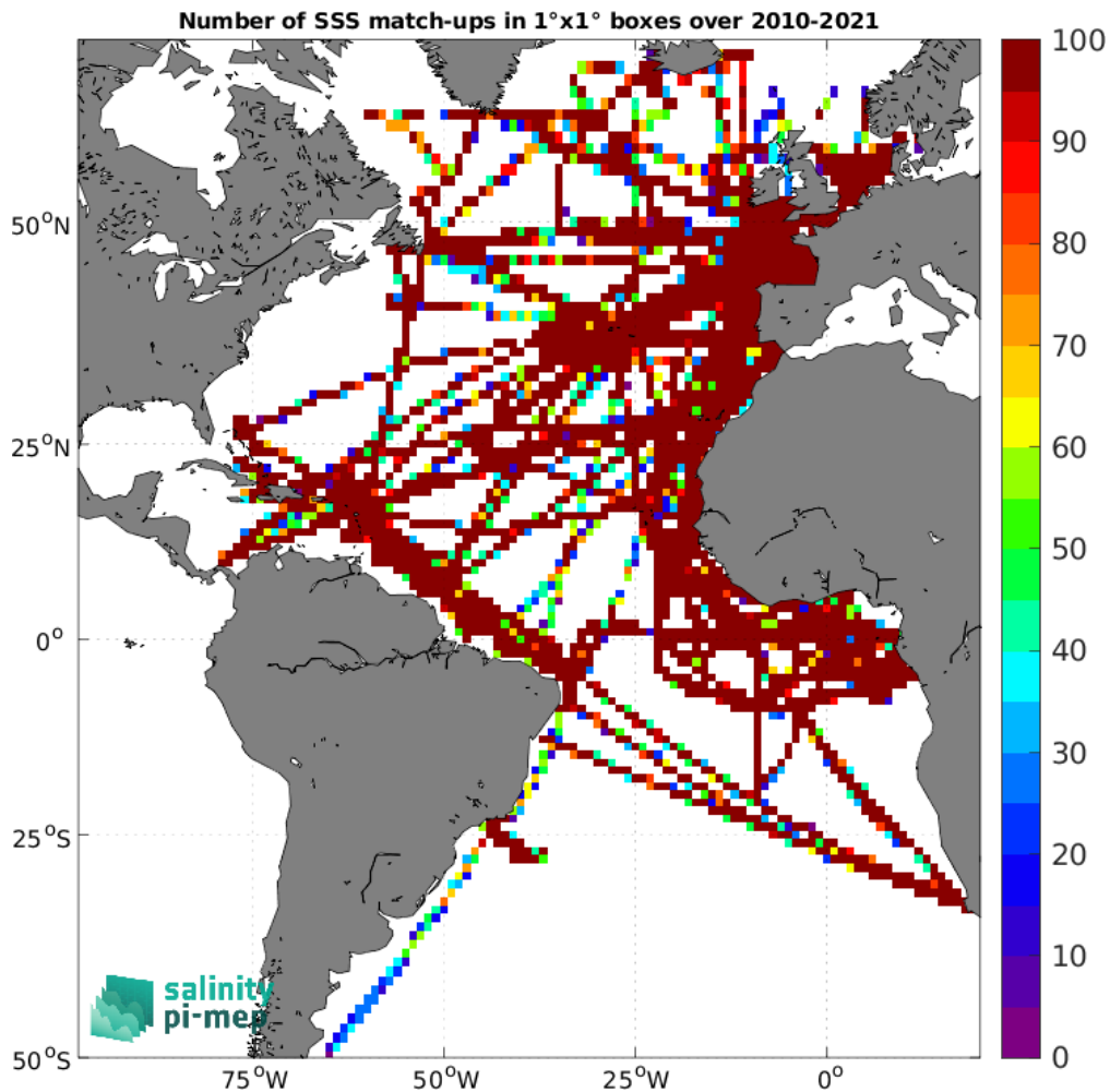
Figure 5: Number of SSS match-ups between TSG (GOSUD-Research-vessel) SSS and the SMOS SSS L4 OI v346 - Weekly (CMEMS-CATDS-LOPS) SSS product for the Atlantic Ocean Pi-MEP region over 1^\circ \times 1^\circ boxes and for the full satellite product period.
