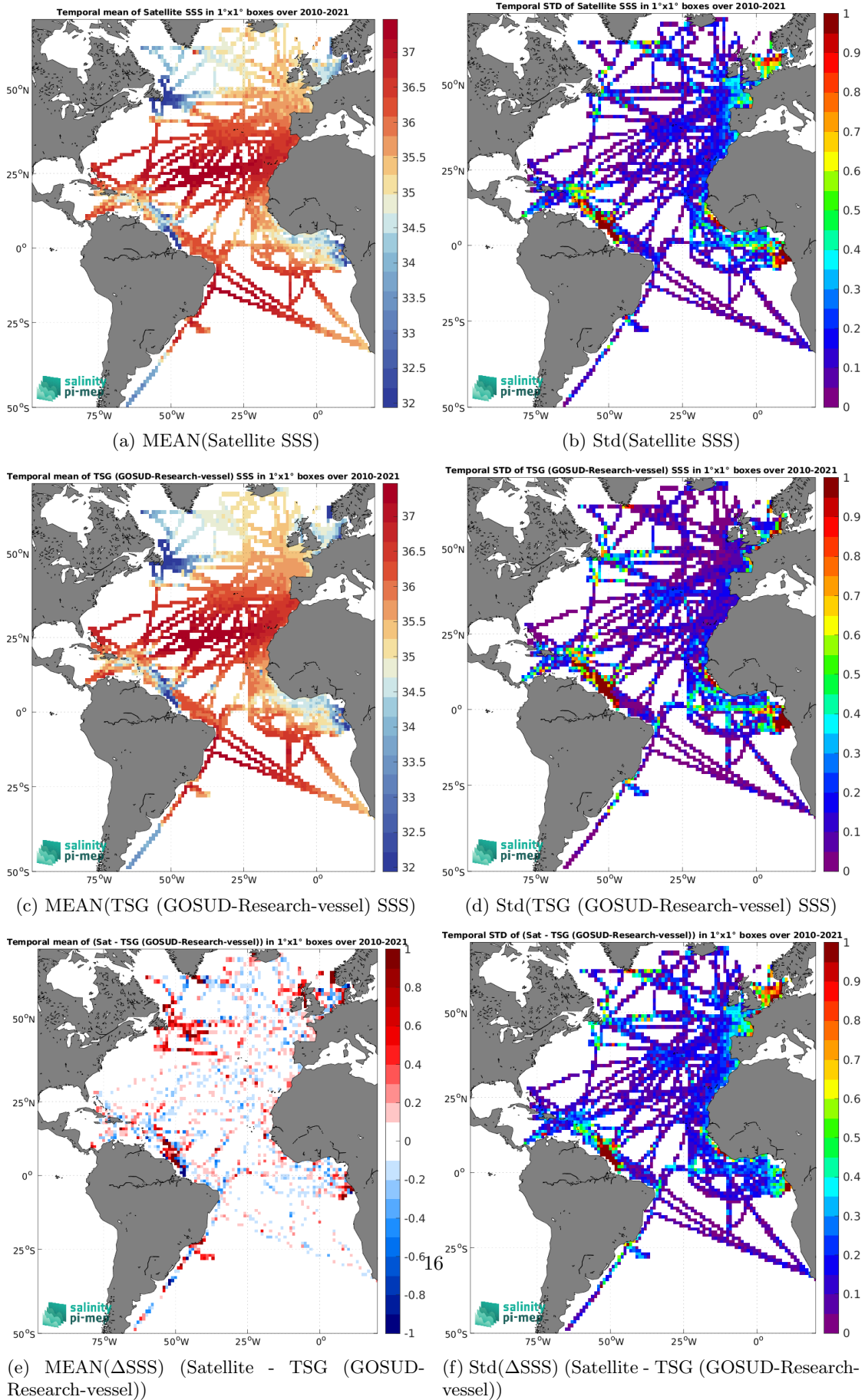
Figure 7: Temporal mean (left) and Std (right) of SSS from SMOS SSS L4 OI v346 - Weekly (CMEMS-CATDS-LOPS) (top), TSG (GOSUD-Research-vessel) (middle), and of \Delta SSS (Satellite - TSG (GOSUD-Research-vessel)). Only match-up pairs are used to generate these maps.
