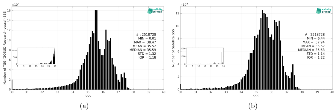
Figure 3: Histograms of SSS from TSG (GOSUD-Research-vessel) (a) and SMOS SSS L4 OI v346 - Weekly (CMEMS-CATDS-LOPS) (b) considering all match-up pairs per bins of 0.1 over the Atlantic Ocean Pi-MEP region and for the full satellite product period.
