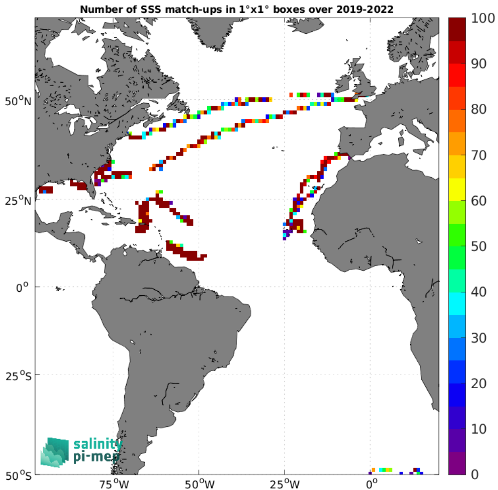
Figure 5: Number of SSS match-ups between Saildrone SSS and the SMOS SSS L4 OI v346 - Weekly (CMEMS-CATDS-LOPS) SSS product for the Atlantic Ocean Pi-MEP region over 1°×1° boxes and for the full satellite product period.
