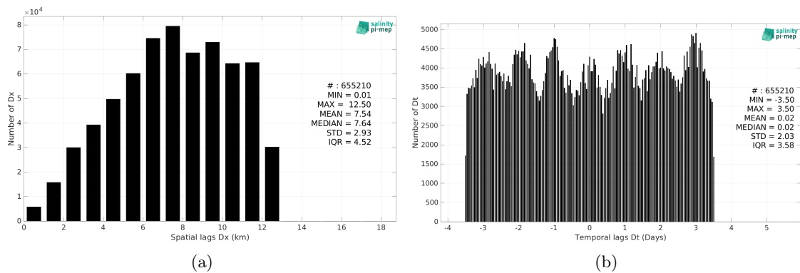
Figure 6: Histograms of the spatial (a) and temporal (b) lags between the location/time of the ICES measurement and the date of the corresponding SMOS SSS L4 OI v346 - Weekly (CMEMS-CATDS-LOPS) SSS pixel.
