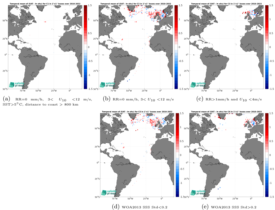
Figure 14: Temporal mean gridded over spatial boxes of size 1^\circ \times 1^\circ of \Delta\text{SSS} (SMOS SSS L4 OI v346 - Weekly (CMEMS-CATDS-LOPS) - ICES) for 5 different subdatasets corresponding to:RR=0 mm/h, 3 < U_{10} < 12 m/s, SST>5°C, distance to coast > 800 km (a), RR=0 mm/h, 3 < U_{10} < 12 m/s (b), RR>1mm/h and U_{10} < 4 m/s (c), WOA2013 SSS Std<0.2 (d), WOA2013 SSS Std>0.2 (e).
