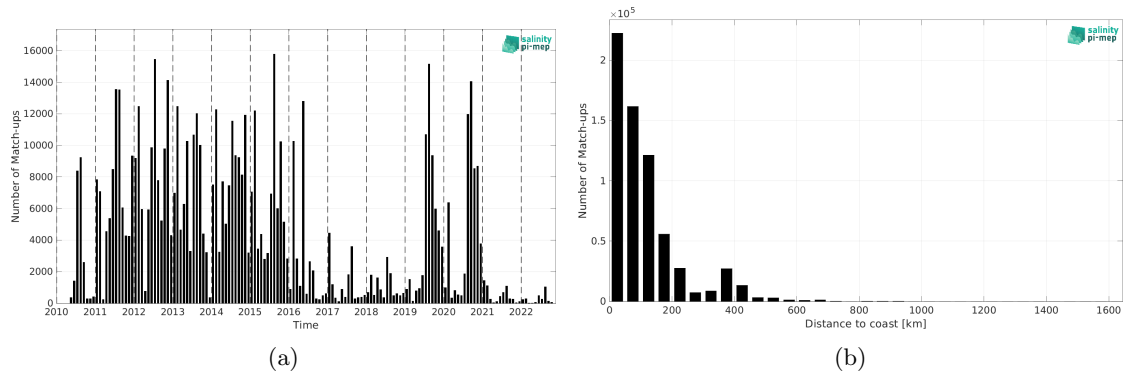
Figure 2: Number of match-ups between ICES and SMOS SSS L4 OI v346 - Weekly (CMEMS-CATDS-LOPS) SSS as a function of time (a) and as function of the distance to coast (b) over the Atlantic Ocean Pi-MEP region and for the full satellite product period.
