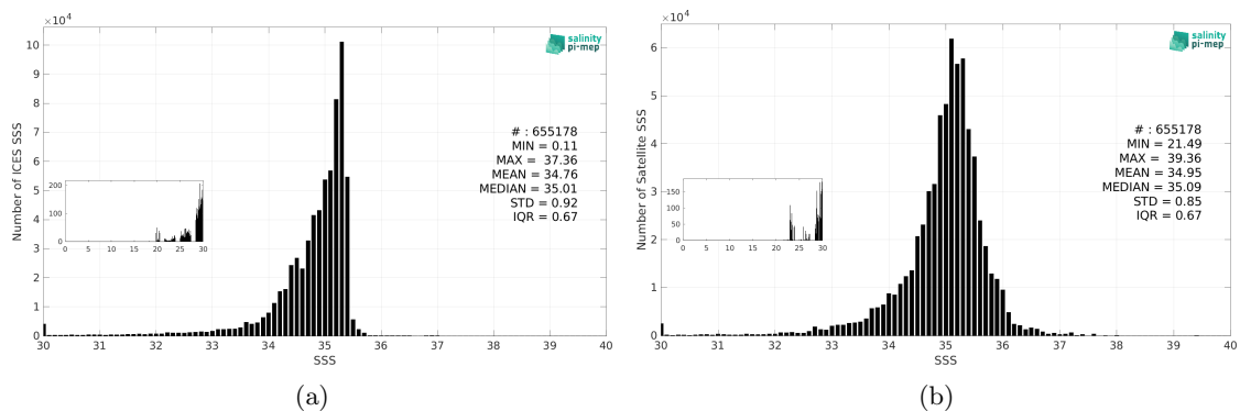
Figure 3: Histograms of SSS from ICES (a) and SMOS SSS L4 OI v346 - Weekly (CMEMS-CATDS-LOPS) (b) considering all match-up pairs per bins of 0.1 over the Atlantic Ocean Pi-MEP region and for the full satellite product period.
