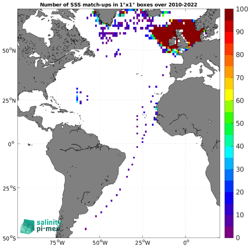
Figure 5: Number of SSS match-ups between ICES SSS and the SMOS SSS L4 OI v346 - Weekly (CMEMS-CATDS-LOPS) SSS product for the Atlantic Ocean Pi-MEP region over 1^\circ \times 1^\circ boxes and for the full satellite product period.
