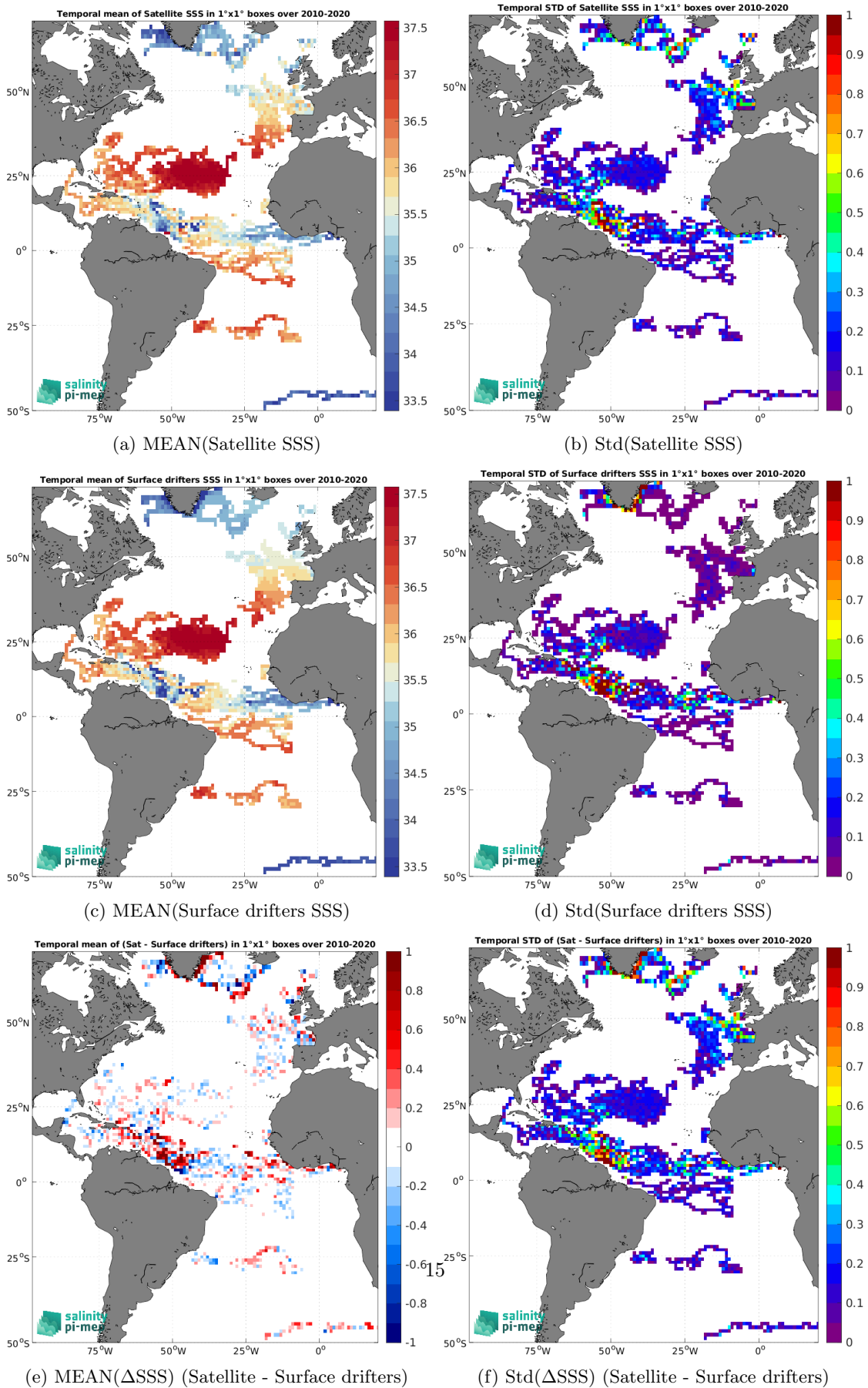
Figure 6: Temporal mean (left) and Std (right) of SSS from SMOS SSS L4 OI v346 - Weekly (CMEMS-CATDS-LOPS) (top), Surface drifters (middle), and of \Delta SSS (Satellite - Surface drifters). Only match-up pairs are used to generate these maps.
