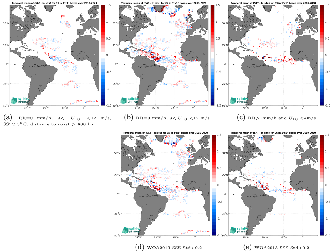
Figure 13: Temporal mean gridded over spatial boxes of size 1^\circ \times 1^\circ of \Delta SSS (SMOS SSS L4 OI v346 - Weekly (CMEMS-CATDS-LOPS) - Surface drifters) for 5 different subdatasets corresponding to:RR=0 mm/h, 3 < U_{10} < 12 m/s, SST >5^\circ\text{C} , distance to coast > 800 km (a), RR=0 mm/h, 3 < U_{10} < 12 m/s (b), RR >1 mm/h and U_{10} < 4 m/s (c), WOA2013 SSS Std <0.2 (d), WOA2013 SSS Std >0.2 (e).
