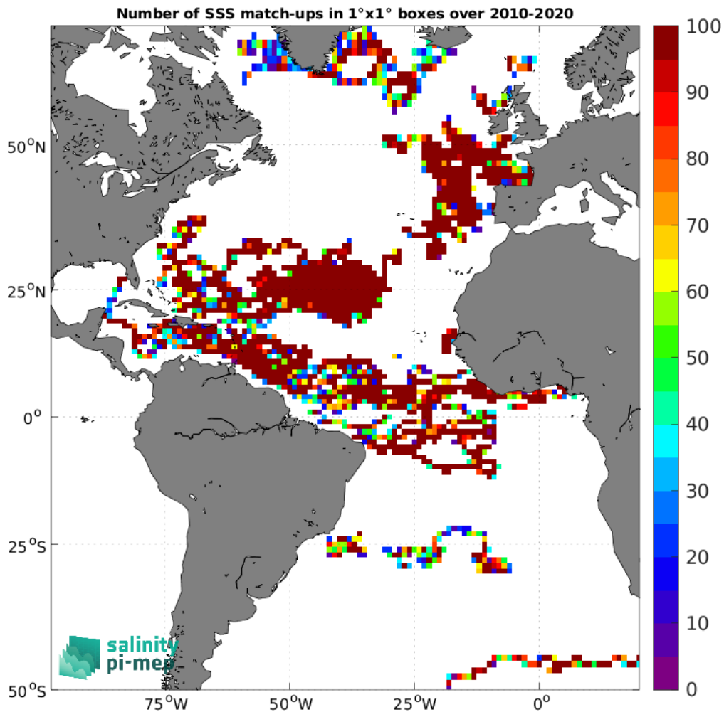
Figure 4: Number of SSS match-ups between Surface drifters SSS and the SMOS SSS L4 OI v346 - Weekly (CMEMS-CATDS-LOPS) SSS product for the Atlantic Ocean Pi-MEP region over 1°x1° boxes and for the full satellite product period.
