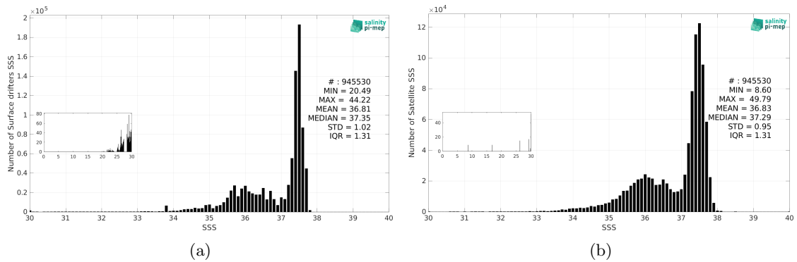
Figure 3: Histograms of SSS from Surface drifters (a) and SMOS SSS L4 OI v346 - Weekly (CMEMS-CATDS-LOPS) (b) considering all match-up pairs per bins of 0.1 over the Atlantic Ocean Pi-MEP region and for the full satellite product period.
