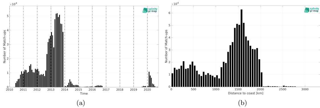
Figure 2: Number of match-ups between Surface drifters and SMOS SSS L4 OI v346 - Weekly (CMEMS-CATDS-LOPS) SSS as a function of time (a) and as function of the distance to coast (b) over the Atlantic Ocean Pi-MEP region and for the full satellite product period.
