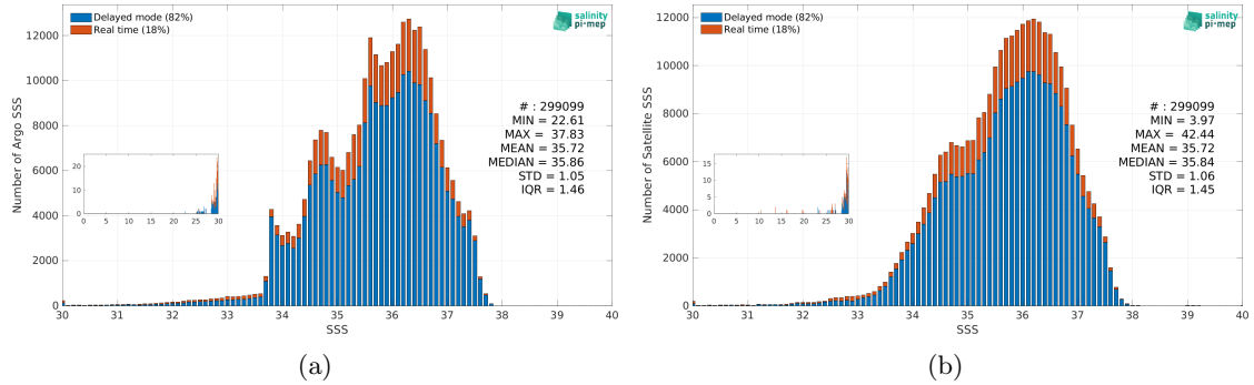
Figure 3: Histograms of SSS from Argo (a) and SMOS SSS L4 OI v346 - Weekly (CMEMS-CATDS-LOPS) (b) considering all match-up pairs per bins of 0.1 over the Atlantic Ocean Pi-MEP region and for the full satellite product period.
