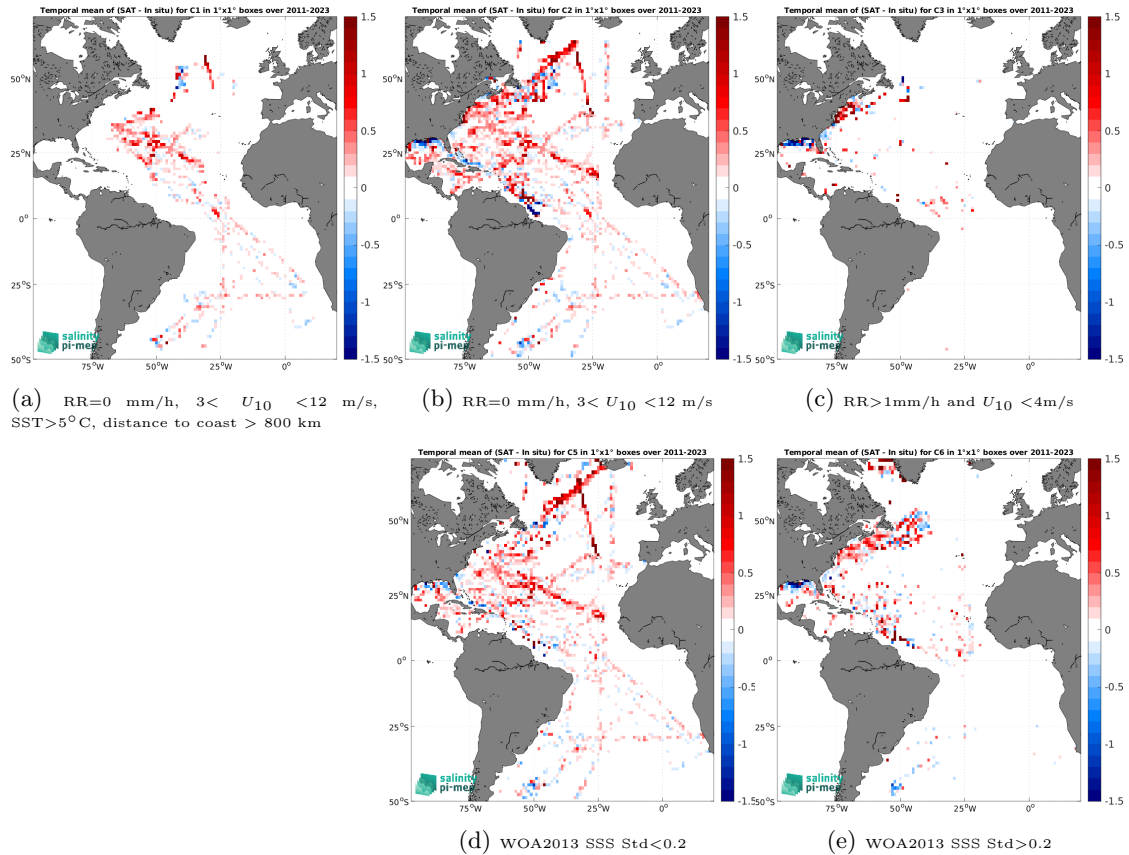
Figure 12: Temporal mean gridded over spatial boxes of size 1^\circ \times 1^\circ of \Delta\text{SSS} (SMOS SSS L4 OI v342 - Weekly (CMEMS-CATDS-LOPS) - TSG (SAMOS)) for 5 different subdatasets corresponding to:RR=0 mm/h, 3 < U_{10} < 12 m/s, SST >5^\circ\text{C} , distance to coast > 800 km (a), RR=0 mm/h, 3 < U_{10} < 12 m/s (b), RR >1 mm/h and U_{10} < 4 m/s (c), WOA2013 SSS Std <0.2 (d), WOA2013 SSS Std >0.2 (e).
