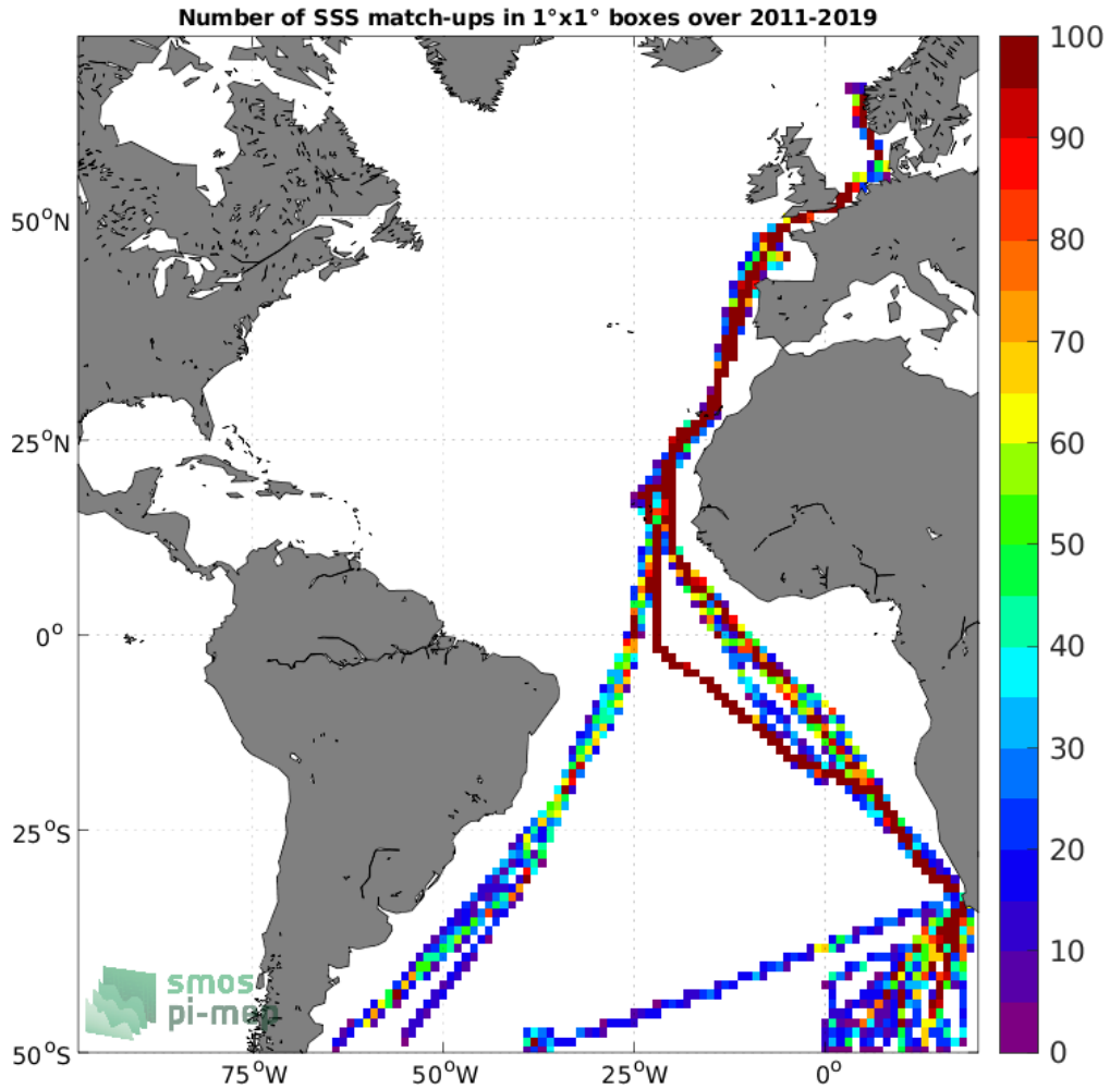
Figure 4: Number of SSS match-ups between TSG (Polarstern) SSS and the SMOS SSS L4 OI v342 - Weekly (CMEMS-CATDS-LOPS) SSS product for the Atlantic Ocean Pi-MEP region over 1^\circ \times 1^\circ boxes and for the full satellite product period.
