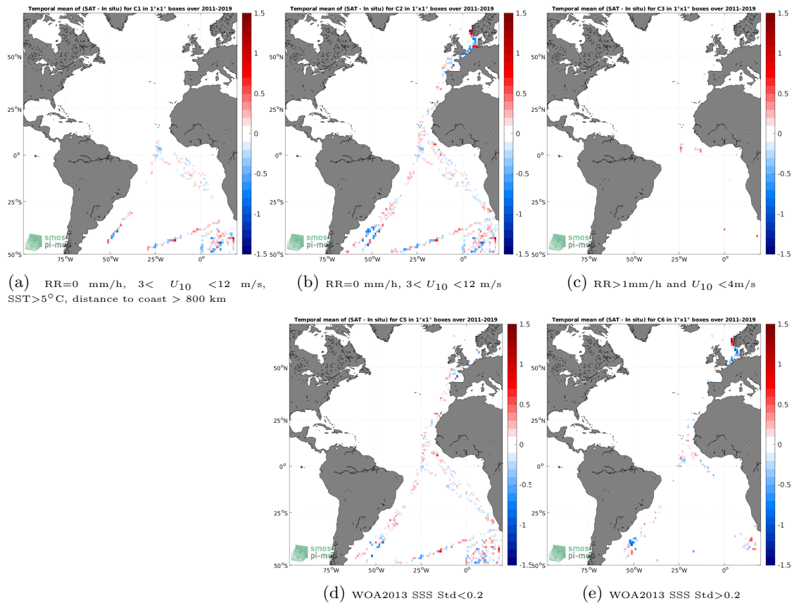
Figure 12: Temporal mean gridded over spatial boxes of size 1^\circ \times 1^\circ of \Delta\text{SSS} (SMOS SSS L4 OI v342 - Weekly (CMEMS-CATDS-LOPS) - TSG (Polarstern)) for 5 different subdatasets corresponding to:RR=0 mm/h, 3 < U_{10} < 12 m/s, SST >5^\circ\text{C} , distance to coast > 800 km (a), RR=0 mm/h, 3 < U_{10} < 12 m/s (b), RR >1 mm/h and U_{10} < 4 m/s (c), WOA2013 SSS Std <0.2 (d), WOA2013 SSS Std >0.2 (e).
