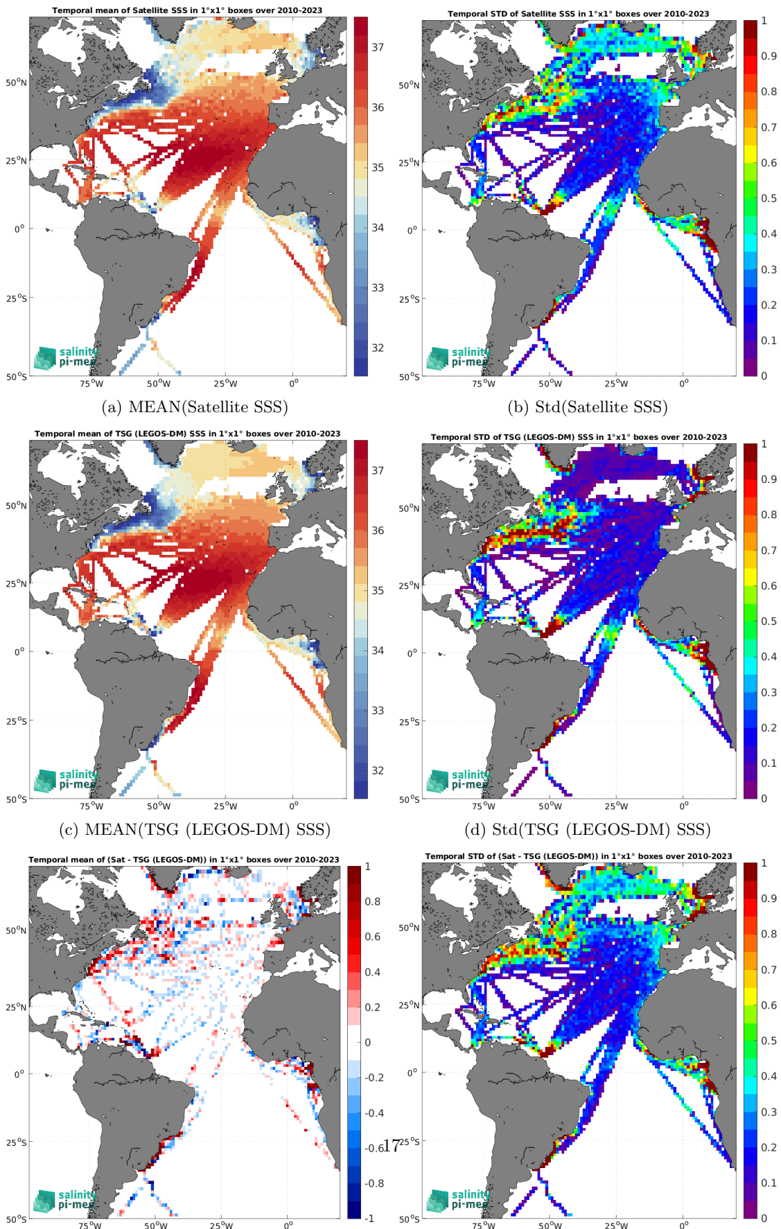
Figure 6: Temporal mean (left) and Std (right) of SSS from SMOS SSS L4 OI v342 - Weekly (CMEMS-CATDS-LOPS) (top), TSG (LEGOS-DM) (middle), and of \Delta SSS (Satellite - TSG (LEGOS-DM)). Only match-up pairs are used to generate these maps.
