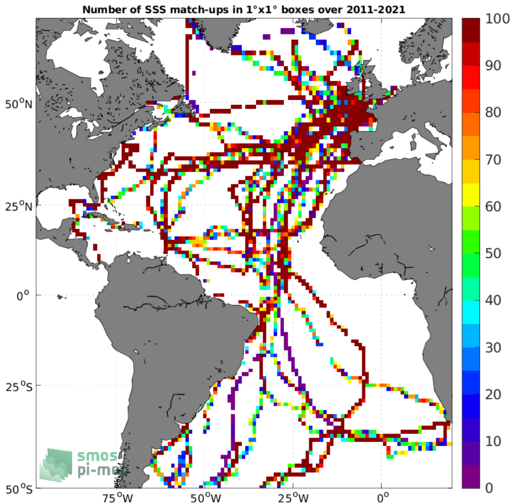
Figure 4: Number of SSS match-ups between TSG (GOSUD-Sailing-ship) SSS and the SMOS SSS L4 OI v342 - Weekly (CMEMS-CATDS-LOPS) SSS product for the Atlantic Ocean Pi-MEP region over 1^\circ \times 1^\circ boxes and for the full satellite product period.
