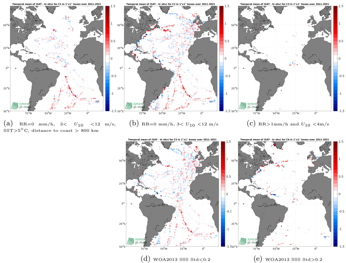
Figure 12: Temporal mean gridded over spatial boxes of size 1^\circ \times 1^\circ of \Delta\text{SSS} (SMOS SSS L4 OI v342 - Weekly (CMEMS-CATDS-LOPS) - TSG (GOSUD-Sailing-ship)) for 5 different sub-datasets corresponding to:RR=0 mm/h, 3 < U_{10} < 12 m/s, SST>5°C, distance to coast > 800 km (a), RR=0 mm/h, 3 < U_{10} < 12 m/s (b), RR>1mm/h and U_{10} < 4 m/s (c), WOA2013 SSS Std<0.2 (d), WOA2013 SSS Std>0.2 (e).
