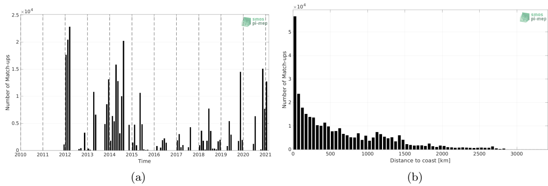
Figure 1: Number of match-ups between TSG (GOSUD-Sailing-ship) and SMOS SSS L4 OI v342 - Weekly (CMEMS-CATDS-LOPS) SSS as a function of time (a) and as function of the distance to coast (b) over the Atlantic Ocean Pi-MEP region and for the full satellite product period.
