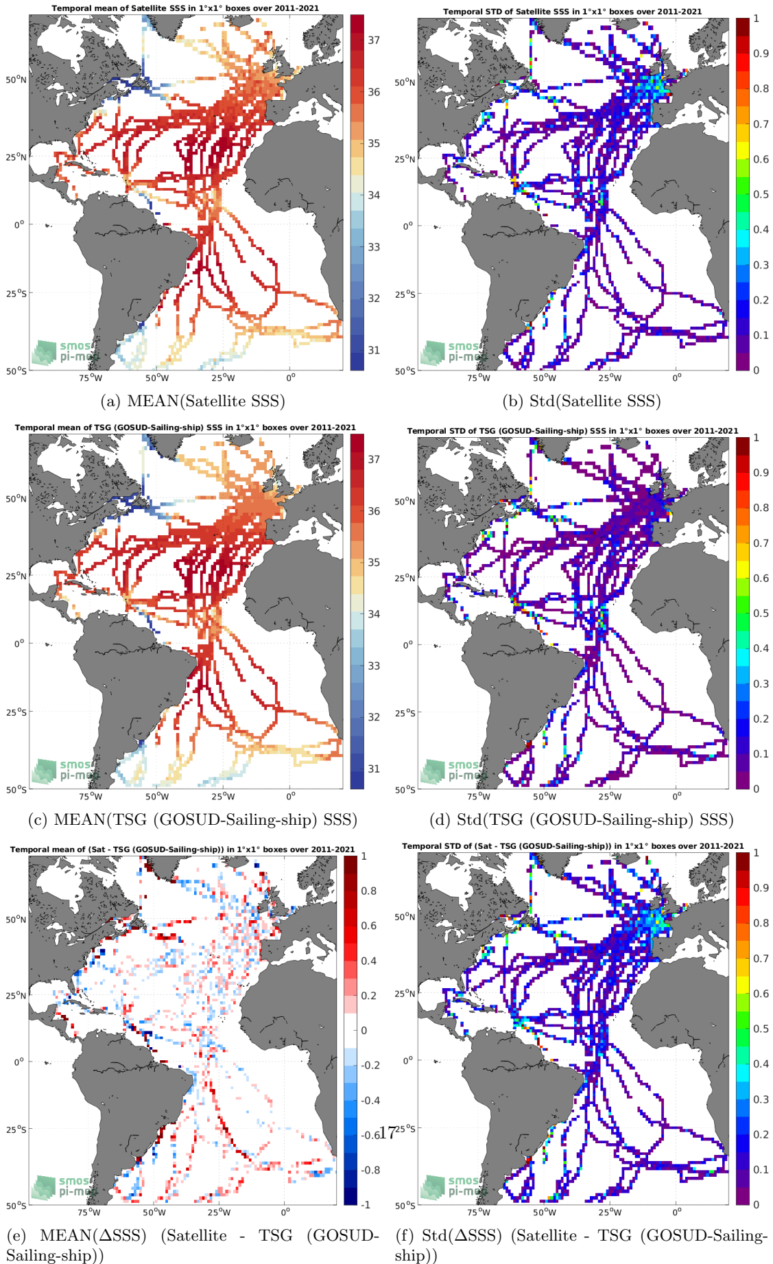
Figure 6: Temporal mean (left) and Std (right) of SSS from SMOS SSS L4 OI v342 - Weekly (CMEMS-CATDS-LOPS) (top), TSG (GOSUD-Sailing-ship) (middle), and of \Delta SSS (Satellite - TSG (GOSUD-Sailing-ship)). Only match-up pairs are used to generate these maps.
