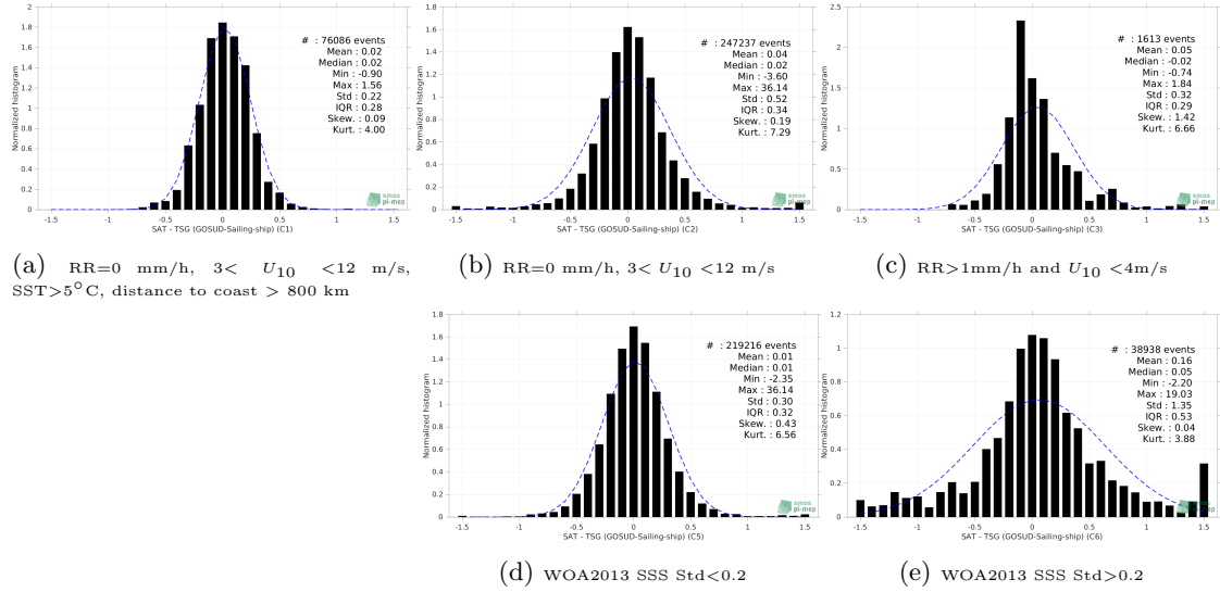
Figure 13: Normalized histogram of \Delta\text{SSS} (SMOS SSS L4 OI v342 - Weekly (CMEMS-CATDS-LOPS) - TSG (GOSUD-Sailing-ship)) for 5 different subdatasets corresponding to: RR=0 mm/h, 3 < U_{10} < 12 m/s, SST >5^{\circ}\text{C} , distance to coast > 800 km (a), RR=0 mm/h, 3 < U_{10} < 12 m/s (b), RR >1 mm/h and U_{10} < 4 m/s (c), WOA2013 SSS Std <0.2 (d), WOA2013 SSS Std >0.2 (e).
