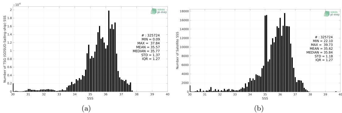
Figure 2: Histograms of SSS from TSG (GOSUD-Sailing-ship) (a) and SMOS SSS L4 OI v342 - Weekly (CMEMS-CATDS-LOPS) (b) considering all match-up pairs per bins of 0.1 over the Atlantic Ocean Pi-MEP region and for the full satellite product period.
