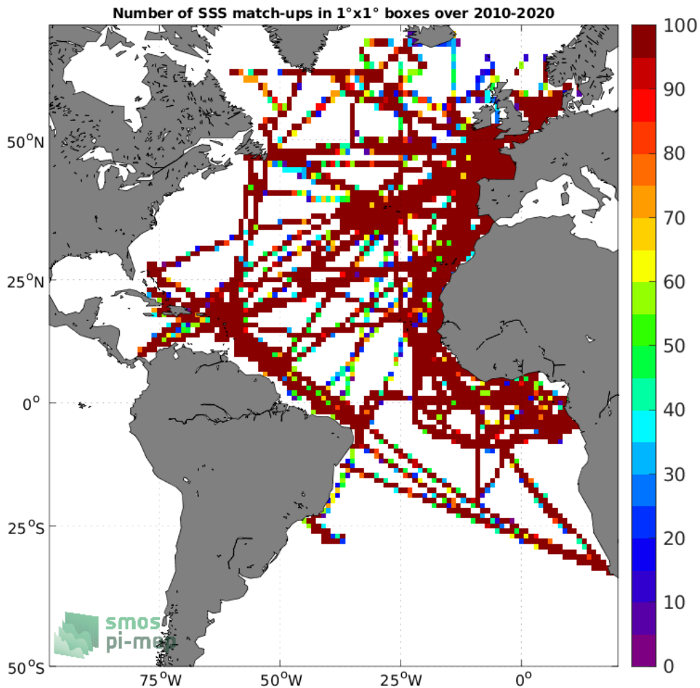
Figure 4: Number of SSS match-ups between TSG (GOSUD-Research-vessel) SSS and the SMOS SSS L4 OI v342 - Weekly (CMEMS-CATDS-LOPS) SSS product for the Atlantic Ocean Pi-MEP region over 1°x1° boxes and for the full satellite product period.
