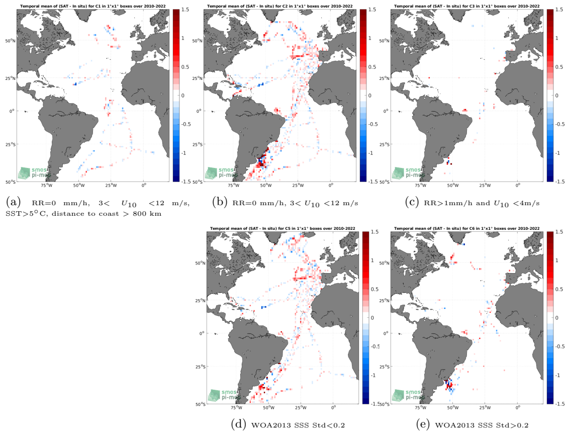
Figure 12: Temporal mean gridded over spatial boxes of size 1^\circ \times 1^\circ of \Delta\text{SSS} (SMOS SSS L4 OI v342 - Weekly (CMEMS-CATDS-LOPS) - TSG (CSIC-UTM)) for 5 different subdatasets corresponding to:RR=0 mm/h, 3 < U_{10} < 12 m/s, SST >5^\circ\text{C} , distance to coast > 800 km (a), RR=0 mm/h, 3 < U_{10} < 12 m/s (b), RR >1 mm/h and U_{10} < 4 m/s (c), WOA2013 SSS Std <0.2 (d), WOA2013 SSS Std >0.2 (e).
