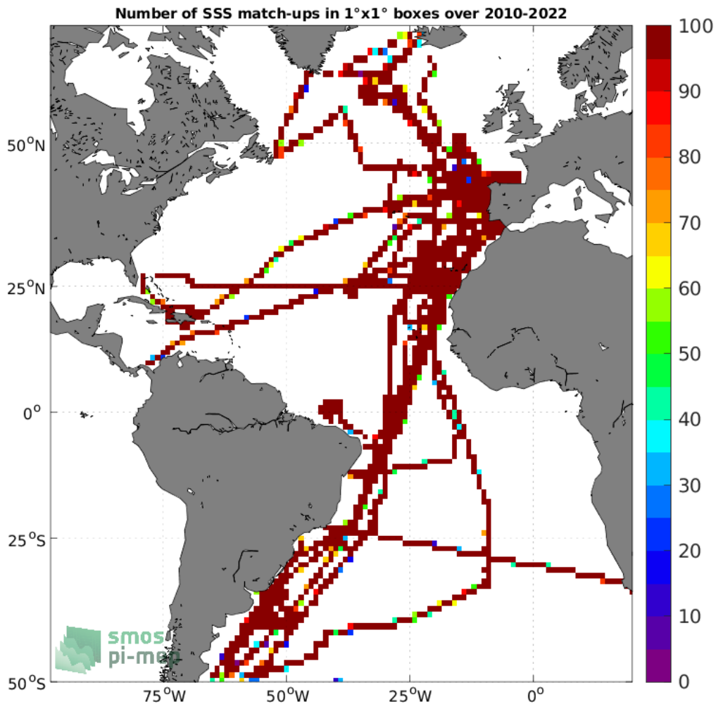
Figure 4: Number of SSS match-ups between TSG (CSIC-UTM) SSS and the SMOS SSS L4 OI v342 - Weekly (CMEMS-CATDS-LOPS) SSS product for the Atlantic Ocean Pi-MEP region over 1°x1° boxes and for the full satellite product period.
