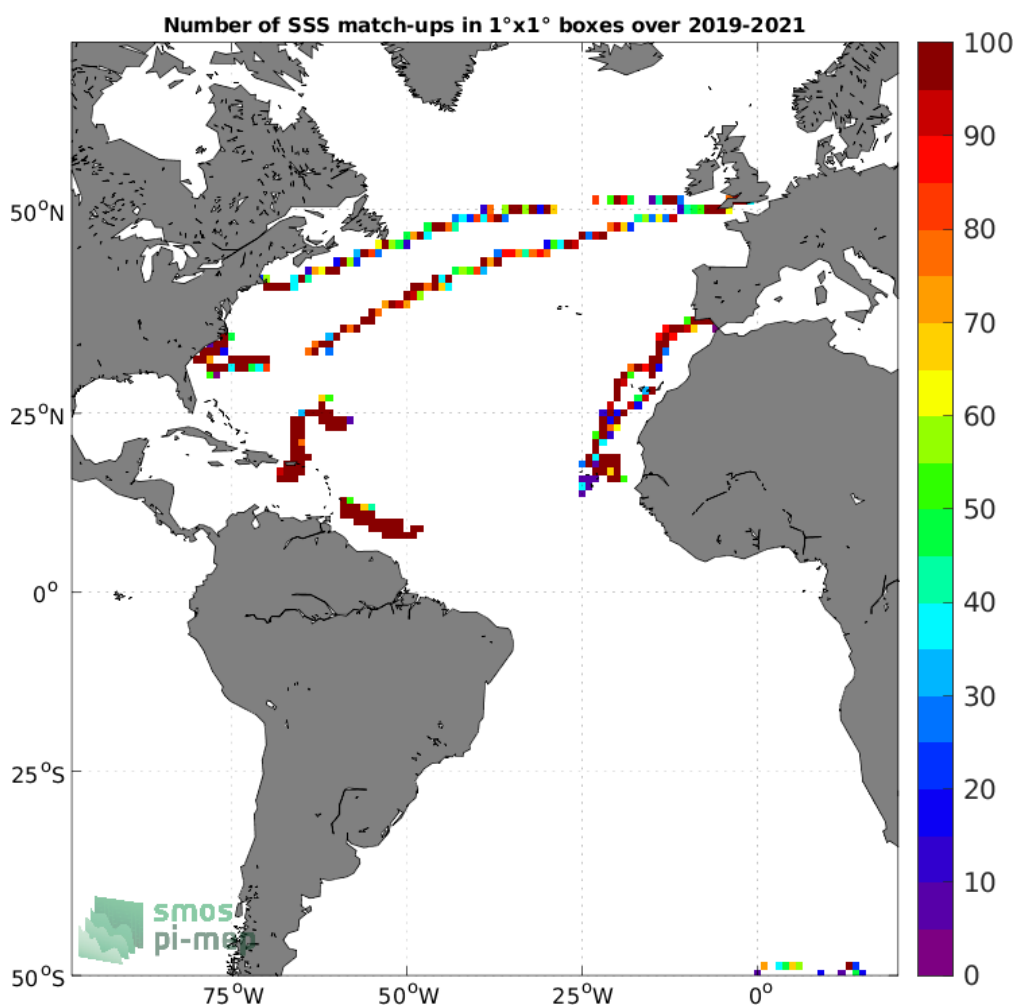
Figure 4: Number of SSS match-ups between Saildrone SSS and the SMOS SSS L4 OI v342 - Weekly (CMEMS-CATDS-LOPS) SSS product for the Atlantic Ocean Pi-MEP region over 1°x1° boxes and for the full satellite product period.
