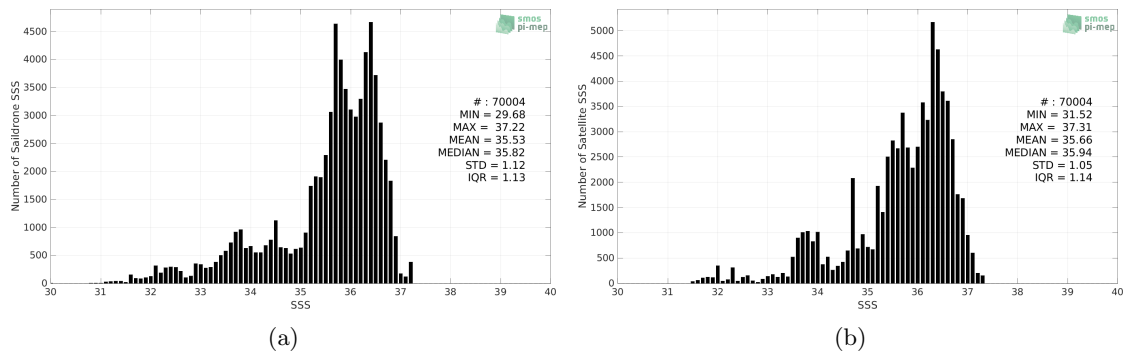
Figure 2: Histograms of SSS from Saildrone (a) and SMOS SSS L4 OI v342 - Weekly (CMEMS-CATDS-LOPS) (b) considering all match-up pairs per bins of 0.1 over the Atlantic Ocean Pi-MEP region and for the full satellite product period.
