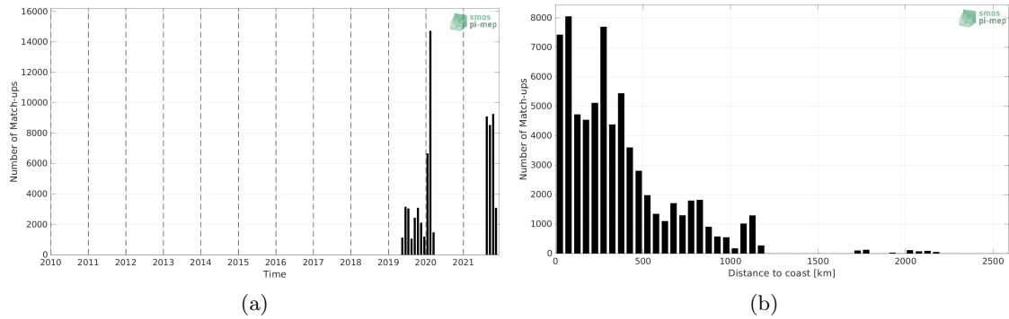
Figure 1: Number of match-ups between Saildrone and SMOS SSS L4 OI v342 - Weekly (CMEMS-CATDS-LOPS) SSS as a function of time (a) and as function of the distance to coast (b) over the Atlantic Ocean Pi-MEP region and for the full satellite product period.
