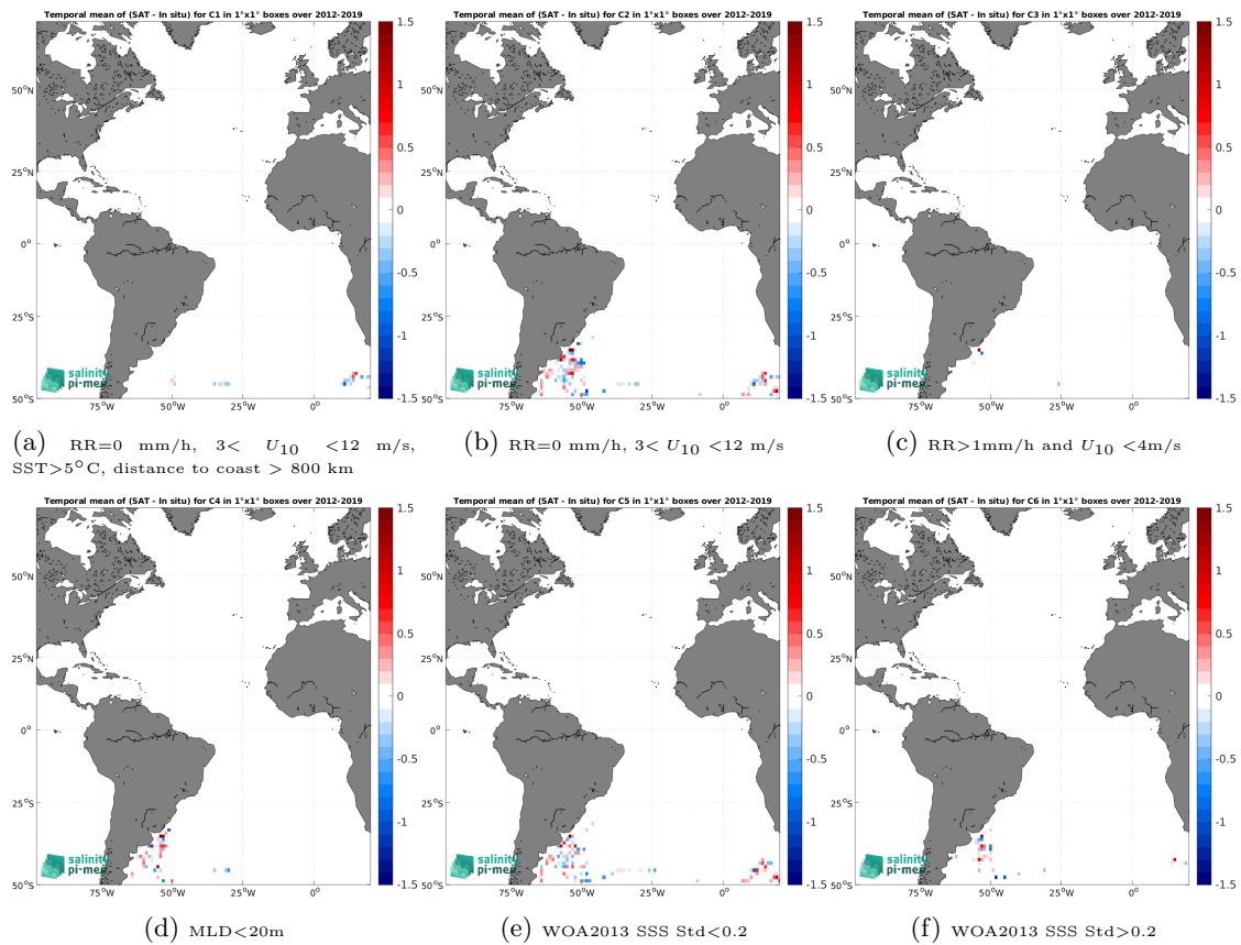
Figure 12: Temporal mean gridded over spatial boxes of size 1^\circ \times 1^\circ of \Delta SSS (SMOS SSS L4 OI v342 - Weekly (CMEMS-CATDS-LOPS) - Marine mammals) for 6 different subdatasets corresponding to: RR=0 mm/h, 3 < U_{10} < 12 m/s, SST > 5°C, distance to coast > 800 km (a), RR=0 mm/h, 3 < U_{10} < 12 m/s (b), RR > 1mm/h and U_{10} < 4 m/s (c), MLD < 20m (d), WOA2013 SSS Std < 0.2 (e), WOA2013 SSS Std > 0.2 (f).
