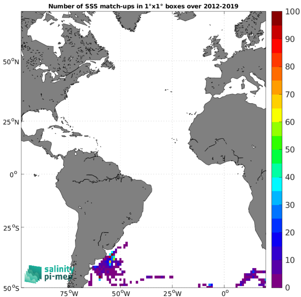
Figure 4: Number of SSS match-ups between Marine mammals SSS and the SMOS SSS L4 OI v342 - Weekly (CMEMS-CATDS-LOPS) SSS product for the Atlantic Ocean Pi-MEP region over 1°x1° boxes and for the full satellite product period.
