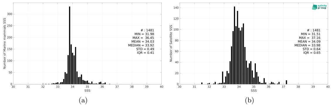
Figure 2: Histograms of SSS from Marine mammals (a) and SMOS SSS L4 OI v342 - Weekly (CMEMS-CATDS-LOPS) (b) considering all match-up pairs per bins of 0.1 over the Atlantic Ocean Pi-MEP region and for the full satellite product period.
