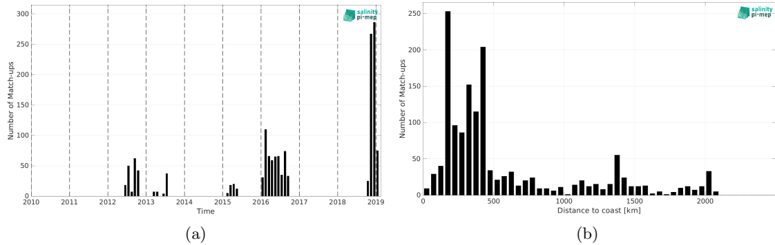
Figure 1: Number of match-ups between Marine mammals and SMOS SSS L4 OI v342 - Weekly (CMEMS-CATDS-LOPS) SSS as a function of time (a) and as function of the distance to coast (b) over the Atlantic Ocean Pi-MEP region and for the full satellite product period.
