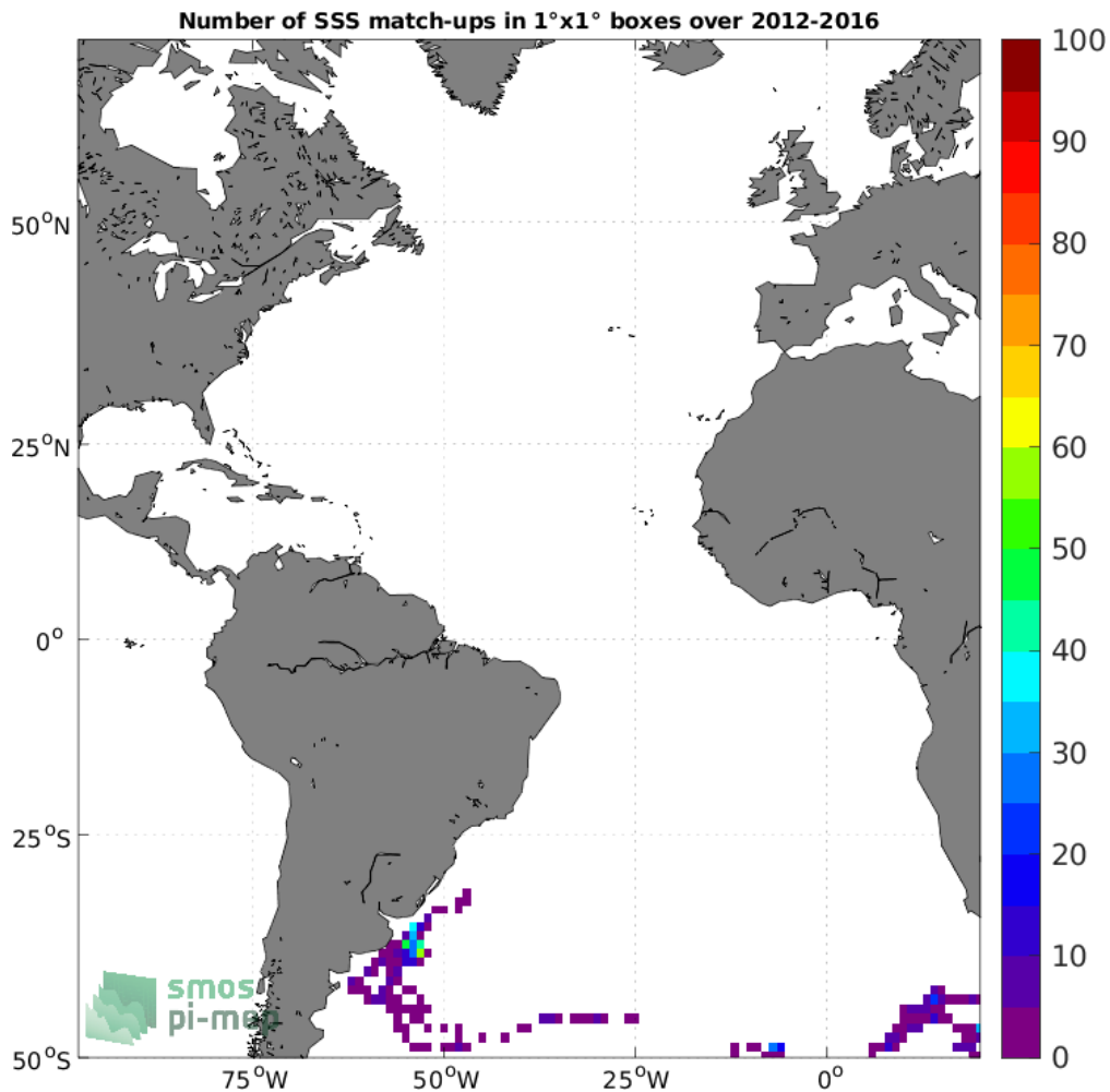
Figure 4: Number of SSS match-ups between Marine mammals SSS and the SMOS SSS L4 OI v342 - Weekly (CMEMS-CATDS-LOPS) SSS product for the Atlantic Ocean Pi-MEP region over 1^\circ \times 1^\circ boxes and for the full satellite product period.
