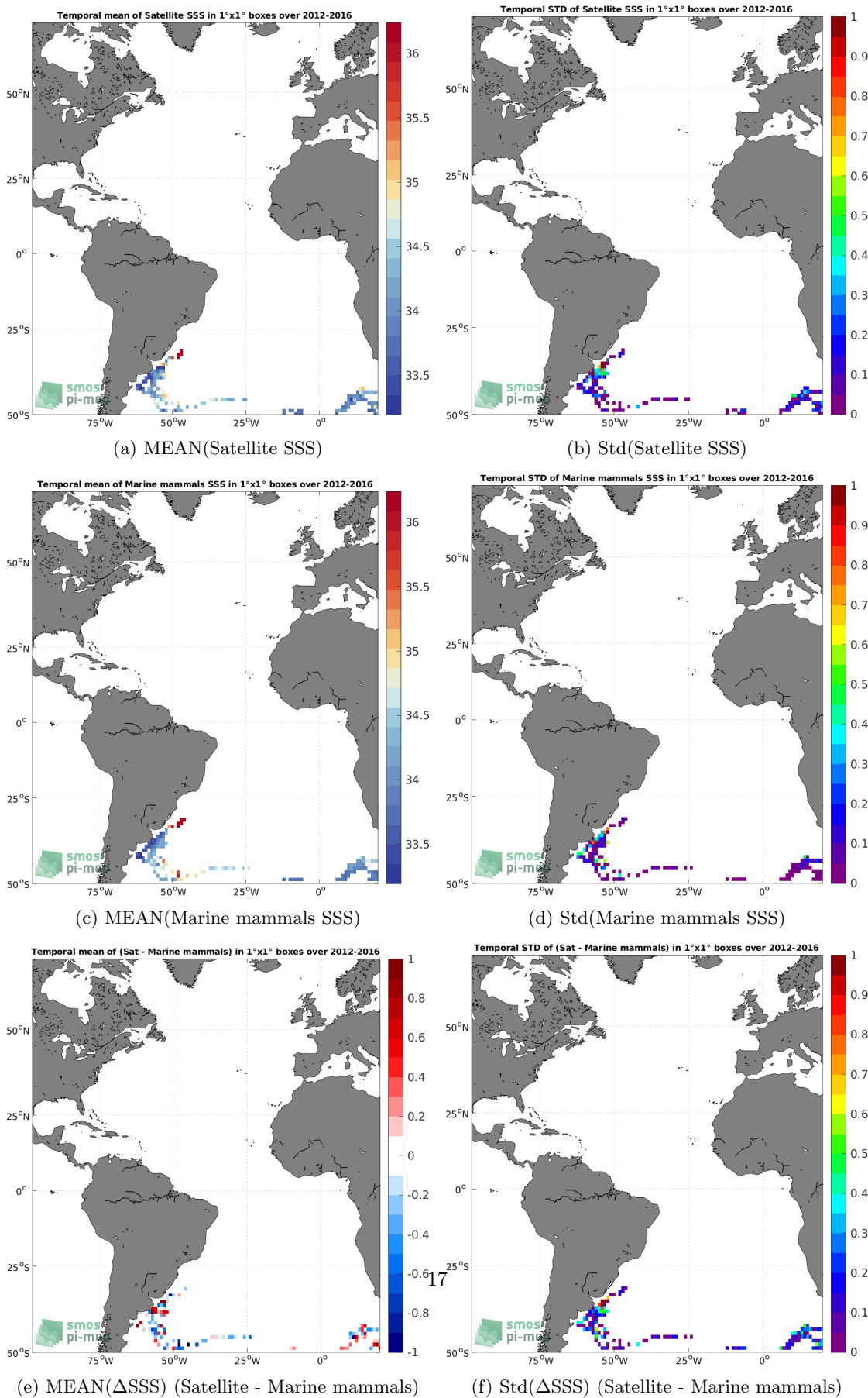
Figure 6: Temporal mean (left) and Std (right) of SSS from SMOS SSS L4 OI v342 - Weekly (CMEMS-CATDS-LOPS) (top), Marine mammals (middle), and of \Delta SSS (Satellite - Marine mammals). Only match-up pairs are used to generate these maps.
