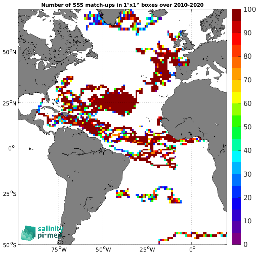
Figure 3: Number of SSS match-ups between Surface drifters SSS and the SMOS SSS L4 OI v342 - Weekly (CMEMS-CATDS-LOPS) SSS product for the Atlantic Ocean Pi-MEP region over 1°x1° boxes and for the full satellite product period.
