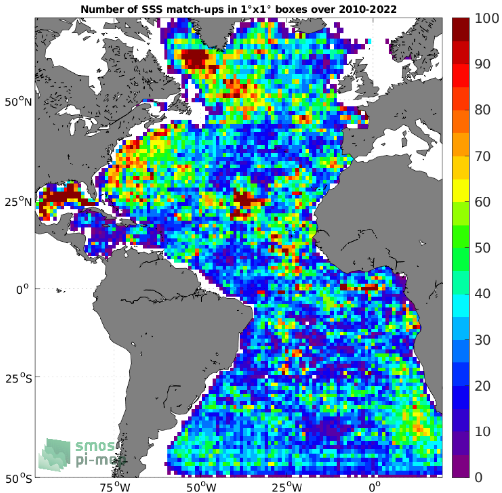
Figure 4: Number of SSS match-ups between Argo SSS and the SMOS SSS L4 OI v342 - Weekly (CMEMS-CATDS-LOPS) SSS product for the Atlantic Ocean Pi-MEP region over 1°x1° boxes and for the full satellite product period.
