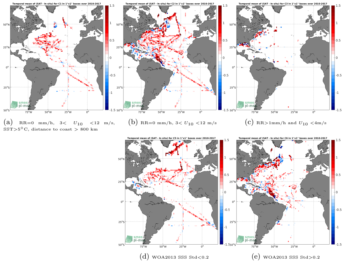
Figure 12: Temporal mean gridded over spatial boxes of size 1^\circ \times 1^\circ of \Delta SSS (SMOS L4 v2 Weekly (CATDS-CECOS-IFREMER) - TSG (SAMOS)) for 5 different subdatasets corresponding to:RR=0 mm/h, 3 < U_{10} < 12 m/s, SST >5^\circ\text{C} , distance to coast > 800 km (a), RR=0 mm/h, 3 < U_{10} < 12 m/s (b), RR >1 mm/h and U_{10} < 4 m/s (c), WOA2013 SSS Std <0.2 (d), WOA2013 SSS Std >0.2 (e).
