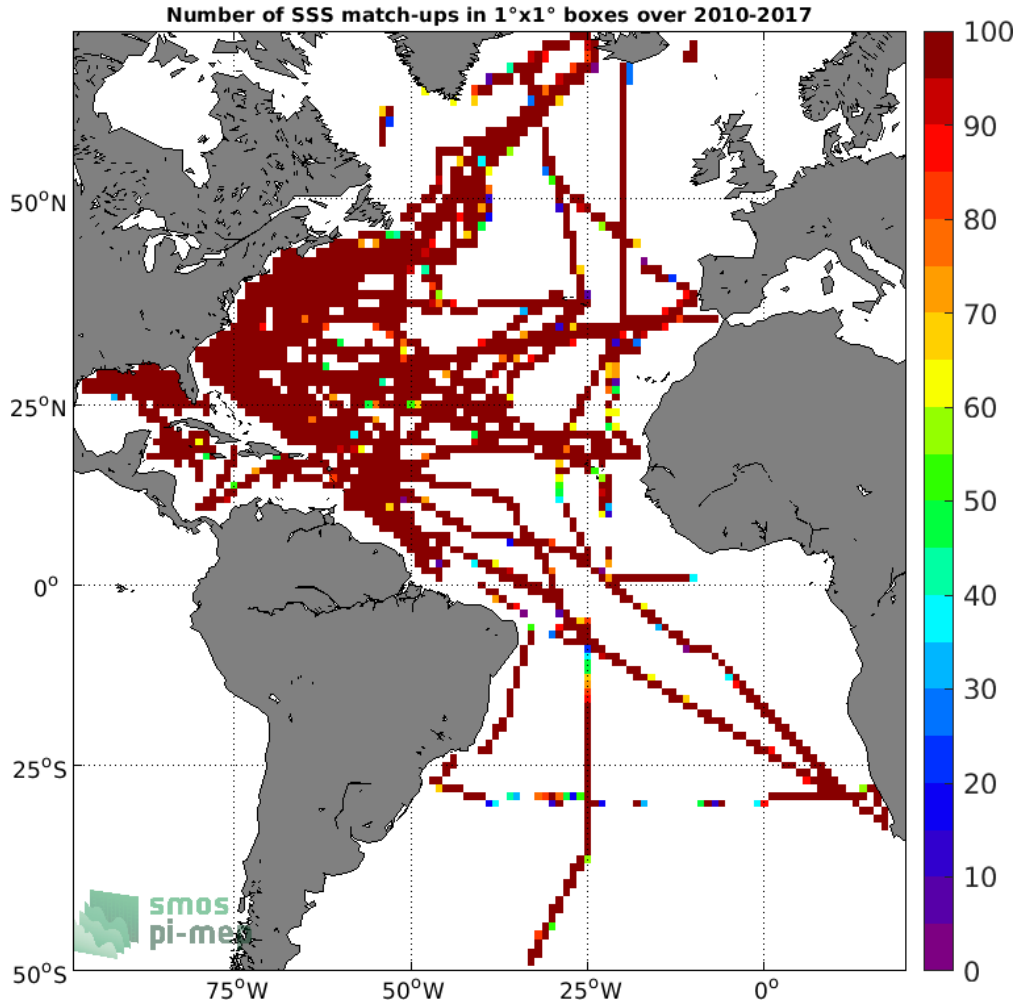
Figure 4: Number of SSS match-ups between TSG (SAMOS) SSS and the SMOS L4 v2 Weekly (CATDS-CECOS-IFREMER) SSS product for the Atlantic Ocean Pi-MEP region over 1^\circ \times 1^\circ boxes and for the full satellite product period.
