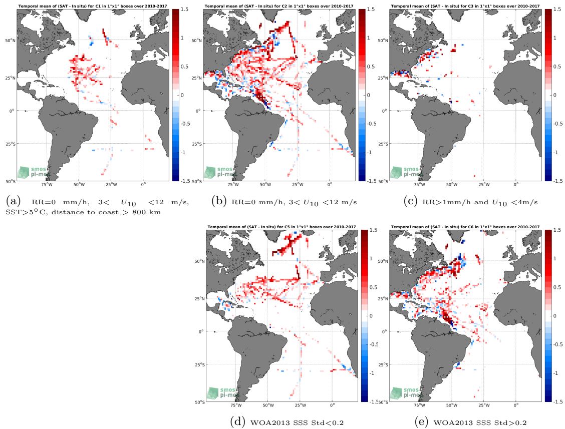
Figure 12: Temporal mean gridded over spatial boxes of size 1^\circ \times 1^\circ of \Delta SSS (SMOS-L4-CATDS-CECOS-IFREMER-V2-WEEKLY-0.5DEG - TSG-SAMOS) for 5 different subdatasets corresponding to:RR=0 mm/h, 3 < U_{10} < 12 m/s, SST >5^\circ\text{C} , distance to coast > 800 km (a), RR=0 mm/h, 3 < U_{10} < 12 m/s (b), RR >1 mm/h and U_{10} < 4 m/s (c), WOA2013 SSS Std <0.2 (d), WOA2013 SSS Std >0.2 (e).
