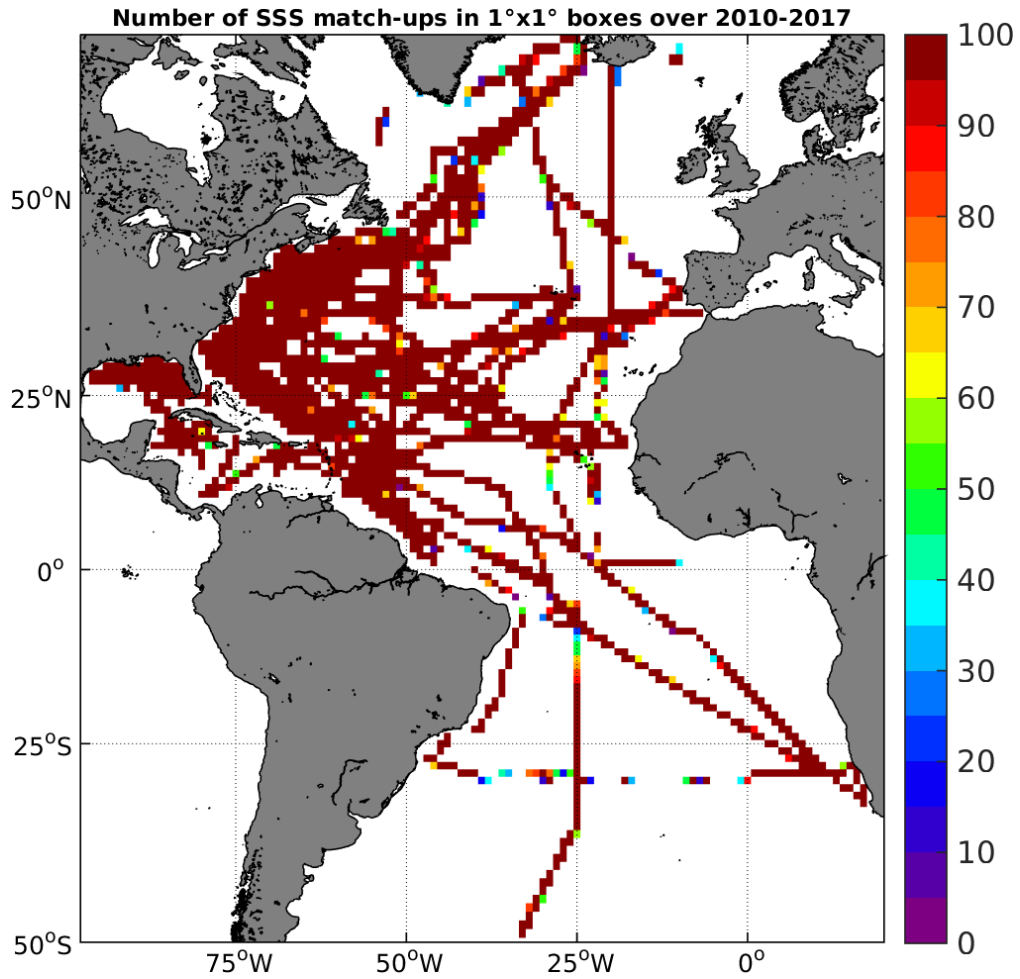
Figure 4: Number of SSS match-ups between TSG-SAMOS SSS and the SMOS-L4-CATDS-CECOS-IFREMER-V2-WEEKLY-0.5DEG SSS product for the Atlantic Ocean Pi-MEP region over 1°x1° boxes and for the full satellite product period.
