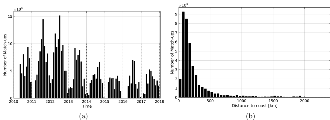
Figure 1: Number of match-ups between TSG-SAMOS and SMOS-L4-CATDS-CECOS-IFREMER-V2-WEEKLY-0.5DEG SSS as a function of time (a) and as function of the distance to coast (b) over the Atlantic Ocean Pi-MEP region and for the full satellite product period.
