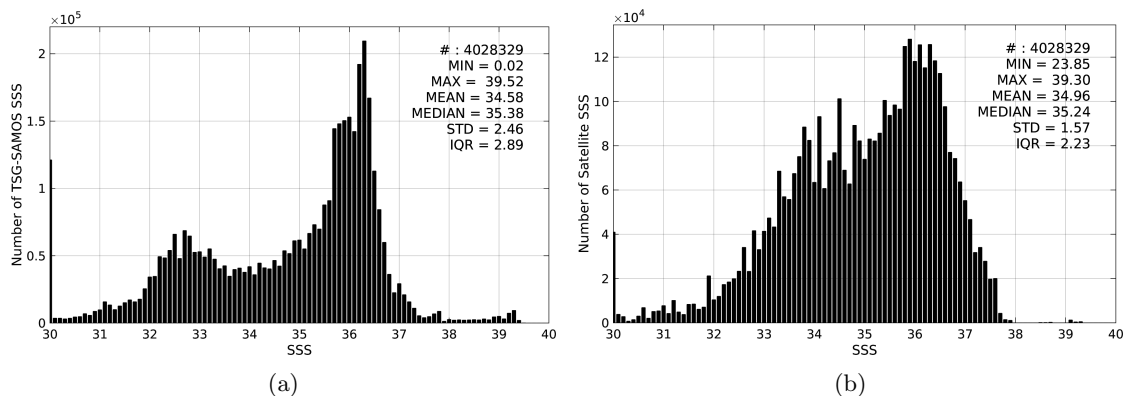
Figure 2: Histograms of SSS from TSG-SAMOS (a) and SMOS-L4-CATDS-CECOS-IFREMER-V2-WEEKLY-0.5DEG (b) considering all match-up pairs per bins of 0.1 over the Atlantic Ocean Pi-MEP region and for the full satellite product period.
