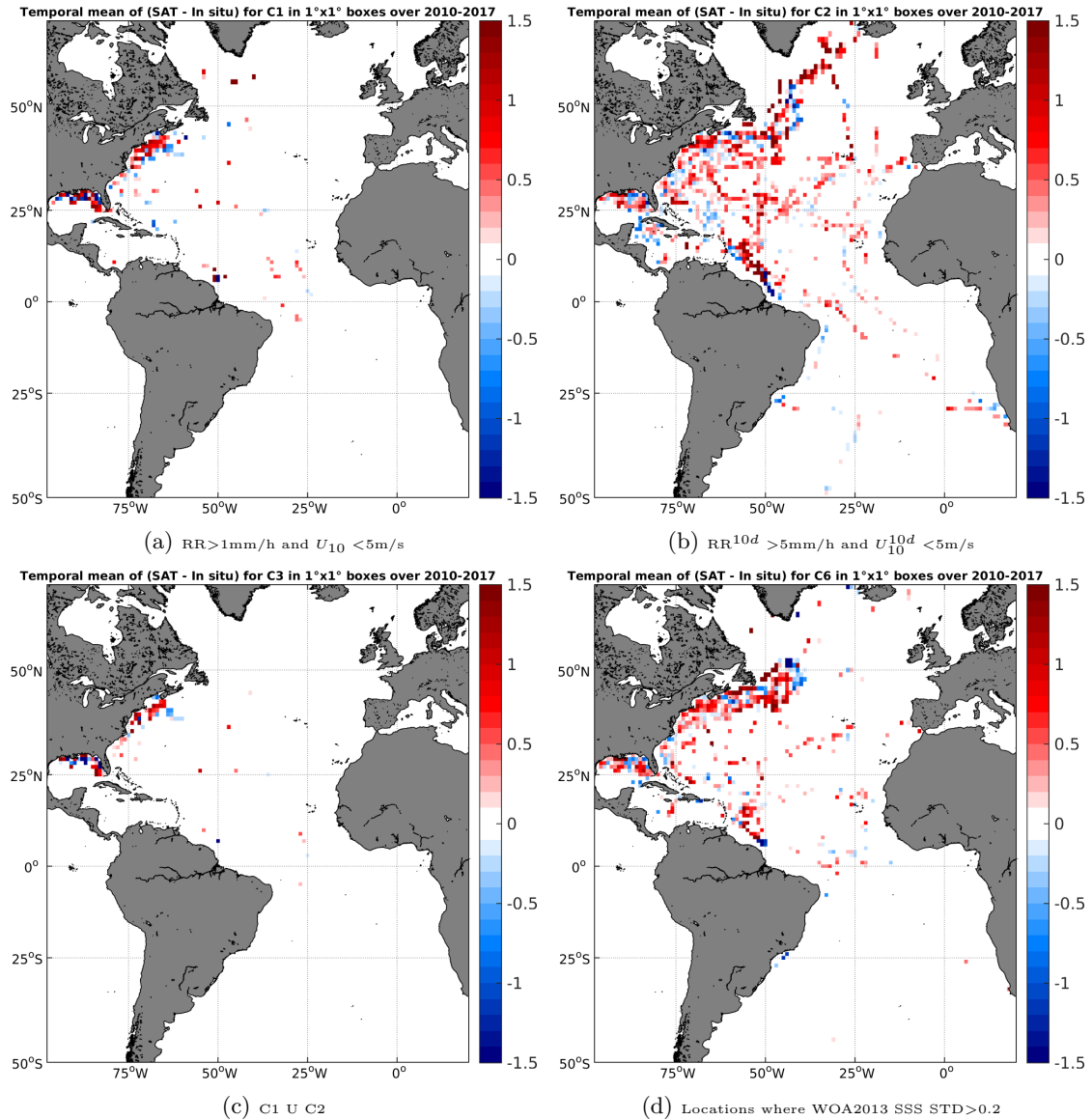
Figure 12: Temporal mean gridded over spatial boxes of size 1^\circ \times 1^\circ of \Delta SSS (SMOS-L4-CATDS-CECOS-IFREMER-V2-WEEKLY-0.5DEG - TSG-SAMOS) for 4 different subdatasets corresponding to: RR > 1\text{mm/h} and U_{10} < 5\text{m/s} (a), RR^{10d} > 5\text{mm/h} and U_{10}^{10d} < 5\text{m/s} (b), C1 U C2 (c), Locations where WOA2013 SSS STD > 0.2 (d).
