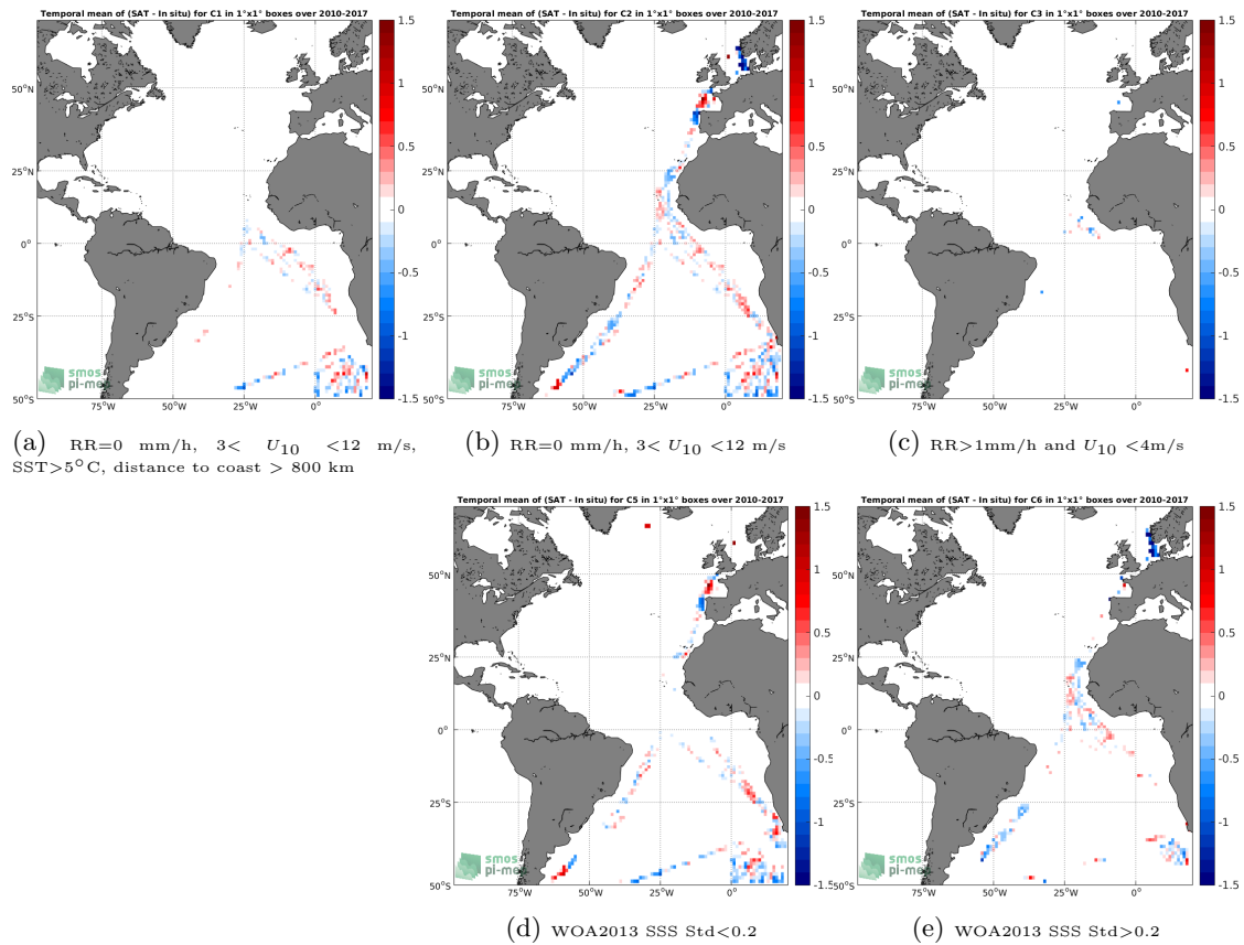
Figure 12: Temporal mean gridded over spatial boxes of size 1^\circ \times 1^\circ of \Delta SSS (SMOS-L4-CATDS-CECOS-IFREMER-V2-WEEKLY-0.5DEG - TSG-POLARSTERN) for 5 different subdatasets corresponding to:RR=0 mm/h, 3 < U_{10} < 12 m/s, SST >5^\circ\text{C} , distance to coast > 800 km (a), RR=0 mm/h, 3 < U_{10} < 12 m/s (b), RR >1 mm/h and U_{10} < 4 m/s (c), WOA2013 SSS Std <0.2 (d), WOA2013 SSS Std >0.2 (e).
