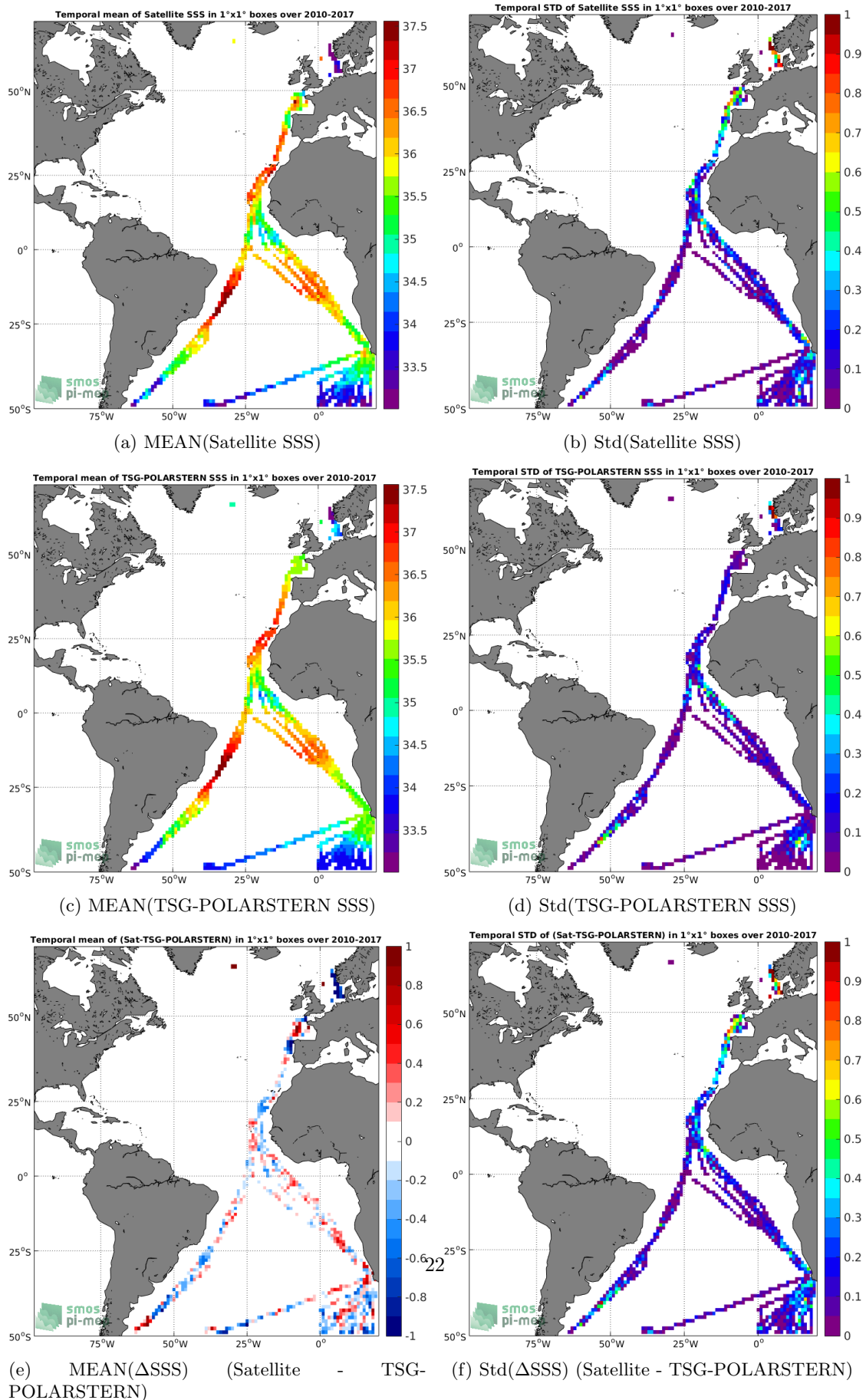
Figure 6: Temporal mean (left) and Std (right) of SSS from SMOS-L4-CATDS-CECOS-IFREMER-V2-WEEKLY-0.5DEG (top), TSG-POLARSTERN (middle), and of \Delta SSS (Satellite - TSG-POLARSTERN). Only match-up pairs are used to generate these maps.
