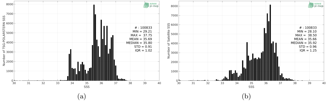
Figure 2: Histograms of SSS from TSG-POLARSTERN (a) and SMOS-L4-CATDS-CECOS-IFREMER-V2-WEEKLY-0.5DEG (b) considering all match-up pairs per bins of 0.1 over the Atlantic Ocean Pi-MEP region and for the full satellite product period.
