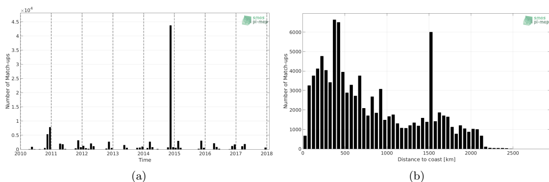
Figure 1: Number of match-ups between TSG-POLARSTERN and SMOS-L4-CATDS-CECOS-IFREMER-V2-WEEKLY-0.5DEG SSS as a function of time (a) and as function of the distance to coast (b) over the Atlantic Ocean Pi-MEP region and for the full satellite product period.
