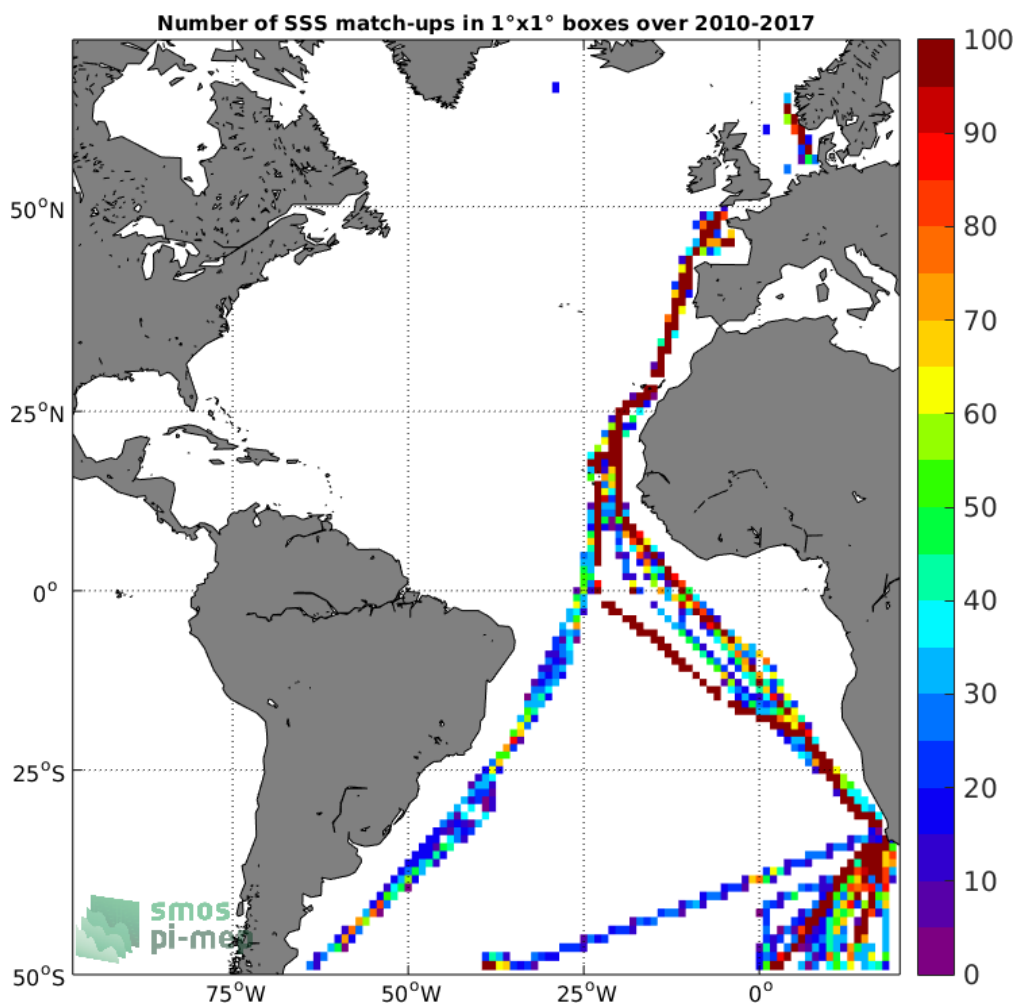
Figure 4: Number of SSS match-ups between TSG-POLARSTERN SSS and the SMOS-L4-CATDS-CECOS-IFREMER-V2-WEEKLY-0.5DEG SSS product for the Atlantic Ocean Pi-MEP region over 1°x1° boxes and for the full satellite product period.
