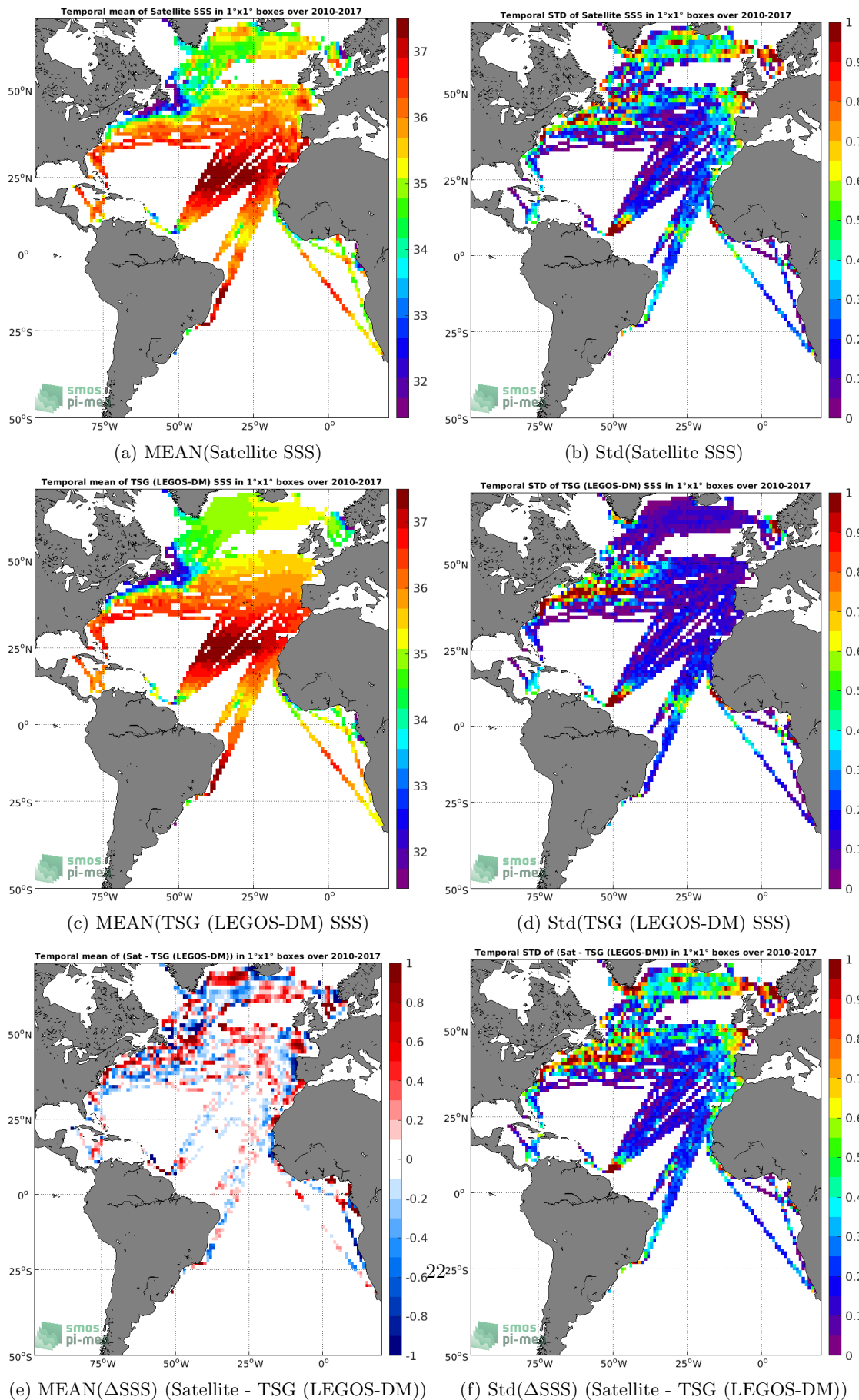
Figure 6: Temporal mean (left) and Std (right) of SSS from SMOS L4 v2 Weekly (CATDS-CECOS-IFREMER) (top), TSG (LEGOS-DM) (middle), and of \Delta SSS (Satellite - TSG (LEGOS-DM)). Only match-up pairs are used to generate these maps.
