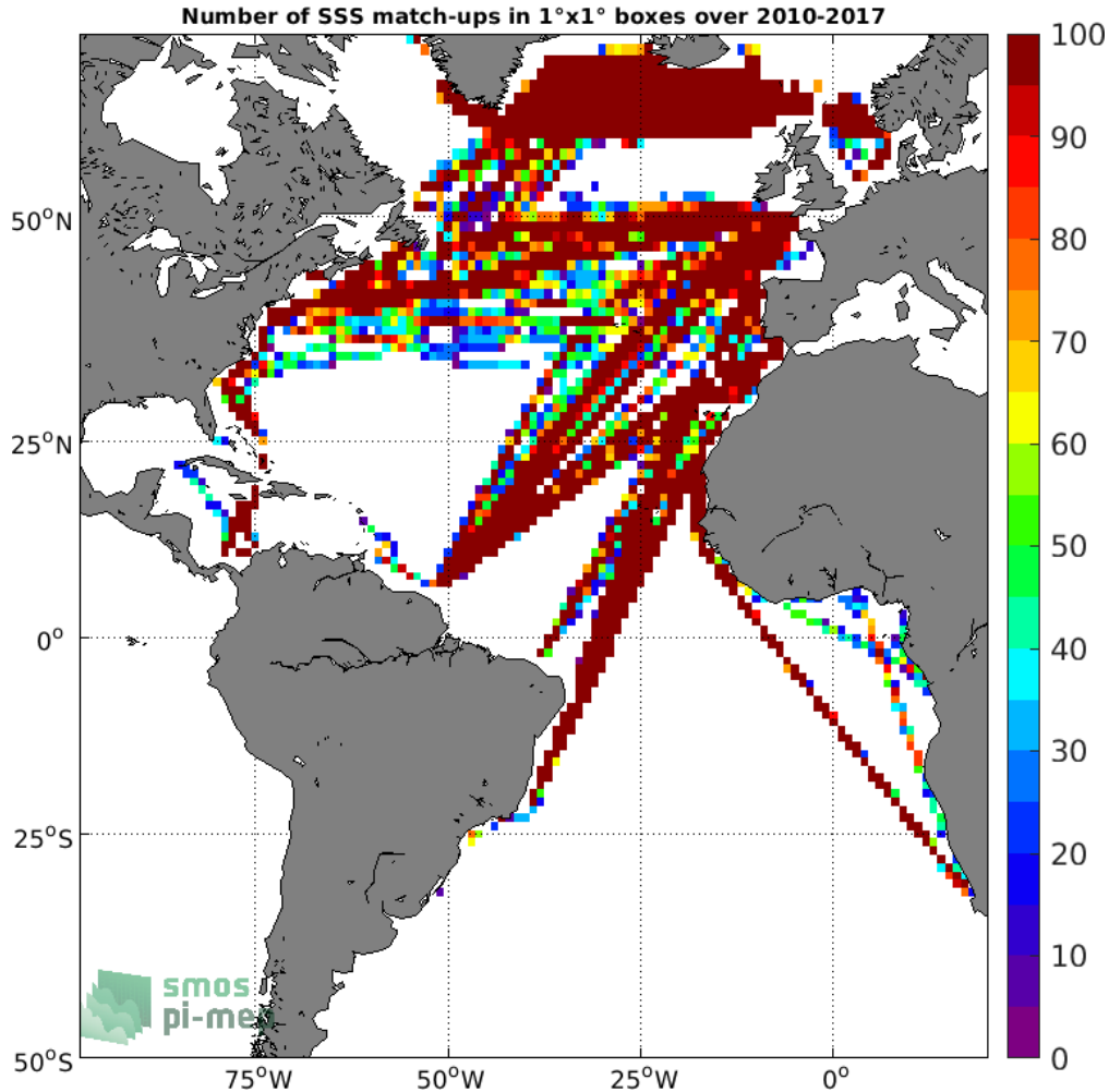
Figure 4: Number of SSS match-ups between TSG (LEGOS-DM) SSS and the SMOS L4 v2 Weekly (CATDS-CECOS-IFREMER) SSS product for the Atlantic Ocean Pi-MEP region over 1^\circ \times 1^\circ boxes and for the full satellite product period.
