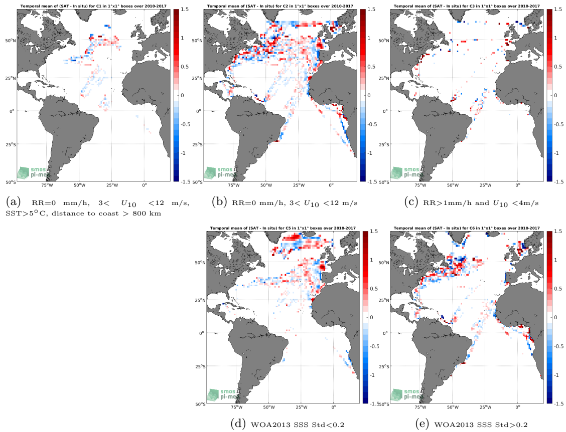
Figure 12: Temporal mean gridded over spatial boxes of size 1^\circ \times 1^\circ of \Delta SSS (SMOS L4 v2 Weekly (CATDS-CECOS-IFREMER) - TSG (LEGOS-DM)) for 5 different subdatasets corresponding to:RR=0 mm/h, 3 < U_{10} < 12 m/s, SST >5^\circ\text{C} , distance to coast > 800 km (a), RR=0 mm/h, 3 < U_{10} < 12 m/s (b), RR >1 mm/h and U_{10} < 4 m/s (c), WOA2013 SSS Std <0.2 (d), WOA2013 SSS Std >0.2 (e).
