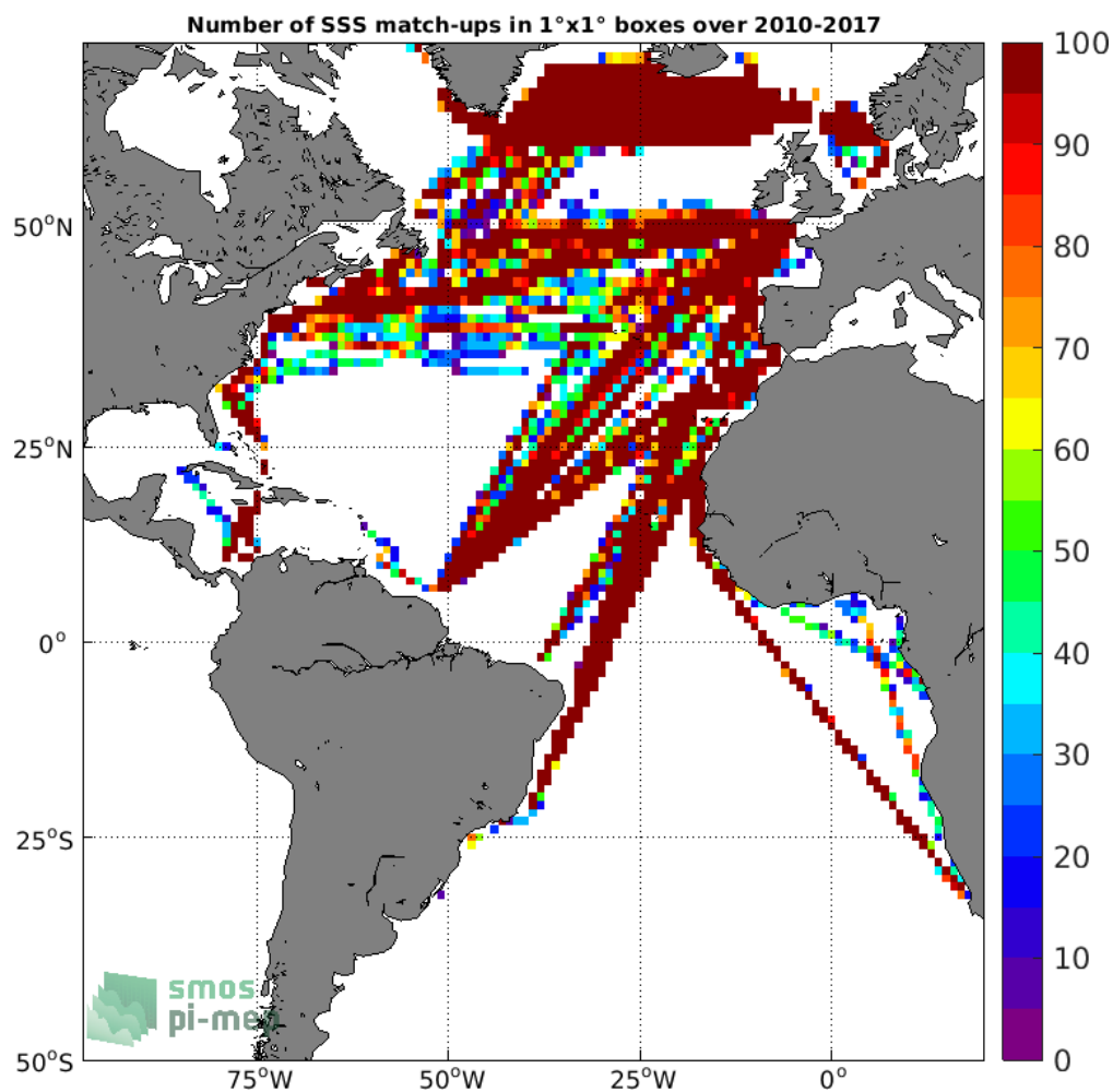
Figure 4: Number of SSS match-ups between TSG (LEGOS-DM) SSS and the SMOS L4 v2 Weekly (CATDS-CECOS-IFREMER) SSS product for the Atlantic Ocean Pi-MEP region over 1°x1° boxes and for the full satellite product period.
