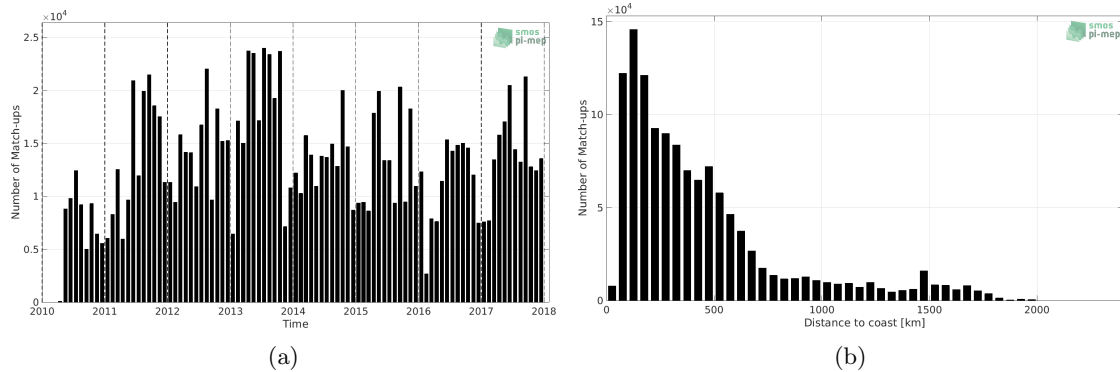
Figure 1: Number of match-ups between TSG (LEGOS-DM) and SMOS L4 v2 Weekly (CATDS-CECOS-IFREMER) SSS as a function of time (a) and as function of the distance to coast (b) over the Atlantic Ocean Pi-MEP region and for the full satellite product period.
