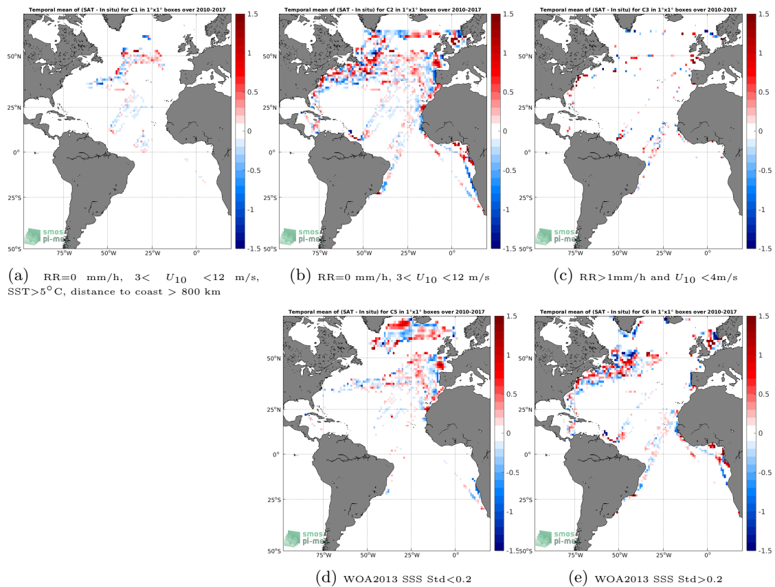
Figure 12: Temporal mean gridded over spatial boxes of size 1^\circ \times 1^\circ of \Delta SSS (SMOS L4 v2 Weekly (CATDS-CECOS-IFREMER) - TSG (LEGOS-DM)) for 5 different subdatasets corresponding to:RR=0 mm/h, 3 < U_{10} < 12 m/s, SST >5^\circ\text{C} , distance to coast > 800 km (a), RR=0 mm/h, 3 < U_{10} < 12 m/s (b), RR >1 mm/h and U_{10} < 4 m/s (c), WOA2013 SSS Std <0.2 (d), WOA2013 SSS Std >0.2 (e).
