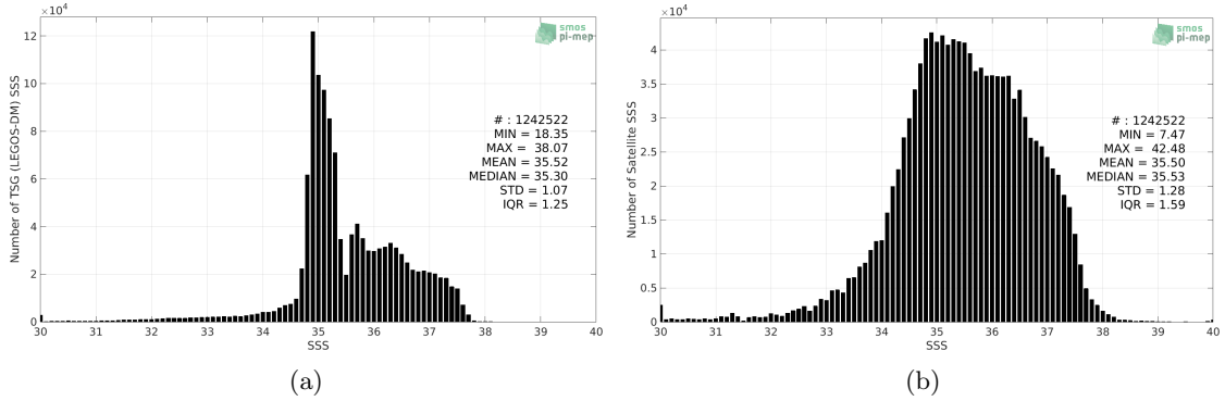
Figure 2: Histograms of SSS from TSG (LEGOS-DM) (a) and SMOS L4 v2 Weekly (CATDS-CECOS-IFREMER) (b) considering all match-up pairs per bins of 0.1 over the Atlantic Ocean Pi-MEP region and for the full satellite product period.
