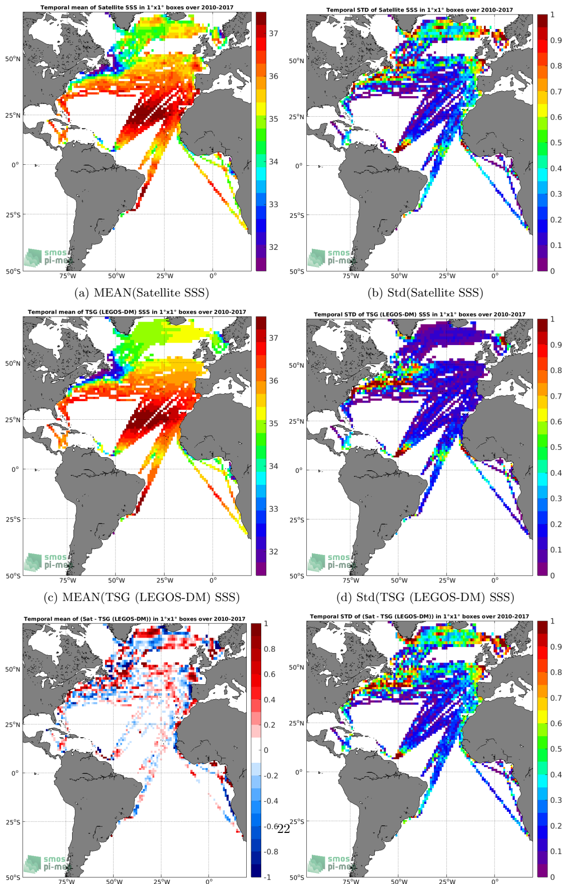
Figure 6: Temporal mean (left) and Std (right) of SSS from SMOS L4 v2 Weekly (CATDS-CECOS-IFREMER) (top), TSG (LEGOS-DM) (middle), and of \Delta SSS (Satellite - TSG (LEGOS-DM)). Only match-up pairs are used to generate these maps.
