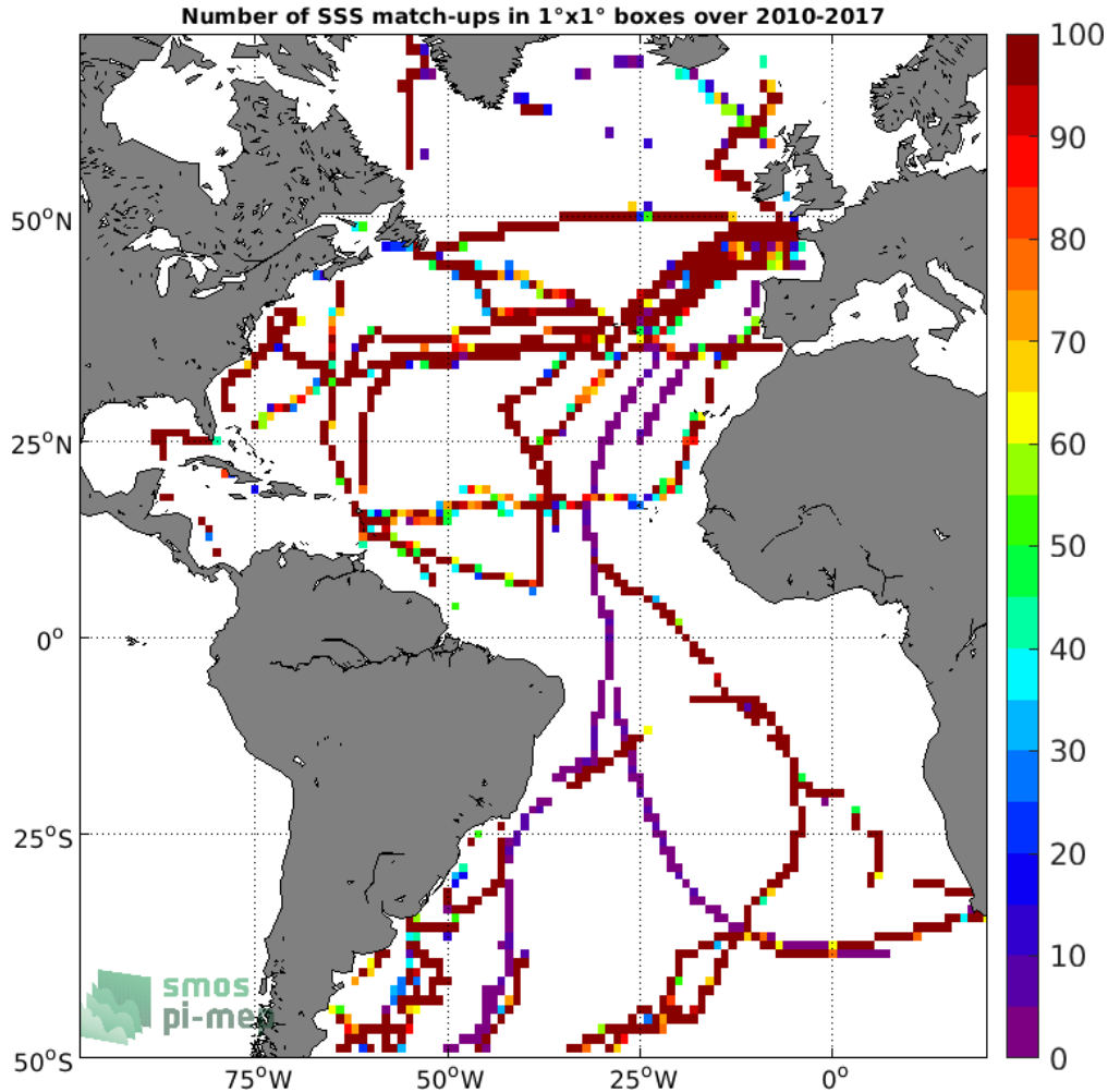
Figure 4: Number of SSS match-ups between TSG (GOSUD-Sailing-ship) SSS and the SMOS L4 v2 Weekly (CATDS-CECOS-IFREMER) SSS product for the Atlantic Ocean Pi-MEP region over 1^\circ \times 1^\circ boxes and for the full satellite product period.
