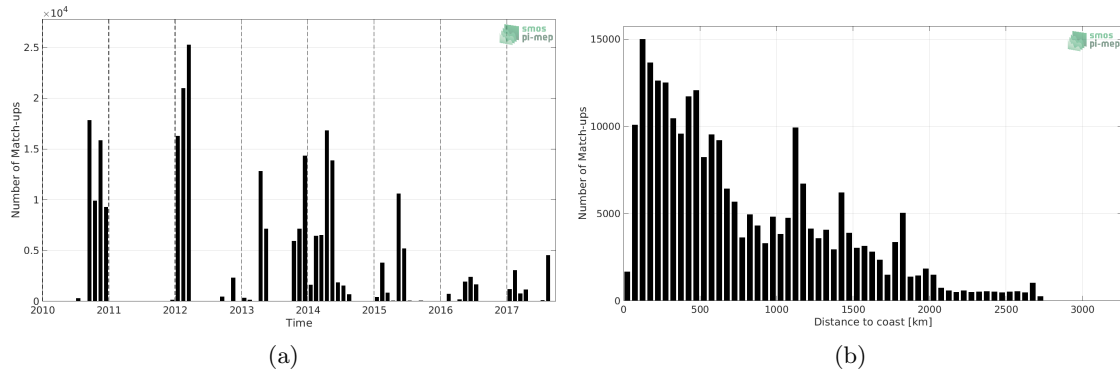
Figure 1: Number of match-ups between TSG (GOSUD-Sailing-ship) and SMOS L4 v2 Weekly (CATDS-CECOS-IFREMER) SSS as a function of time (a) and as function of the distance to coast (b) over the Atlantic Ocean Pi-MEP region and for the full satellite product period.
