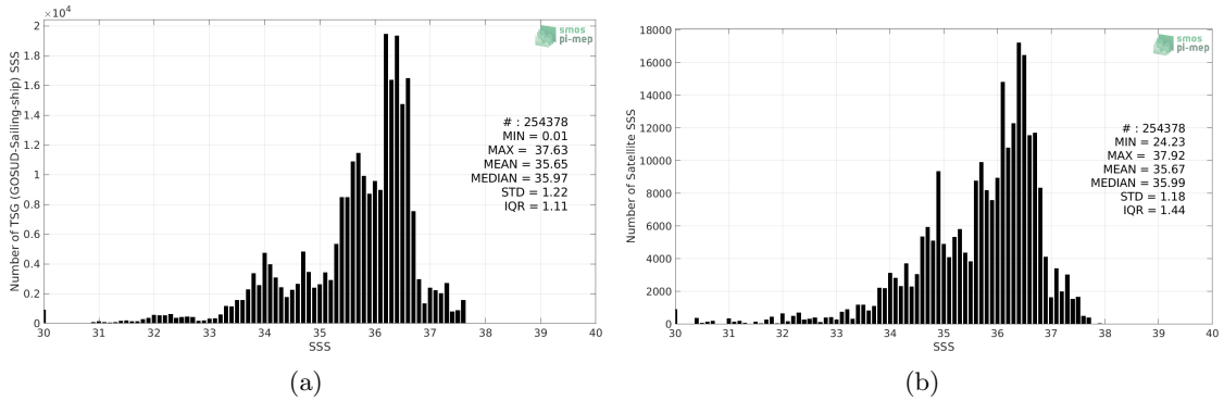
Figure 2: Histograms of SSS from TSG (GOSUD-Sailing-ship) (a) and SMOS L4 v2 Weekly (CATDS-CECOS-IFREMER) (b) considering all match-up pairs per bins of 0.1 over the Atlantic Ocean Pi-MEP region and for the full satellite product period.
