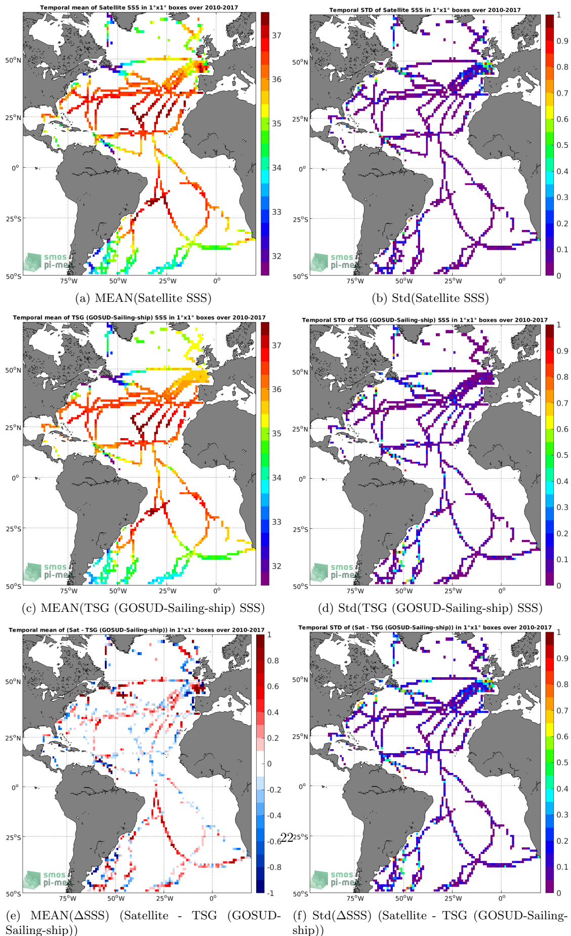
Figure 6: Temporal mean (left) and Std (right) of SSS from SMOS L4 v2 Weekly (CATDS-CECOS-IFREMER) (top), TSG (GOSUD-Sailing-ship) (middle), and of \Delta SSS (Satellite - TSG (GOSUD-Sailing-ship)). Only match-up pairs are used to generate these maps.
