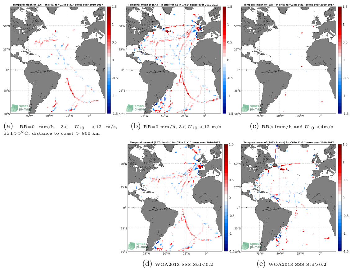
Figure 12: Temporal mean gridded over spatial boxes of size 1^\circ \times 1^\circ of \Delta SSS (SMOS L4 v2 Weekly (CATDS-CECOS-IFREMER) - TSG (GOSUD-Sailing-ship)) for 5 different subdatasets corresponding to:RR=0 mm/h, 3 < U_{10} < 12 m/s, SST>5°C, distance to coast > 800 km (a), RR=0 mm/h, 3 < U_{10} < 12 m/s (b), RR>1mm/h and U_{10} < 4 m/s (c), WOA2013 SSS Std<0.2 (d), WOA2013 SSS Std>0.2 (e).
