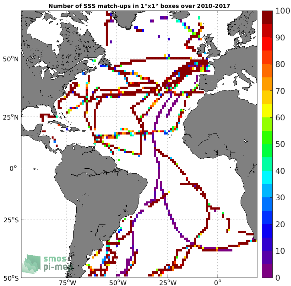
Figure 4: Number of SSS match-ups between TSG (GOSUD-Sailing-ship) SSS and the SMOS L4 v2 Weekly (CATDS-CECOS-IFREMER) SSS product for the Atlantic Ocean Pi-MEP region over 1°x1° boxes and for the full satellite product period.
