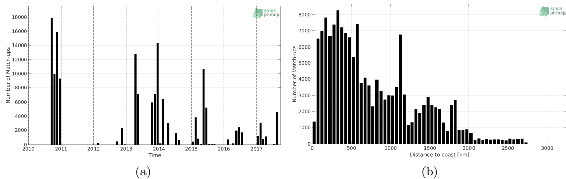
Figure 1: Number of match-ups between TSG-GOSUD-Sailing-ship and SMOS-L4-CATDS-CECOS-IFREMER-V2-WEEKLY-0.5DEG SSS as a function of time (a) and as function of the distance to coast (b) over the Atlantic Ocean Pi-MEP region and for the full satellite product period.
