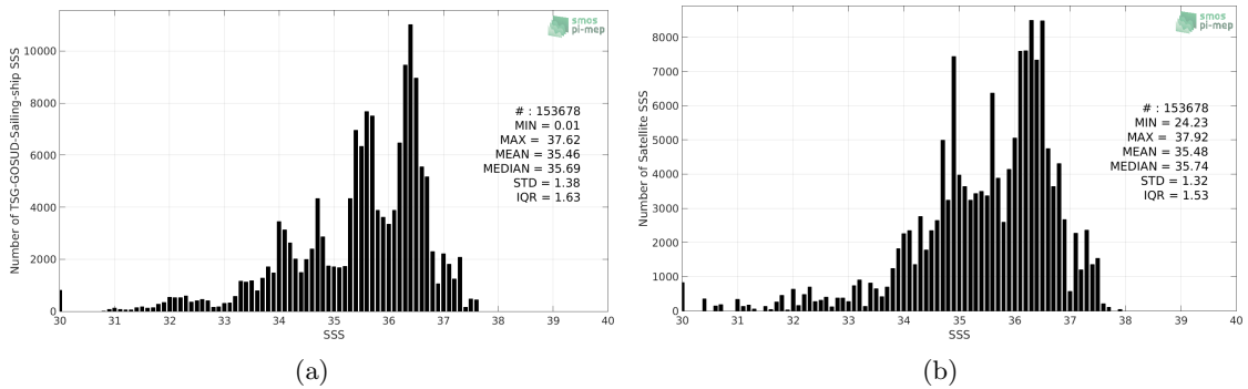
Figure 2: Histograms of SSS from TSG-GOSUD-Sailing-ship (a) and SMOS-L4-CATDS-CECOS-IFREMER-V2-WEEKLY-0.5DEG (b) considering all match-up pairs per bins of 0.1 over the Atlantic Ocean Pi-MEP region and for the full satellite product period.
