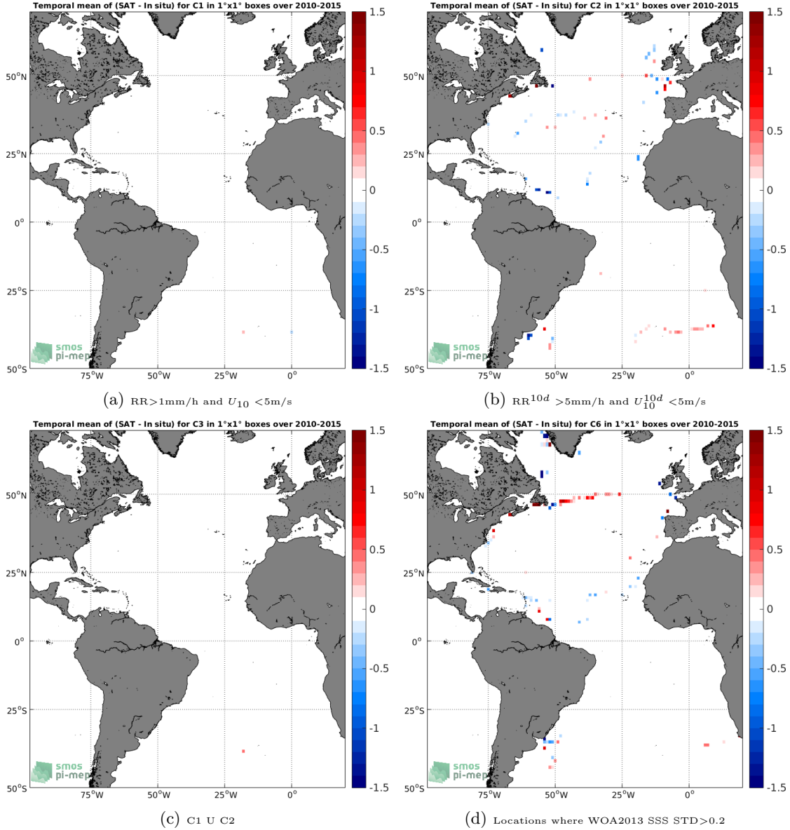
Figure 12: Temporal mean gridded over spatial boxes of size 1^\circ \times 1^\circ of \Delta SSS (SMOS-L4-CATDS-CECOS-IFREMER-V2-WEEKLY-0.5DEG - TSG-GOSUD-Sailing-ship) for 4 different subdatasets corresponding to: RR > 1\text{mm/h} and U_{10} < 5\text{m/s} (a), RR^{10d} > 5\text{mm/h} and U_{10}^{10d} < 5\text{m/s} (b), C1 U C2 (c), Locations where WOA2013 SSS STD > 0.2 (d).
