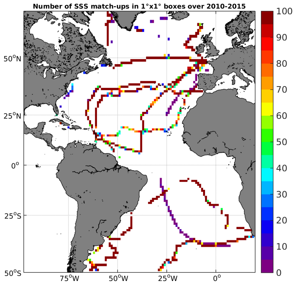
Figure 4: Number of SSS match-ups between TSG-GOSUD-Sailing-ship SSS and the SMOS-L4-CATDS-CECOS-IFREMER-V2-WEEKLY-0.5DEG SSS product for the Atlantic Ocean Pi-MEP region over 1°x1° boxes and for the full satellite product period.
