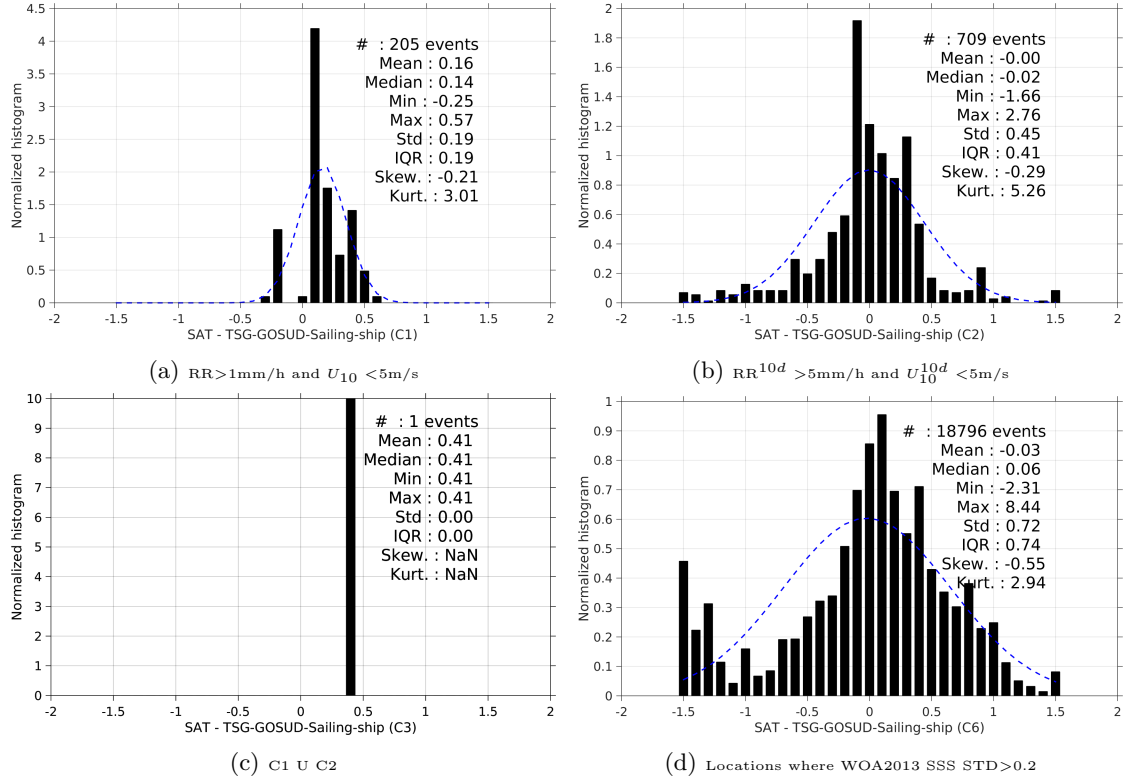
Figure 13: Normalized histogram of \Delta SSS (SMOS-L4-CATDS-CECOS-IFREMER-V2-WEEKLY-0.5DEG - TSG-GOSUD-Sailing-ship) for 6 different subdatasets corresponding to: RR > 1\text{mm/h} and U_{10} < 5\text{m/s} (a), RR^{10d} > 5\text{mm/h} and U_{10}^{10d} < 5\text{m/s} (b), C1 \cup C2 (c), Locations where WOA2013 SSS STD > 0.2 (d).
