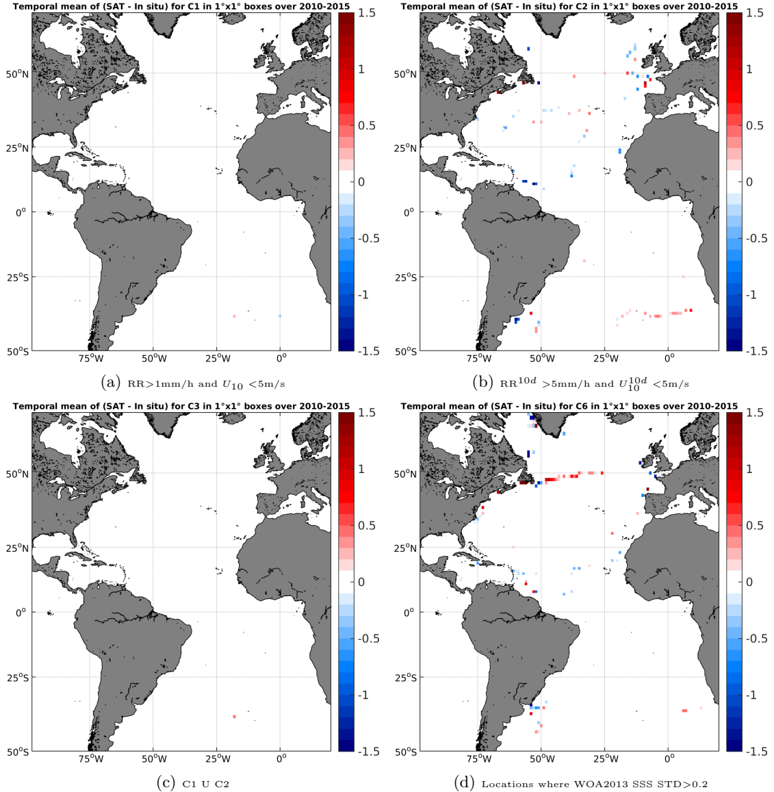
Figure 12: Temporal mean gridded over spatial boxes of size 1°x1° of \Delta SSS (SMOS-L4-CATDS-CECOS-IFREMER-V2-WEEKLY-0.5DEG - TSG-GOSUD-Sailing-ship) for 4 different subdatasets corresponding to:RR>1mm/h and U_{10} < 5\text{m/s} (a), RR^{10d} > 5\text{mm/h} and U_{10}^{10d} < 5\text{m/s} (b), C1 U C2 (c),Locations where WOA2013 SSS STD>0.2 (d).
