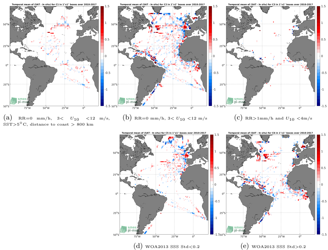
Figure 12: Temporal mean gridded over spatial boxes of size 1^\circ \times 1^\circ of \Delta SSS (SMOS L4 v2 Weekly (CATDS-CECOS-IFREMER) - TSG (GOSUD-Research-vessel)) for 5 different subdatasets corresponding to:RR=0 mm/h, 3 < U_{10} < 12 m/s, SST>5°C, distance to coast > 800 km (a), RR=0 mm/h, 3 < U_{10} < 12 m/s (b), RR>1mm/h and U_{10} < 4 m/s (c), WOA2013 SSS Std<0.2 (d), WOA2013 SSS Std>0.2 (e).
