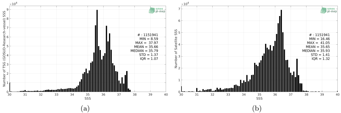
Figure 2: Histograms of SSS from TSG (GOSUD-Research-vessel) (a) and SMOS L4 v2 Weekly (CATDS-CECOS-IFREMER) (b) considering all match-up pairs per bins of 0.1 over the Atlantic Ocean Pi-MEP region and for the full satellite product period.
