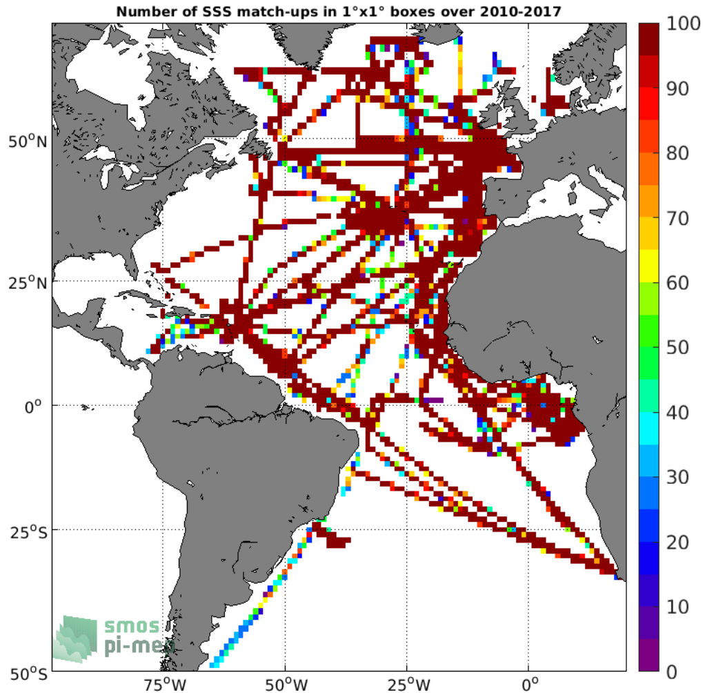
Figure 4: Number of SSS match-ups between TSG (GOSUD-Research-vessel) SSS and the SMOS L4 v2 Weekly (CATDS-CECOS-IFREMER) SSS product for the Atlantic Ocean Pi-MEP region over 1^\circ \times 1^\circ boxes and for the full satellite product period.
