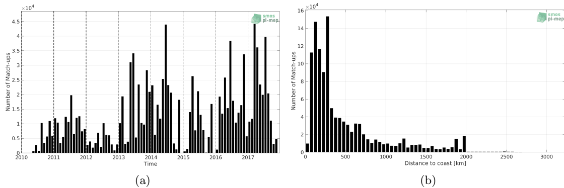
Figure 1: Number of match-ups between TSG (GOSUD-Research-vessel) and SMOS L4 v2 Weekly (CATDS-CECOS-IFREMER) SSS as a function of time (a) and as function of the distance to coast (b) over the Atlantic Ocean Pi-MEP region and for the full satellite product period.
