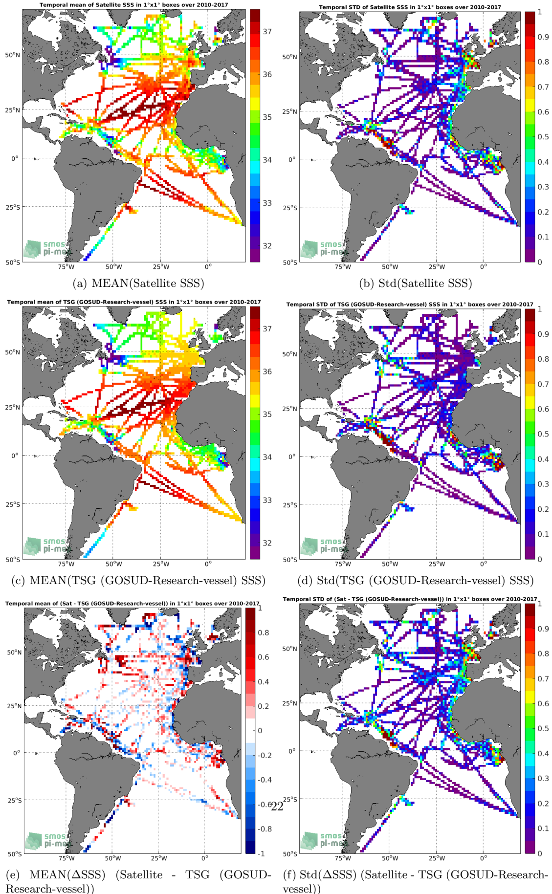
Figure 6: Temporal mean (left) and Std (right) of SSS from SMOS L4 v2 Weekly (CATDS-CECOS-IFREMER) (top), TSG (GOSUD-Research-vessel) (middle), and of \Delta SSS (Satellite - TSG (GOSUD-Research-vessel)). Only match-up pairs are used to generate these maps.
