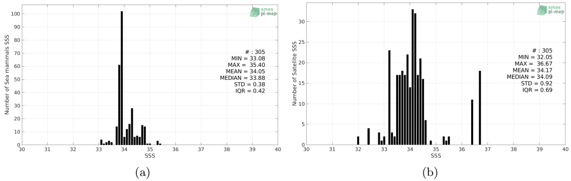
Figure 2: Histograms of SSS from Sea mammals (a) and SMOS L4 v2 Weekly (CATDS-CECOS-IFREMER) (b) considering all match-up pairs per bins of 0.1 over the Atlantic Ocean Pi-MEP region and for the full satellite product period.
