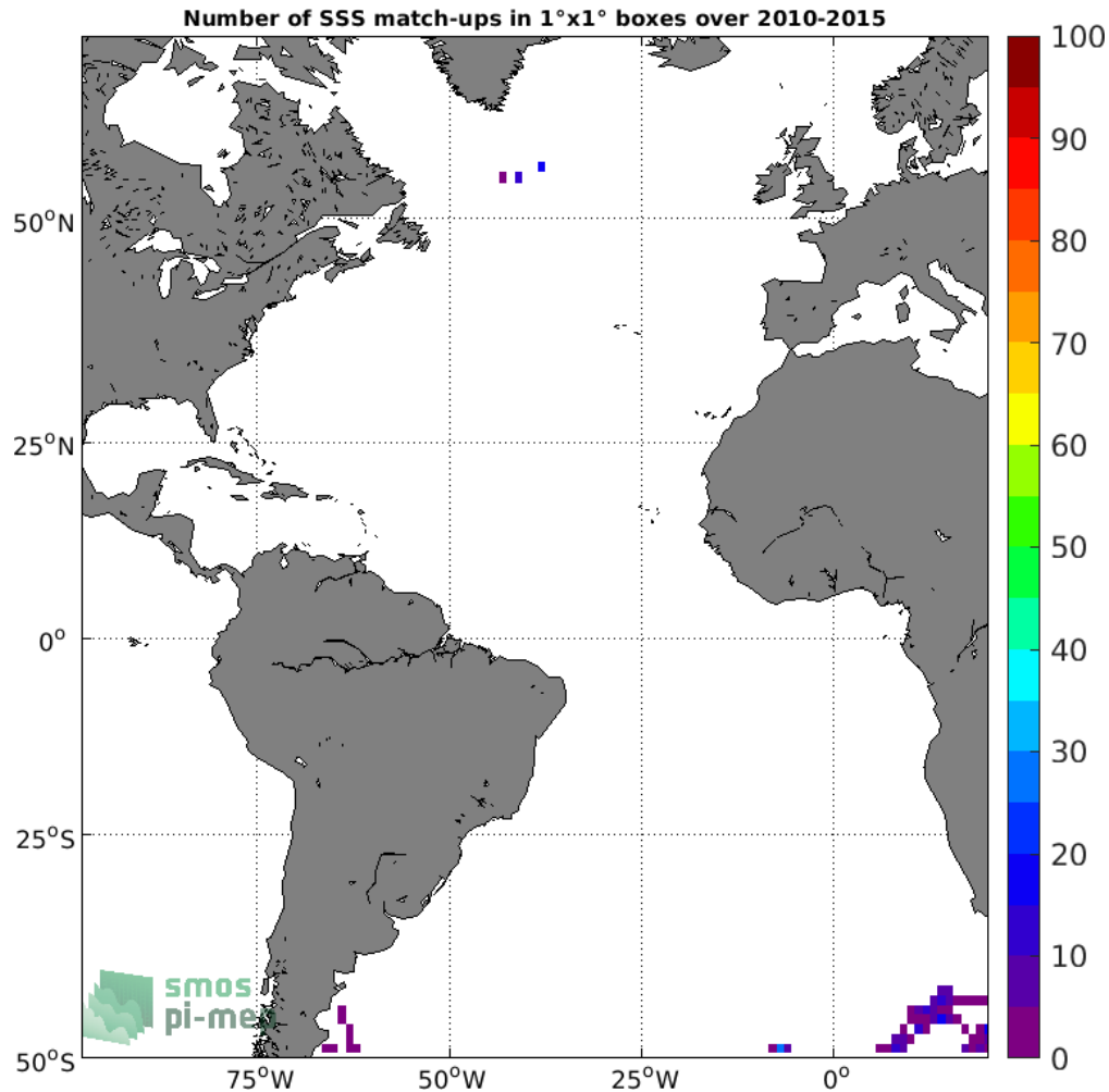
Figure 4: Number of SSS match-ups between Sea mammals SSS and the SMOS L4 v2 Weekly (CATDS-CECOS-IFREMER) SSS product for the Atlantic Ocean Pi-MEP region over 1^\circ \times 1^\circ boxes and for the full satellite product period.
