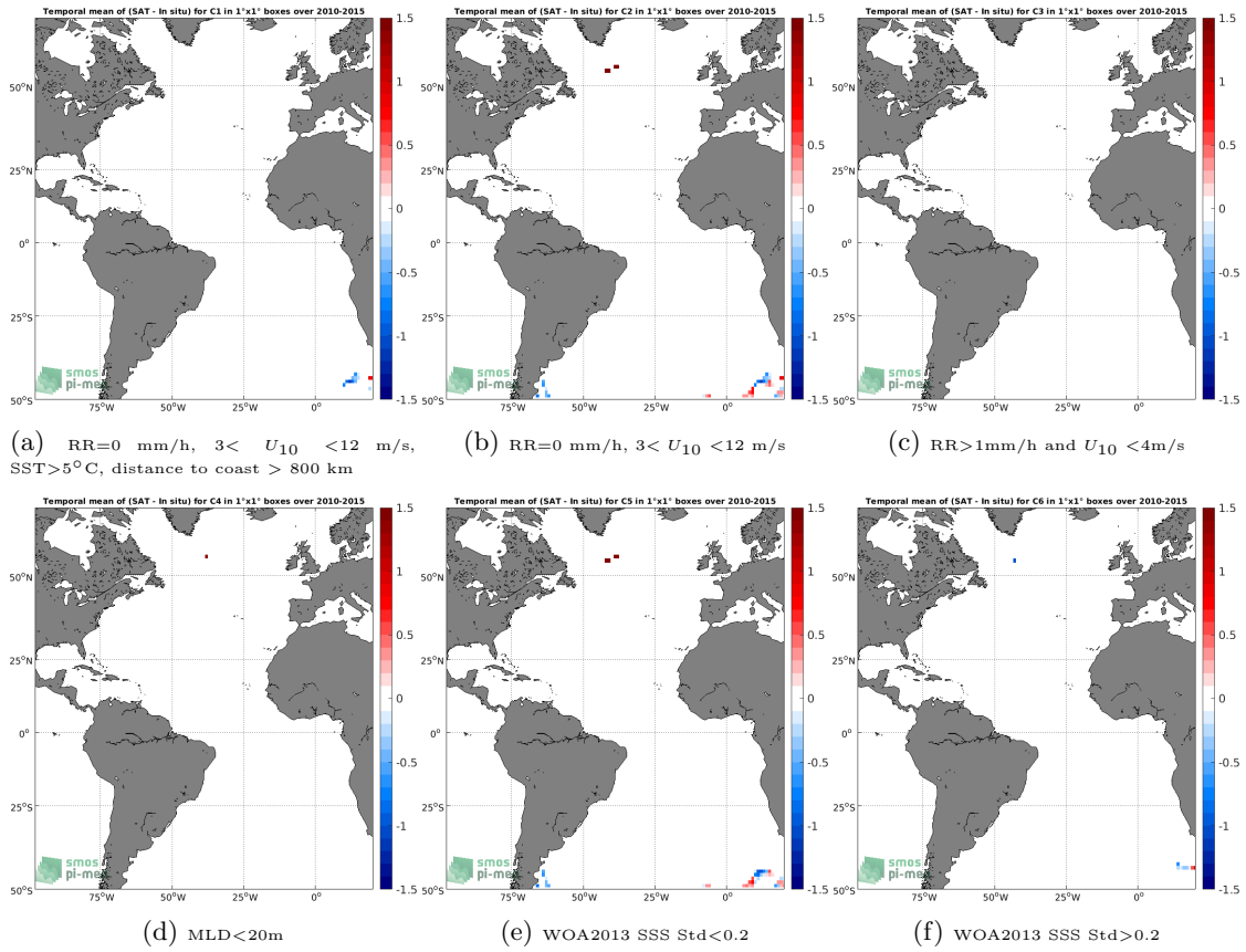
Figure 12: Temporal mean gridded over spatial boxes of size 1^\circ \times 1^\circ of \Delta SSS (SMOS L4 v2 Weekly (CATDS-CECOS-IFREMER) - Sea mammals) for 6 different subdatasets corresponding to:RR=0 mm/h, 3 < U_{10} < 12 m/s, SST>5°C, distance to coast > 800 km (a), RR=0 mm/h, 3 < U_{10} < 12 m/s (b), RR>1mm/h and U_{10} < 4 m/s (c),MLD<20m (d),WOA2013 SSS Std<0.2 (e),WOA2013 SSS Std>0.2 (f).
