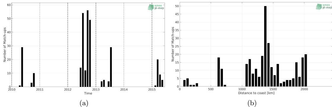
Figure 1: Number of match-ups between Sea mammals and SMOS L4 v2 Weekly (CATDS-CECOS-IFREMER) SSS as a function of time (a) and as function of the distance to coast (b) over the Atlantic Ocean Pi-MEP region and for the full satellite product period.
