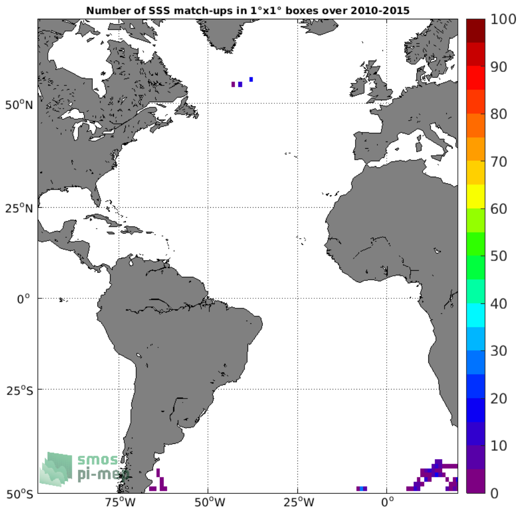
Figure 4: Number of SSS match-ups between Sea mammals SSS and the SMOS L4 v2 Weekly (CATDS-CECOS-IFREMER) SSS product for the Atlantic Ocean Pi-MEP region over 1°x1° boxes and for the full satellite product period.
