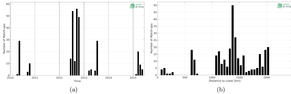
Figure 1: Number of match-ups between Sea mammals and SMOS L4 v2 Weekly (CATDS-CECOS-IFREMER) SSS as a function of time (a) and as function of the distance to coast (b) over the Atlantic Ocean Pi-MEP region and for the full satellite product period.
