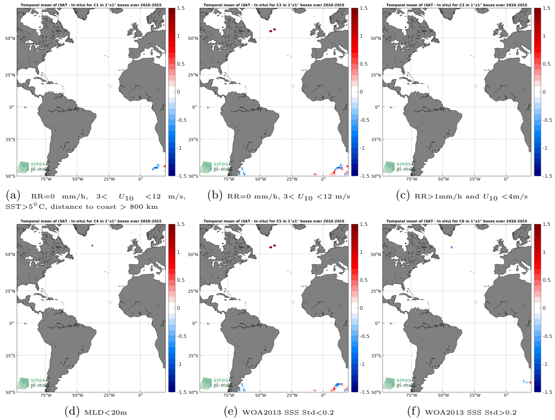
Figure 12: Temporal mean gridded over spatial boxes of size 1^\circ \times 1^\circ of \Delta SSS (SMOS L4 v2 Weekly (CATDS-CECOS-IFREMER) - Sea mammals) for 6 different subdatasets corresponding to: RR=0 mm/h, 3 < U_{10} < 12 m/s, SST>5°C, distance to coast > 800 km (a), RR=0 mm/h, 3 < U_{10} < 12 m/s (b), RR>1mm/h and U_{10} < 4 m/s (c),MLD<20m (d),WOA2013 SSS Std<0.2 (e),WOA2013 SSS Std>0.2 (f).
