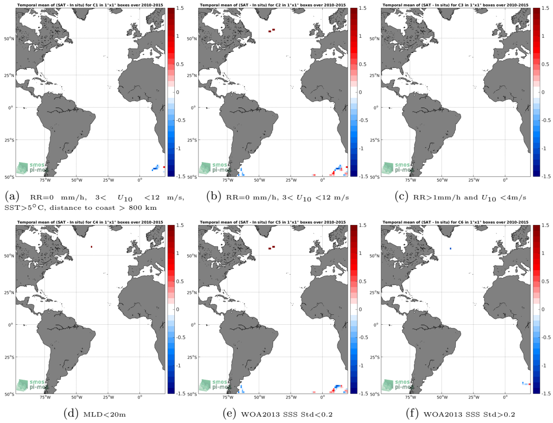
Figure 12: Temporal mean gridded over spatial boxes of size 1^\circ \times 1^\circ of \Delta SSS (SMOS-L4-CATDS-CECOS-IFREMER-V2-WEEKLY-0.5DEG - Sea mammals) for 6 different subdatasets corresponding to:RR=0 mm/h, 3 < U_{10} < 12 m/s, SST>5°C, distance to coast > 800 km (a), RR=0 mm/h, 3 < U_{10} < 12 m/s (b), RR>1mm/h and U_{10} < 4 m/s (c),MLD<20m (d),WOA2013 SSS Std<0.2 (e),WOA2013 SSS Std>0.2 (f).
