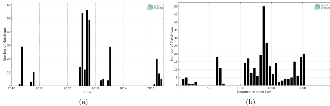
Figure 1: Number of match-ups between Sea mammals and SMOS-L4-CATDS-CECOS-IFREMER-V2-WEEKLY-0.5DEG SSS as a function of time (a) and as function of the distance to coast (b) over the Atlantic Ocean Pi-MEP region and for the full satellite product period.
