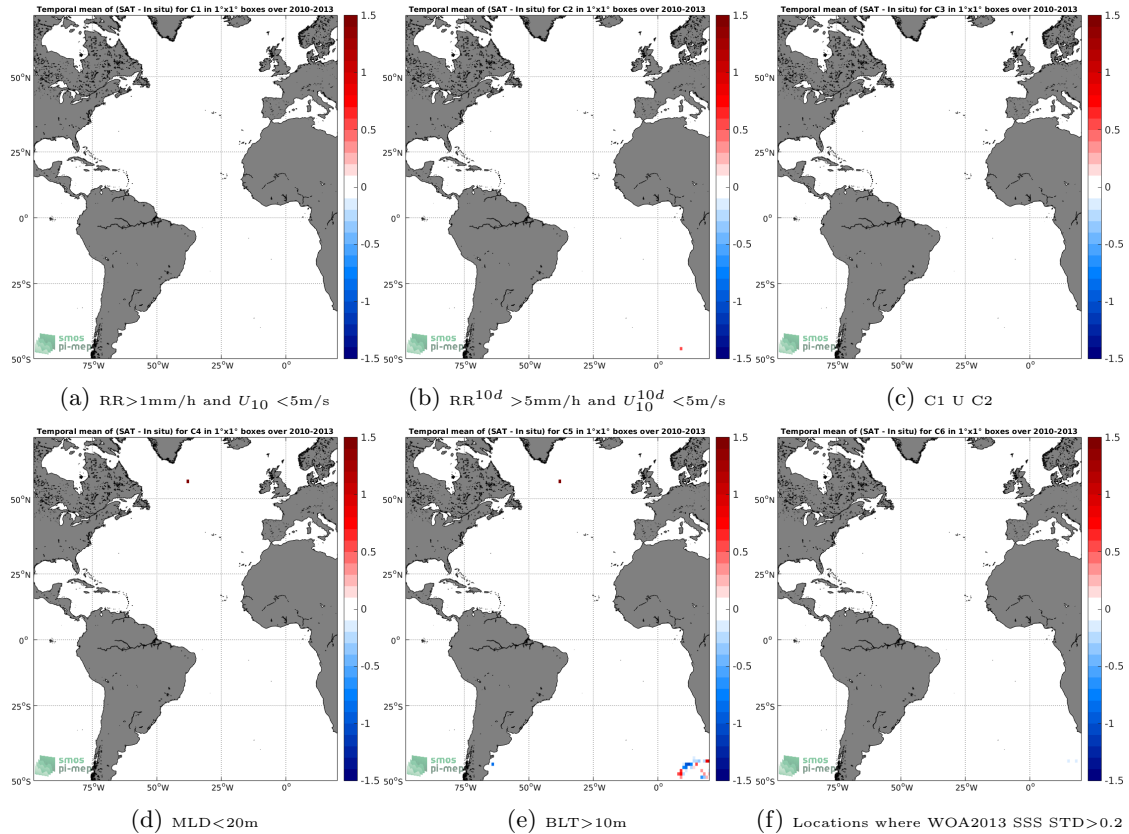
Figure 12: Temporal mean gridded over spatial boxes of size 1^\circ \times 1^\circ of \Delta\text{SSS} (SMOS-L4-CATDS-CECOS-IFREMER-V2-WEEKLY-0.5DEG - Sea mammals) for 6 different subdatasets corresponding to: \text{RR} > 1\text{mm/h} and U_{10} < 5\text{m/s} (a), \text{RR}^{10d} > 5\text{mm/h} and U_{10}^{10d} < 5\text{m/s} (b), C1 U C2 (c), \text{MLD} < 20\text{m} (d), \text{BLT} > 10\text{m} (e), Locations where WOA2013 SSS STD > 0.2 (f).
