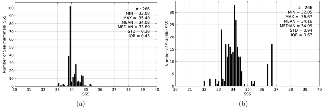
Figure 2: Histograms of SSS from Sea mammals (a) and SMOS-L4-CATDS-CECOS-IFREMER-V2-WEEKLY-0.5DEG (b) considering all match-up pairs per bins of 0.1 over the Atlantic Ocean Pi-MEP region and for the full satellite product period.
