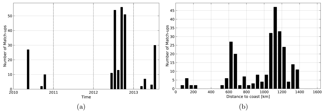
Figure 1: Number of match-ups between Sea mammals and SMOS-L4-CATDS-CECOS-IFREMER-V2-WEEKLY-0.5DEG SSS as a function of time (a) and as function of the distance to coast (b) over the Atlantic Ocean Pi-MEP region and for the full satellite product period.
