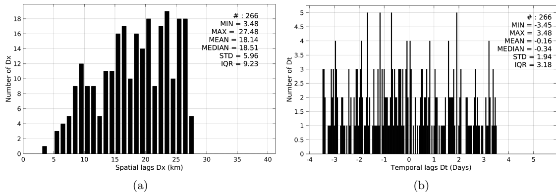
Figure 5: Histograms of the spatial (a) and temporal (b) lags between the time of the Sea mammals measurements and the date of the corresponding SMOS-L4-CATDS-CECOS-IFREMER-V2-WEEKLY-0.5DEG SSS product.
