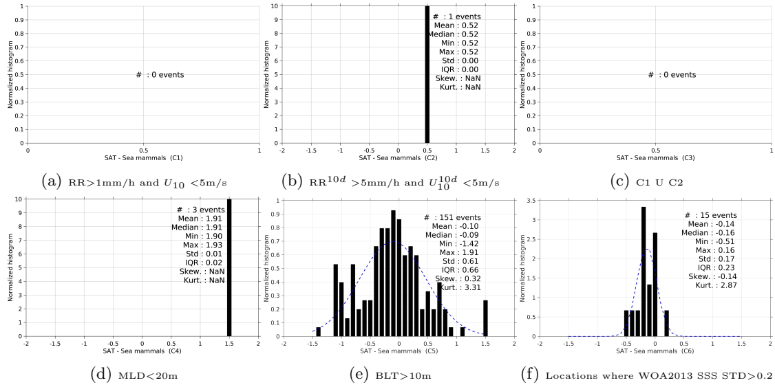
Figure 13: Normalized histogram of \Delta SSS (SMOS-L4-CATDS-CECOS-IFREMER-V2-WEEKLY-0.5DEG - Sea mammals) for 6 different subdatasets corresponding to: RR > 1\text{mm/h} and U_{10} < 5\text{m/s} (a), RR^{10d} > 5\text{mm/h} and U_{10}^{10d} < 5\text{m/s} (b), C1 \cup C2 (c), MLD < 20\text{m} (d), BLT > 10\text{m} (e), Locations where WOA2013 SSS STD > 0.2 (f).
