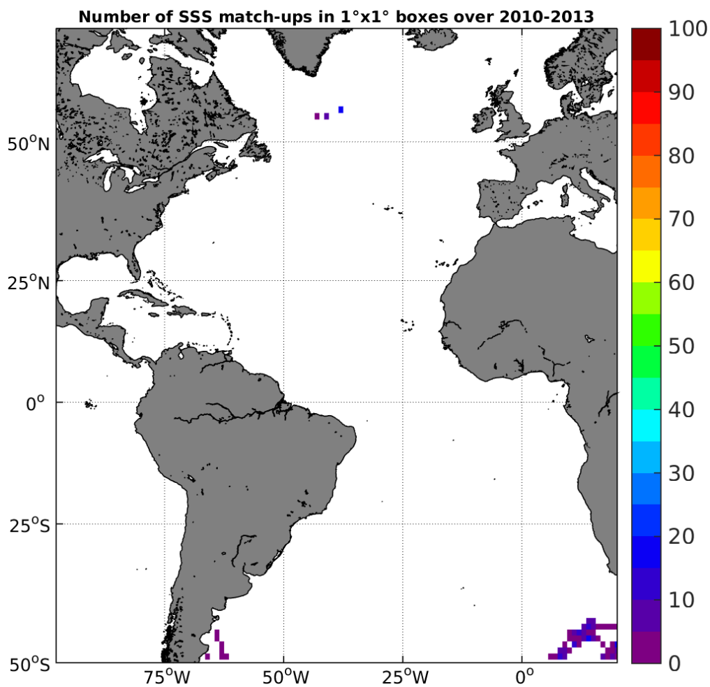
Figure 4: Number of SSS match-ups between Sea mammals SSS and the SMOS-L4-CATDS-CECOS-IFREMER-V2-WEEKLY-0.5DEG SSS product for the Atlantic Ocean Pi-MEP region over 1°x1° boxes and for the full satellite product period.
