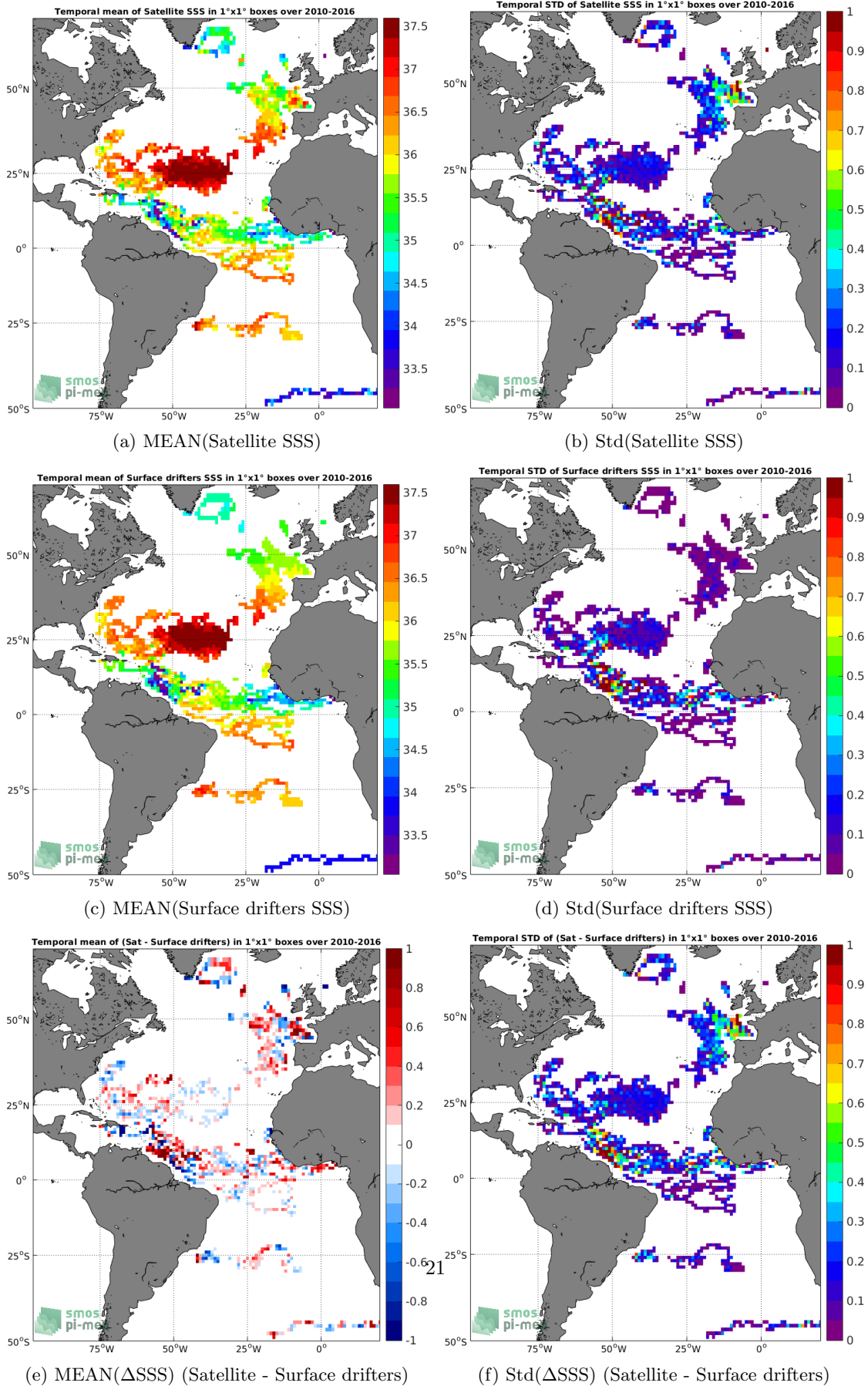
(e) MEAN( \Delta SSS) (Satellite - Surface drifters) (f) Std( \Delta SSS) (Satellite - Surface drifters) Figure 5: Temporal mean (left) and Std (right) of SSS from SMOS-L4-CATDS-CECOS-IFREMER-V2-WEEKLY-0.5DEG (top), Surface drifters (middle), and of \Delta SSS (Satellite - Surface drifters). Only match-up pairs are used to generate these maps.
