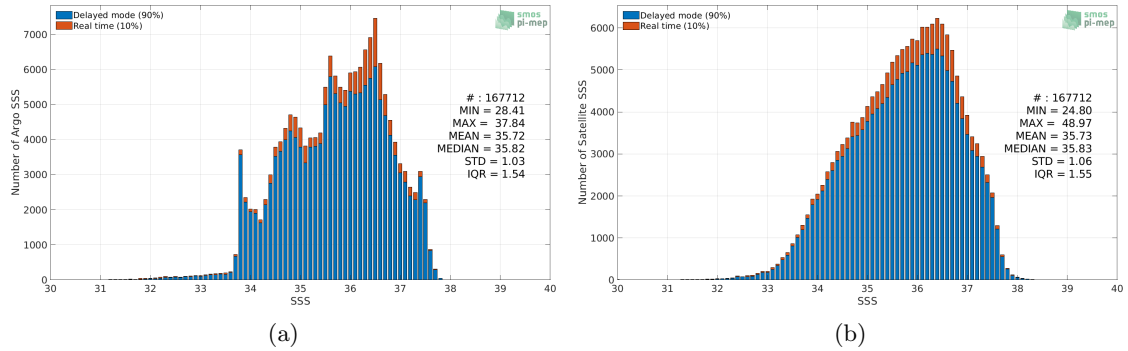
Figure 2: Histograms of SSS from Argo (a) and SMOS L4 v2 Weekly (CATDS-CECOS-IFREMER) (b) considering all match-up pairs per bins of 0.1 over the Atlantic Ocean Pi-MEP region and for the full satellite product period.
