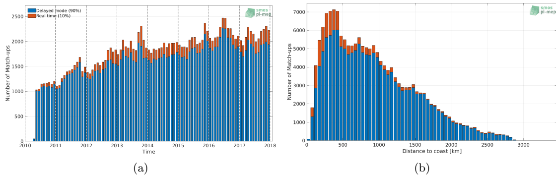
Figure 1: Number of match-ups between Argo and SMOS L4 v2 Weekly (CATDS-CECOS-IFREMER) SSS as a function of time (a) and as function of the distance to coast (b) over the Atlantic Ocean Pi-MEP region and for the full satellite product period.
