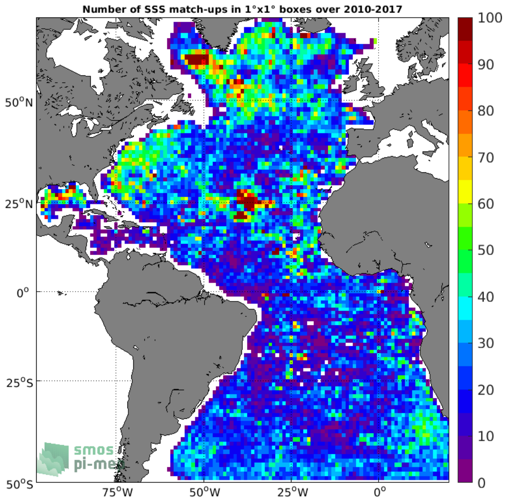
Figure 4: Number of SSS match-ups between Argo SSS and the SMOS L4 v2 Weekly (CATDS-CECOS-IFREMER) SSS product for the Atlantic Ocean Pi-MEP region over 1°x1° boxes and for the full satellite product period.
