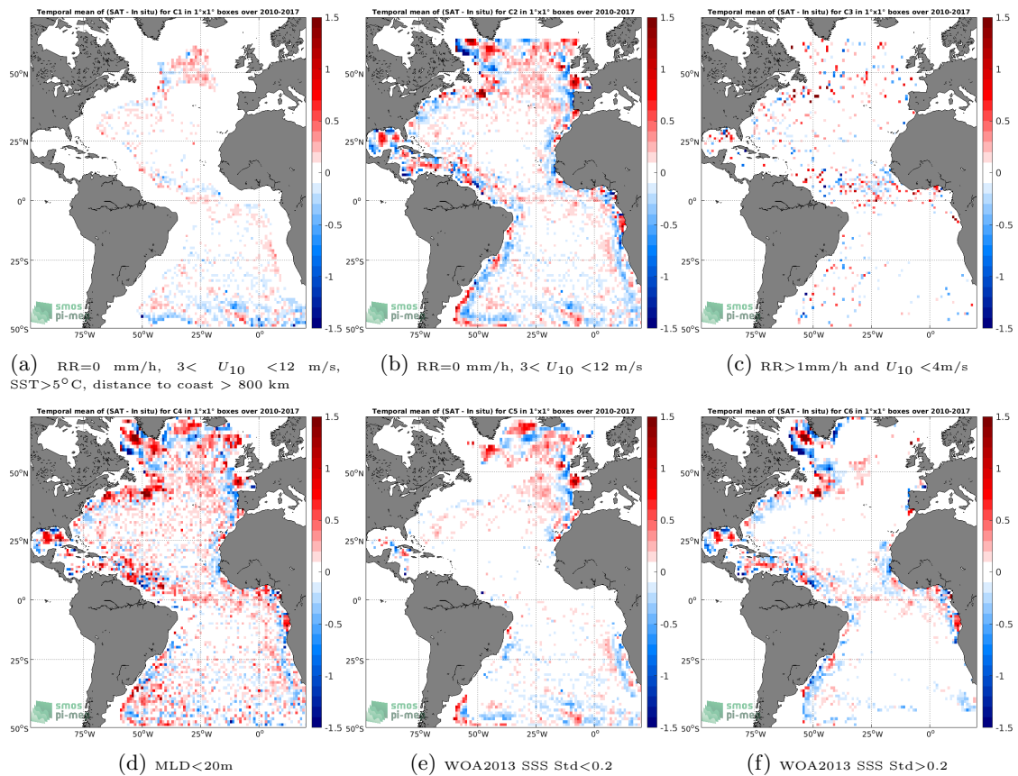
Figure 12: Temporal mean gridded over spatial boxes of size 1^\circ \times 1^\circ of \Delta SSS (SMOS L4 v2 Weekly (CATDS-CECOS-IFREMER) - Argo) for 6 different subdatasets corresponding to:RR=0 mm/h, 3 < U_{10} < 12 m/s, SST > 5^\circ\text{C} , distance to coast > 800 km (a), RR=0 mm/h, 3 < U_{10} < 12 m/s (b), RR > 1 mm/h and U_{10} < 4 m/s (c),MLD < 20 m (d),WOA2013 SSS Std < 0.2 (e),WOA2013 SSS Std > 0.2 (f).
