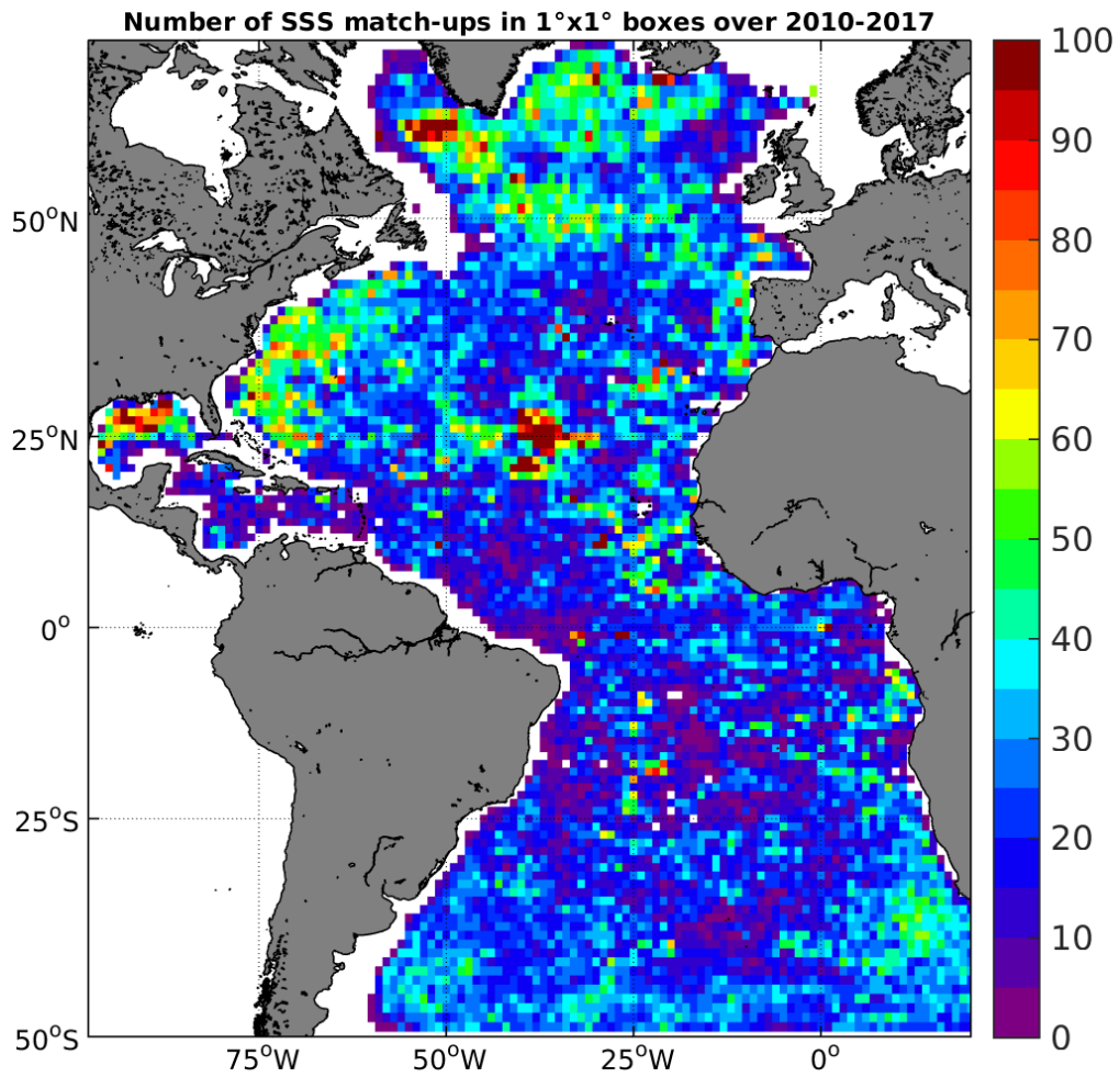
Figure 4: Number of SSS match-ups between Argo SSS and the SMOS-L4-CATDS-CECOS-IFREMER-V2-WEEKLY-0.5DEG SSS product for the Atlantic Ocean Pi-MEP region over 1°x1° boxes and for the full satellite product period.
