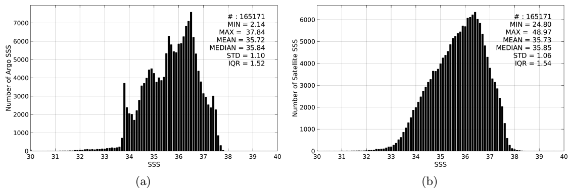
Figure 2: Histograms of SSS from Argo (a) and SMOS-L4-CATDS-CECOS-IFREMER-V2-WEEKLY-0.5DEG (b) considering all match-up pairs per bins of 0.1 over the Atlantic Ocean Pi-MEP region and for the full satellite product period.
