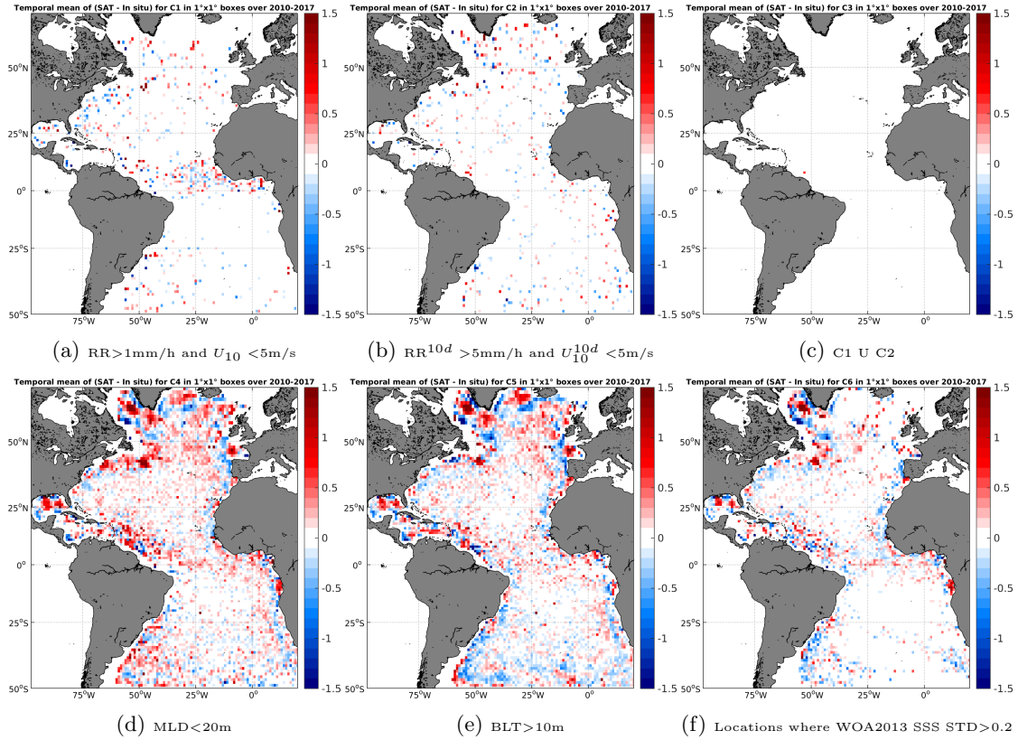
Figure 12: Temporal mean gridded over spatial boxes of size 1^\circ \times 1^\circ of \Delta SSS (SMOS-L4-CATDS-CECOS-IFREMER-V2-WEEKLY-0.5DEG - Argo) for 6 different subdatasets corresponding to:RR>1mm/h and U_{10} < 5 m/s (a), RR^{10d} > 5 mm/h and U_{10}^{10d} < 5 m/s (b), C1 U C2 (c),MLD<20m (d),BLT>10m (e),Locations where WOA2013 SSS STD>0.2 (f).
