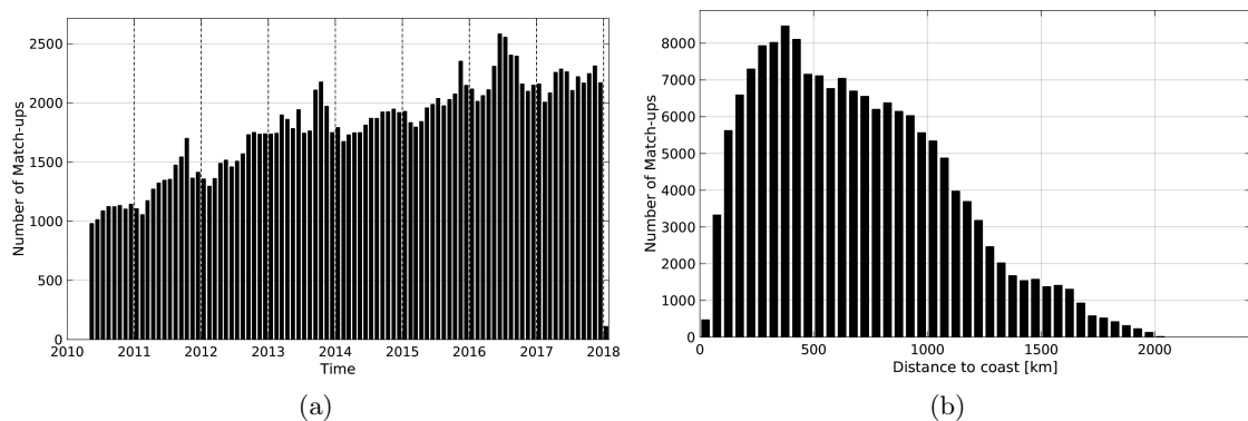
Figure 1: Number of match-ups between Argo and SMOS-L4-CATDS-CECOS-IFREMER-V2-WEEKLY-0.5DEG SSS as a function of time (a) and as function of the distance to coast (b) over the Atlantic Ocean Pi-MEP region and for the full satellite product period.
