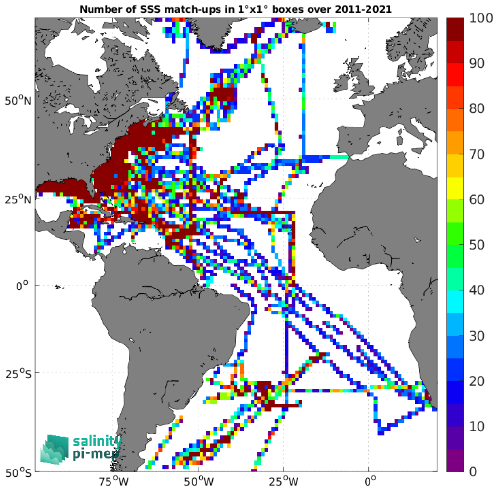
Figure 5: Number of SSS match-ups between TSG (SAMOS) SSS and the SMOS SSS L4 v2 - Daily (BEC) SSS product for the Atlantic Ocean Pi-MEP region over 1^\circ \times 1^\circ boxes and for the full satellite product period.
