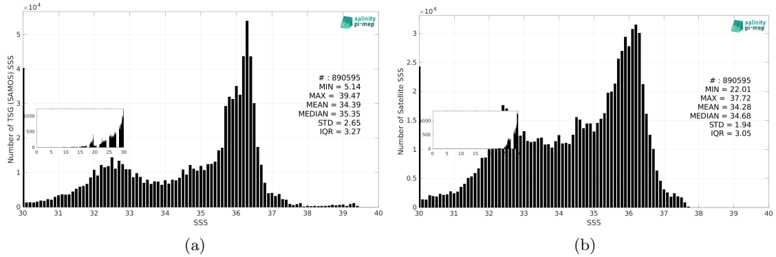
Figure 3: Histograms of SSS from TSG (SAMOS) (a) and SMOS SSS L4 v2 - Daily (BEC) (b) considering all match-up pairs per bins of 0.1 over the Atlantic Ocean Pi-MEP region and for the full satellite product period.
