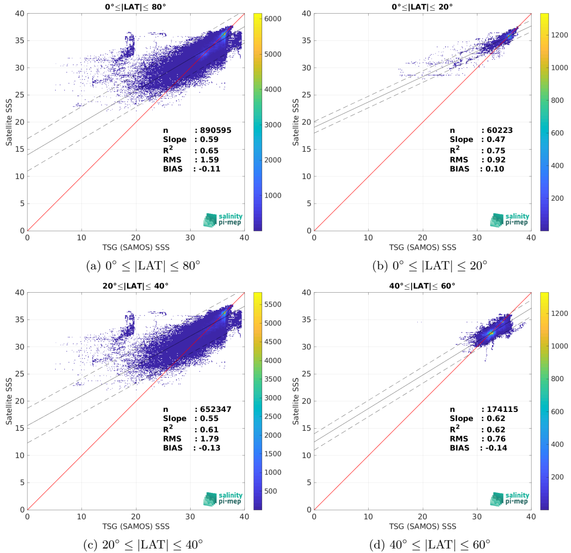
Figure 10: Contour maps of the concentration of SMOS SSS L4 v2 - Daily (BEC) SSS (y-axis) versus TSG (SAMOS) SSS (x-axis) at match-up pairs for different latitude bands. For each plot, the red line shows x=y . The black thin and dashed lines indicate a linear fit through the data cloud and the \pm 95\% confidence levels, respectively. The number match-up pairs n , the slope and R^2 coefficient of the linear fit, the root mean square (RMS) and the mean bias between satellite and in situ data are indicated for each latitude band in each plots.
