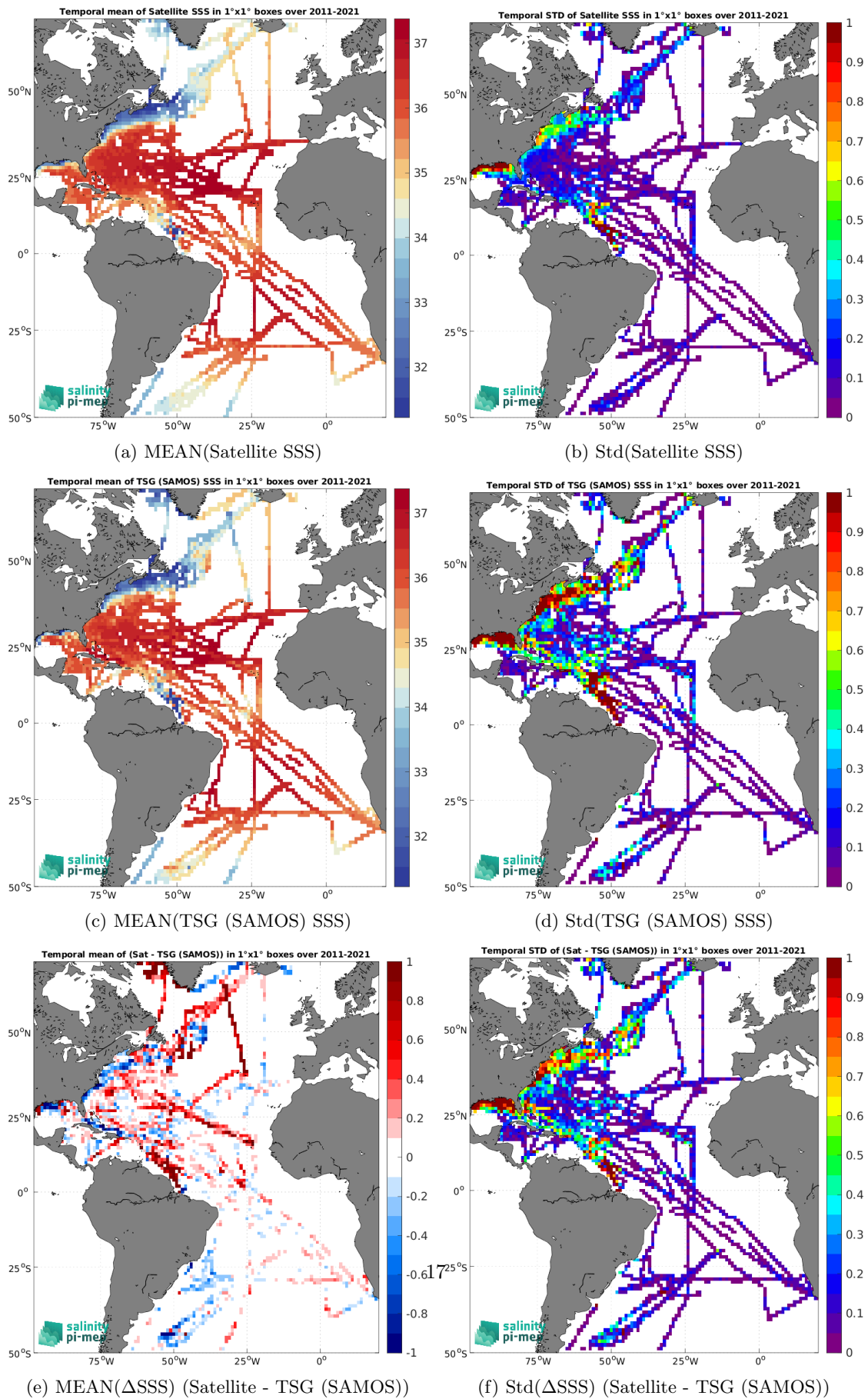
Figure 7: Temporal mean (left) and Std (right) of SSS from SMOS SSS L4 v2 - Daily (BEC) (top), TSG (SAMOS) (middle), and of \Delta SSS (Satellite - TSG (SAMOS)). Only match-up pairs are used to generate these maps.
