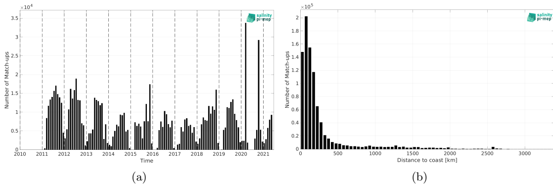
Figure 2: Number of match-ups between TSG (SAMOS) and SMOS SSS L4 v2 - Daily (BEC) SSS as a function of time (a) and as function of the distance to coast (b) over the Atlantic Ocean Pi-MEP region and for the full satellite product period.
