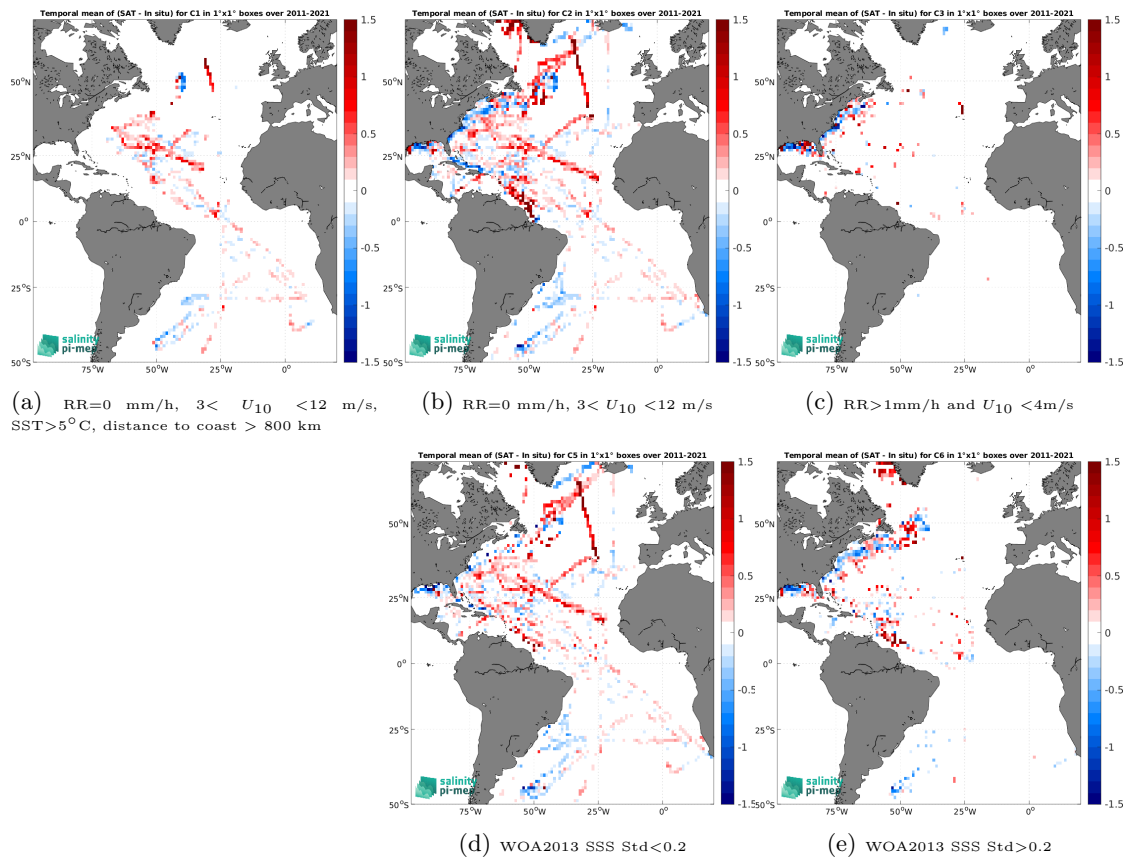
Figure 14: Temporal mean gridded over spatial boxes of size 1^\circ \times 1^\circ of \Delta\text{SSS} (SMOS SSS L4 v2 - Daily (BEC) - TSG (SAMOS)) for 5 different subdatasets corresponding to:RR=0 mm/h, 3 < U_{10} < 12 m/s, SST>5°C, distance to coast > 800 km (a), RR=0 mm/h, 3 < U_{10} < 12 m/s (b), RR>1mm/h and U_{10} < 4 m/s (c), WOA2013 SSS Std<0.2 (d), WOA2013 SSS Std>0.2 (e).
