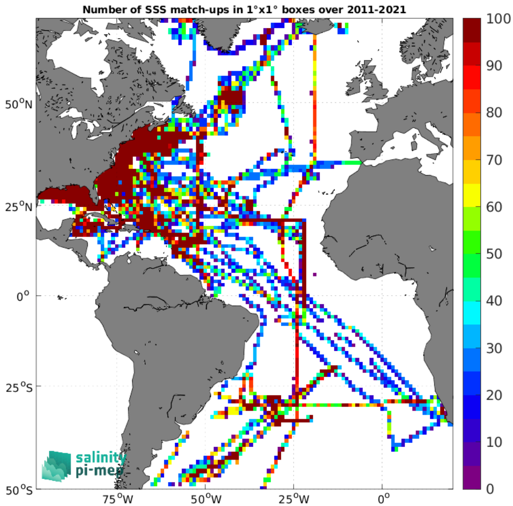
Figure 4: Number of SSS match-ups between TSG (SAMOS) SSS and the SMOS SSS L4 v2 - Daily (BEC) SSS product for the Atlantic Ocean Pi-MEP region over 1^\circ \times 1^\circ boxes and for the full satellite product period.
