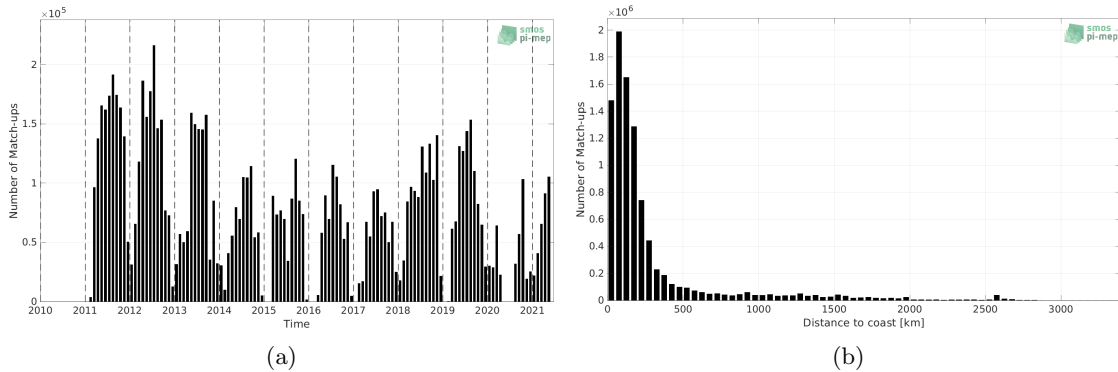
Figure 1: Number of match-ups between TSG (SAMOS) and SMOS SSS L4 v2 - Daily (BEC) SSS as a function of time (a) and as function of the distance to coast (b) over the Atlantic Ocean Pi-MEP region and for the full satellite product period.
