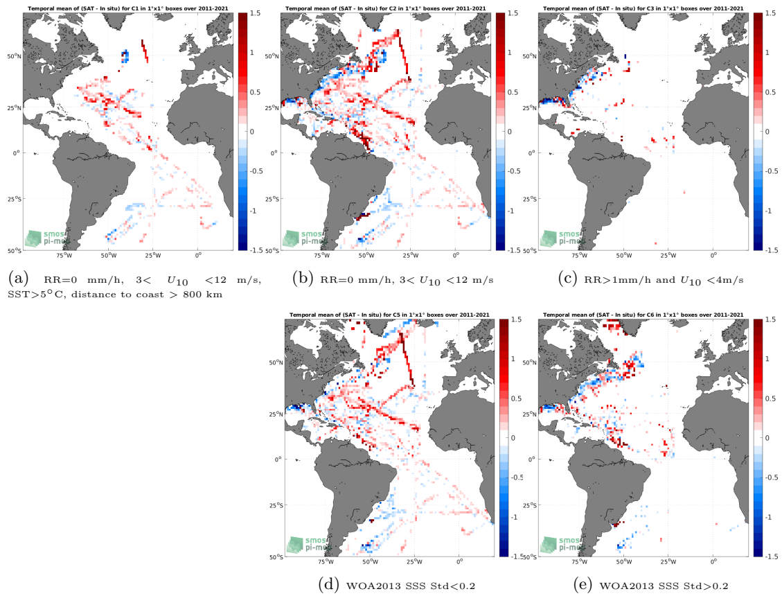
Figure 12: Temporal mean gridded over spatial boxes of size 1^\circ \times 1^\circ of \Delta SSS (SMOS SSS L4 v2 - Daily (BEC) - TSG (SAMOS)) for 5 different subdatasets corresponding to:RR=0 mm/h, 3 < U_{10} < 12 m/s, SST >5^\circ\text{C} , distance to coast > 800 km (a), RR=0 mm/h, 3 < U_{10} < 12 m/s (b), RR >1 mm/h and U_{10} < 4 m/s (c), WOA2013 SSS Std <0.2 (d), WOA2013 SSS Std >0.2 (e).
