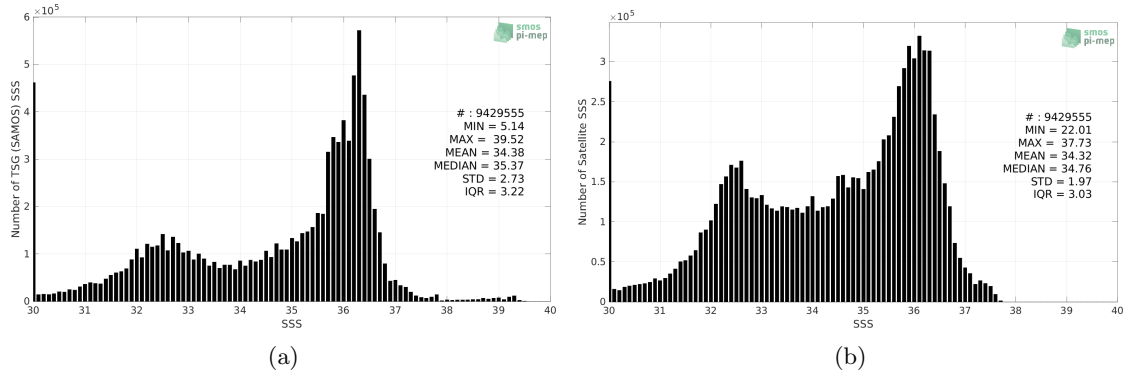
Figure 2: Histograms of SSS from TSG (SAMOS) (a) and SMOS SSS L4 v2 - Daily (BEC) (b) considering all match-up pairs per bins of 0.1 over the Atlantic Ocean Pi-MEP region and for the full satellite product period.
