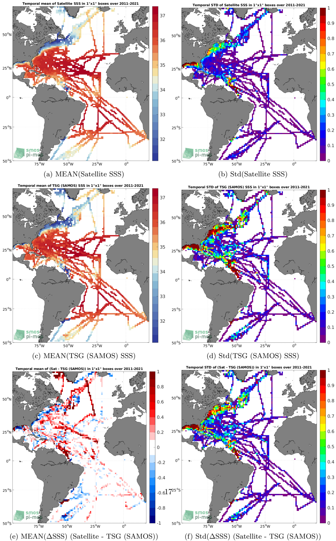
Figure 6: Temporal mean (left) and Std (right) of SSS from SMOS SSS L4 v2 - Daily (BEC) (top), TSG (SAMOS) (middle), and of \Delta SSS (Satellite - TSG (SAMOS)). Only match-up pairs are used to generate these maps.
