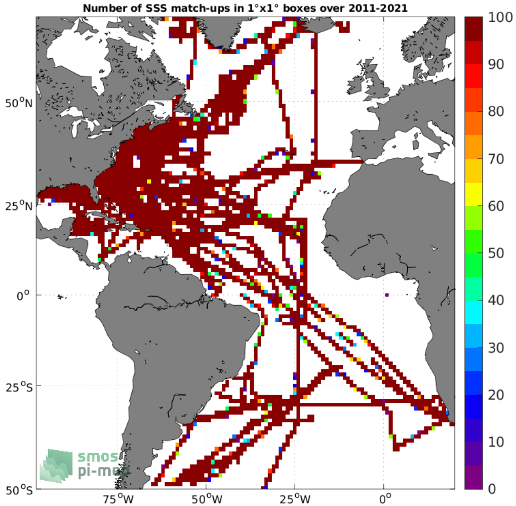
Figure 4: Number of SSS match-ups between TSG (SAMOS) SSS and the SMOS SSS L4 v2 - Daily (BEC) SSS product for the Atlantic Ocean Pi-MEP region over 1°×1° boxes and for the full satellite product period.
