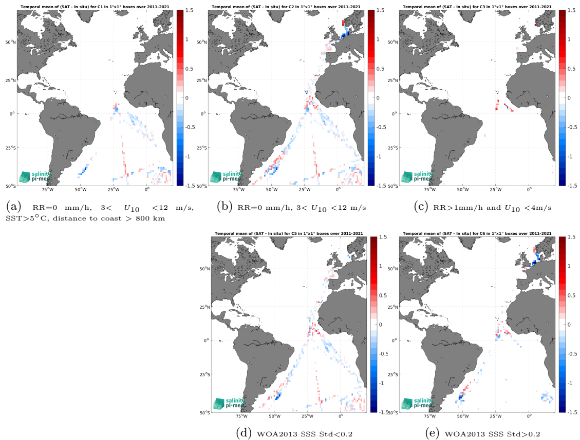
Figure 14: Temporal mean gridded over spatial boxes of size 1^\circ \times 1^\circ of \Delta\text{SSS} (SMOS SSS L4 v2 - Daily (BEC) - TSG (Polarstern)) for 5 different subdatasets corresponding to:RR=0 mm/h, 3 < U_{10} < 12 m/s, SST>5°C, distance to coast > 800 km (a), RR=0 mm/h, 3 < U_{10} < 12 m/s (b), RR>1mm/h and U_{10} < 4 m/s (c), WOA2013 SSS Std<0.2 (d), WOA2013 SSS Std>0.2 (e).
