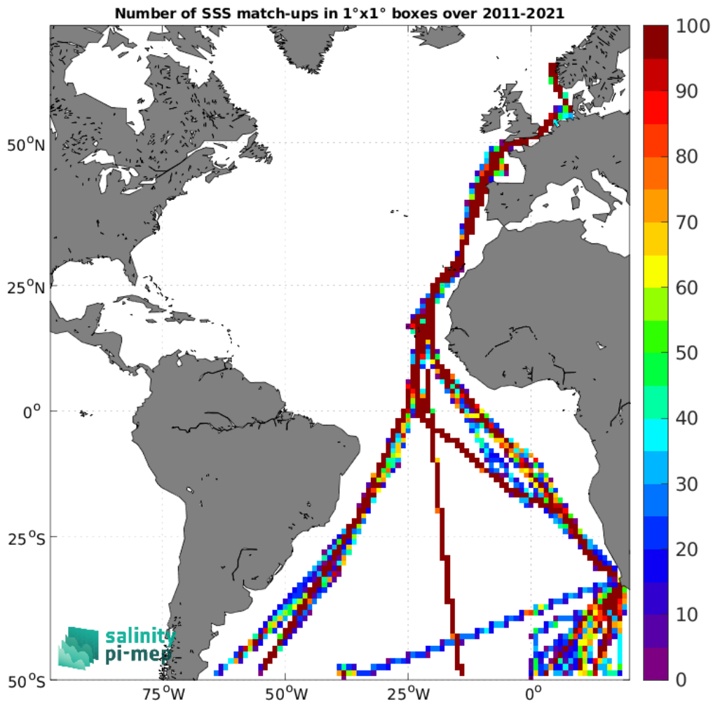
Figure 5: Number of SSS match-ups between TSG (Polarstern) SSS and the SMOS SSS L4 v2 - Daily (BEC) SSS product for the Atlantic Ocean Pi-MEP region over 1^\circ \times 1^\circ boxes and for the full satellite product period.
