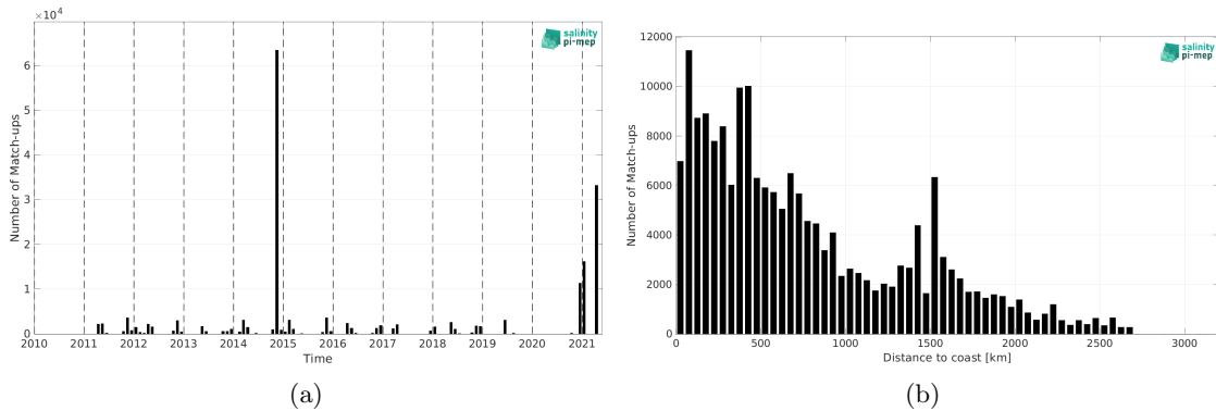
Figure 2: Number of match-ups between TSG (Polarstern) and SMOS SSS L4 v2 - Daily (BEC) SSS as a function of time (a) and as function of the distance to coast (b) over the Atlantic Ocean Pi-MEP region and for the full satellite product period.
