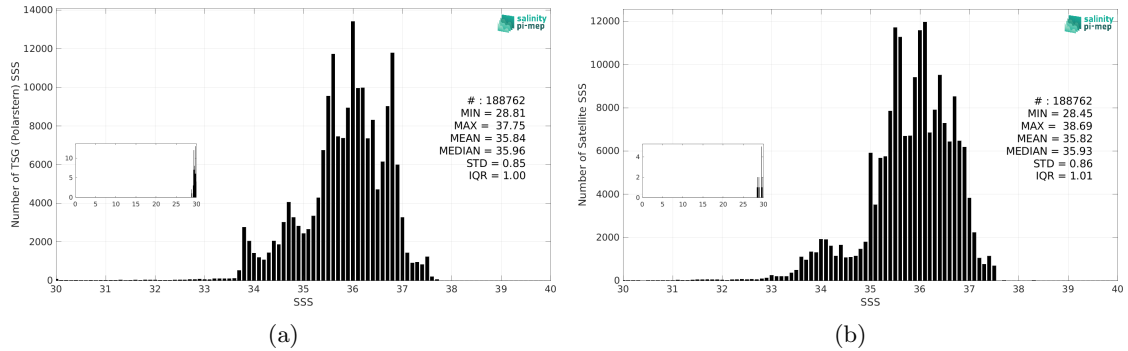
Figure 3: Histograms of SSS from TSG (Polarstern) (a) and SMOS SSS L4 v2 - Daily (BEC) (b) considering all match-up pairs per bins of 0.1 over the Atlantic Ocean Pi-MEP region and for the full satellite product period.
