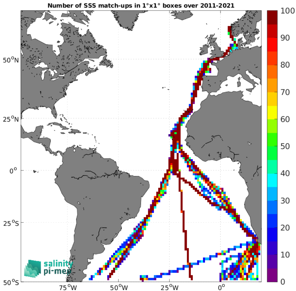
Figure 4: Number of SSS match-ups between TSG (Polarstern) SSS and the SMOS SSS L4 v2 - Daily (BEC) SSS product for the Atlantic Ocean Pi-MEP region over 1^\circ \times 1^\circ boxes and for the full satellite product period.
