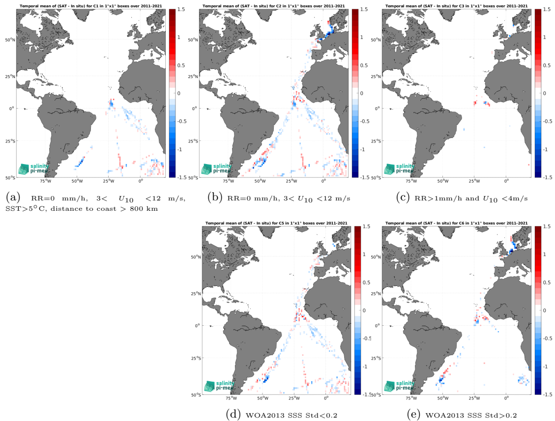
Figure 12: Temporal mean gridded over spatial boxes of size 1^\circ \times 1^\circ of \Delta SSS (SMOS SSS L4 v2 - Daily (BEC) - TSG (Polarstern)) for 5 different subdatasets corresponding to:RR=0 mm/h, 3 < U_{10} < 12 m/s, SST >5^\circ\text{C} , distance to coast > 800 km (a), RR=0 mm/h, 3 < U_{10} < 12 m/s (b), RR >1 mm/h and U_{10} < 4 m/s (c), WOA2013 SSS Std <0.2 (d), WOA2013 SSS Std >0.2 (e).
