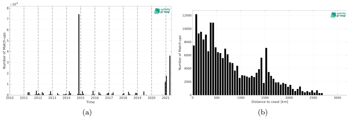
Figure 1: Number of match-ups between TSG (Polarstern) and SMOS SSS L4 v2 - Daily (BEC) SSS as a function of time (a) and as function of the distance to coast (b) over the Atlantic Ocean Pi-MEP region and for the full satellite product period.
