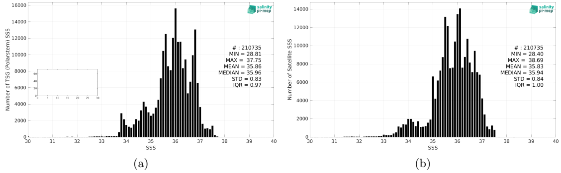
Figure 2: Histograms of SSS from TSG (Polarstern) (a) and SMOS SSS L4 v2 - Daily (BEC) (b) considering all match-up pairs per bins of 0.1 over the Atlantic Ocean Pi-MEP region and for the full satellite product period.
