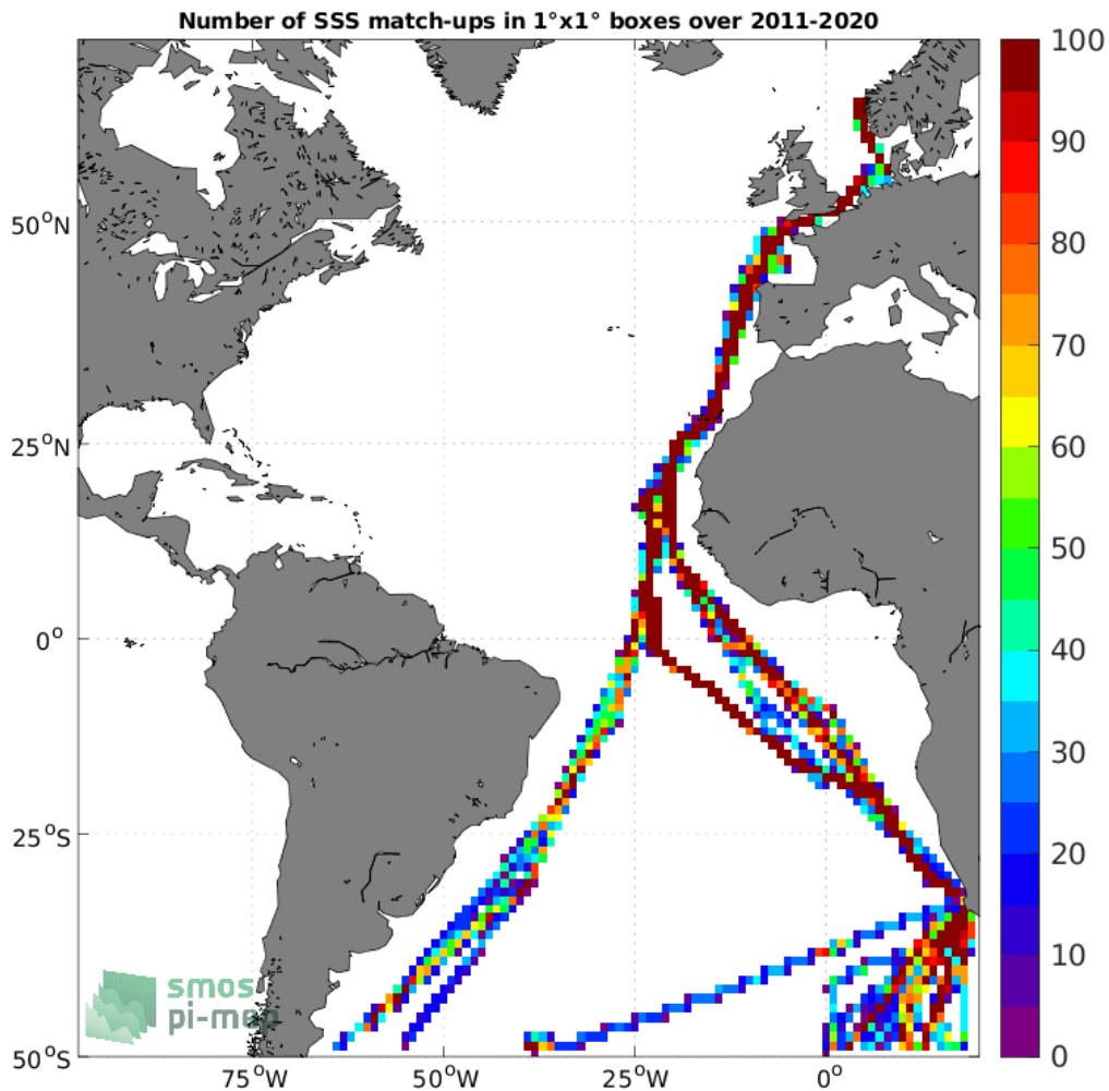
Figure 4: Number of SSS match-ups between TSG (Polarstern) SSS and the SMOS SSS L4 v2 - Daily (BEC) SSS product for the Atlantic Ocean Pi-MEP region over 1°×1° boxes and for the full satellite product period.
