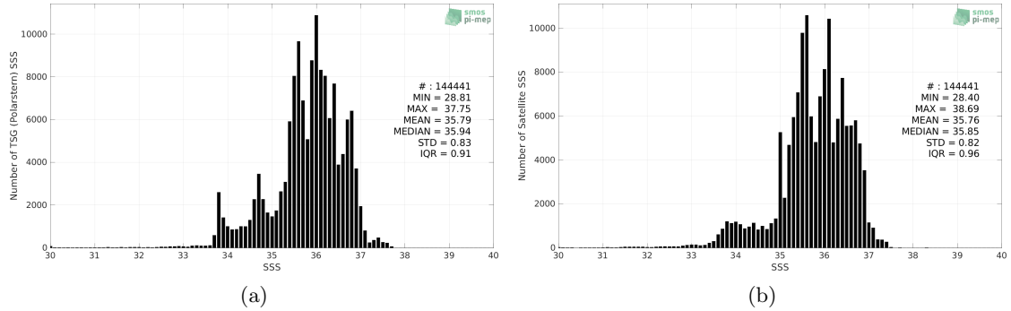
Figure 2: Histograms of SSS from TSG (Polarstern) (a) and SMOS SSS L4 v2 - Daily (BEC) (b) considering all match-up pairs per bins of 0.1 over the Atlantic Ocean Pi-MEP region and for the full satellite product period.
